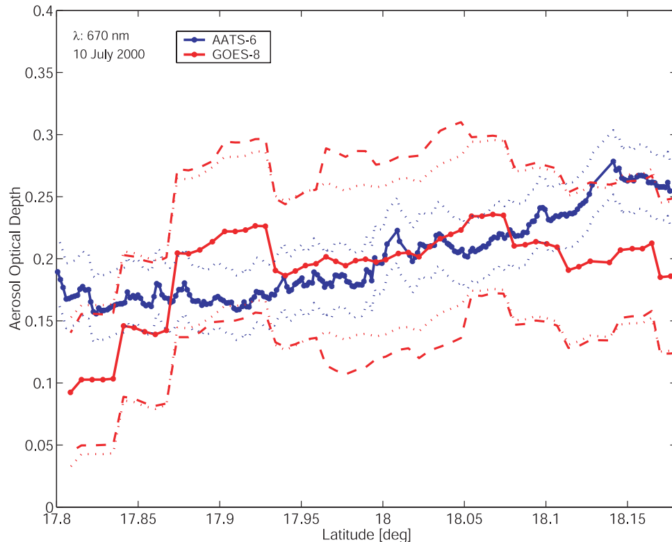
Figure 16. Observation of an AOD latitudinal gradient measured by AATS-6 (interpolated to 670 nm wavelength) and retrieved from GOES 8 measurements on 10 July. Dashed red lines represent a GOES 8 uncertainty of \pm 0.06 ; dotted red lines show sample standard deviations (see text for discussion). Dotted blue lines display the AATS-6 measurement uncertainties.
