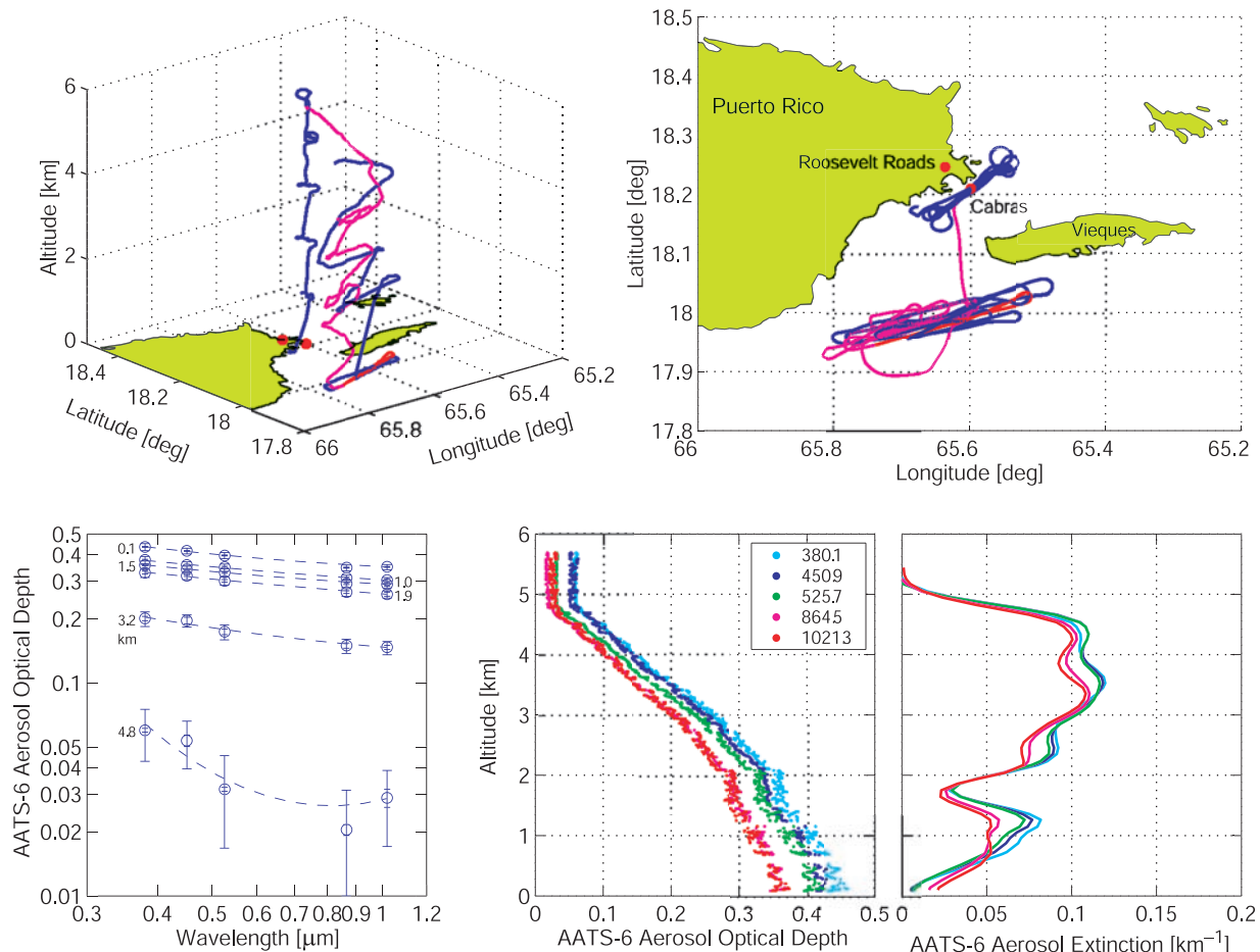
Figure 1. Navajo flight profile and AATS-6 measurements for 21 July 2000. Bottom three frames show measured aerosol optical depth spectra with second-order polynomial fits at various altitudes and vertical profiles of measured aerosol optical depth and derived aerosol extinction.
