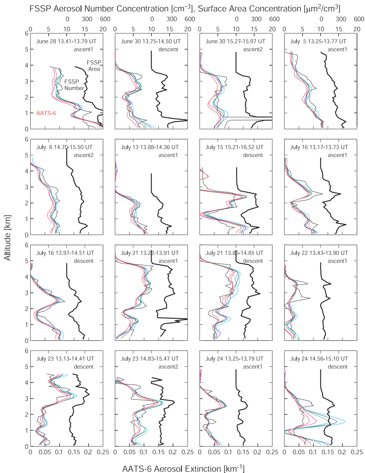
Figure 3. Vertical profiles of aerosol extinction (color lines) calculated from the aerosol optical depth profiles shown in Figure 2; overlays of coincident aircraft-mounted FSSP measurements of aerosol number (thin black line, 0–20 scale) and surface area (thick black line, 0–600 scale) concentration.
