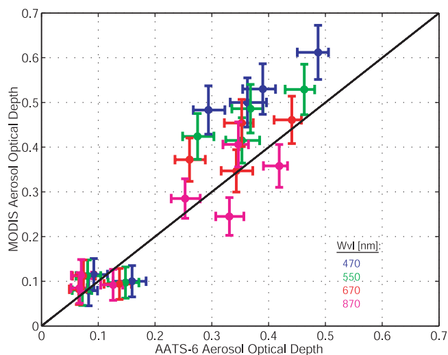
Figure 13. For the data shown in Figure 12, scatterplot of MODIS aerosol optical depth retrievals and coincident AATS-6 aerosol optical depth measurements interpolated to the MODIS wavelengths using the fits shown in Figure 12. Bars show measurement uncertainties.
