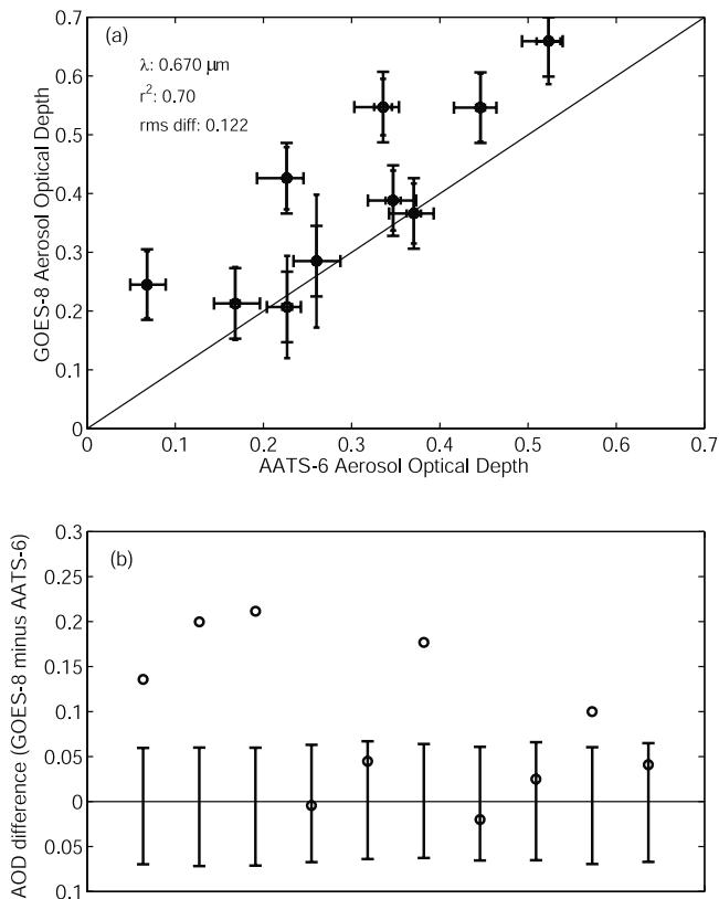
Figure 15. Comparison of GOES 8 AOD retrievals in the GOES visible channel and AATS-6 measurements taken within 100 m of the ocean surface at the time of satellite observation and interpolated to 670 nm wavelength: (a) AOD values, measurement uncertainties, and spatiotemporal sample standard deviations and (b) AOD differences (GOES 8 minus AATS-6) and combined measurement uncertainties.
