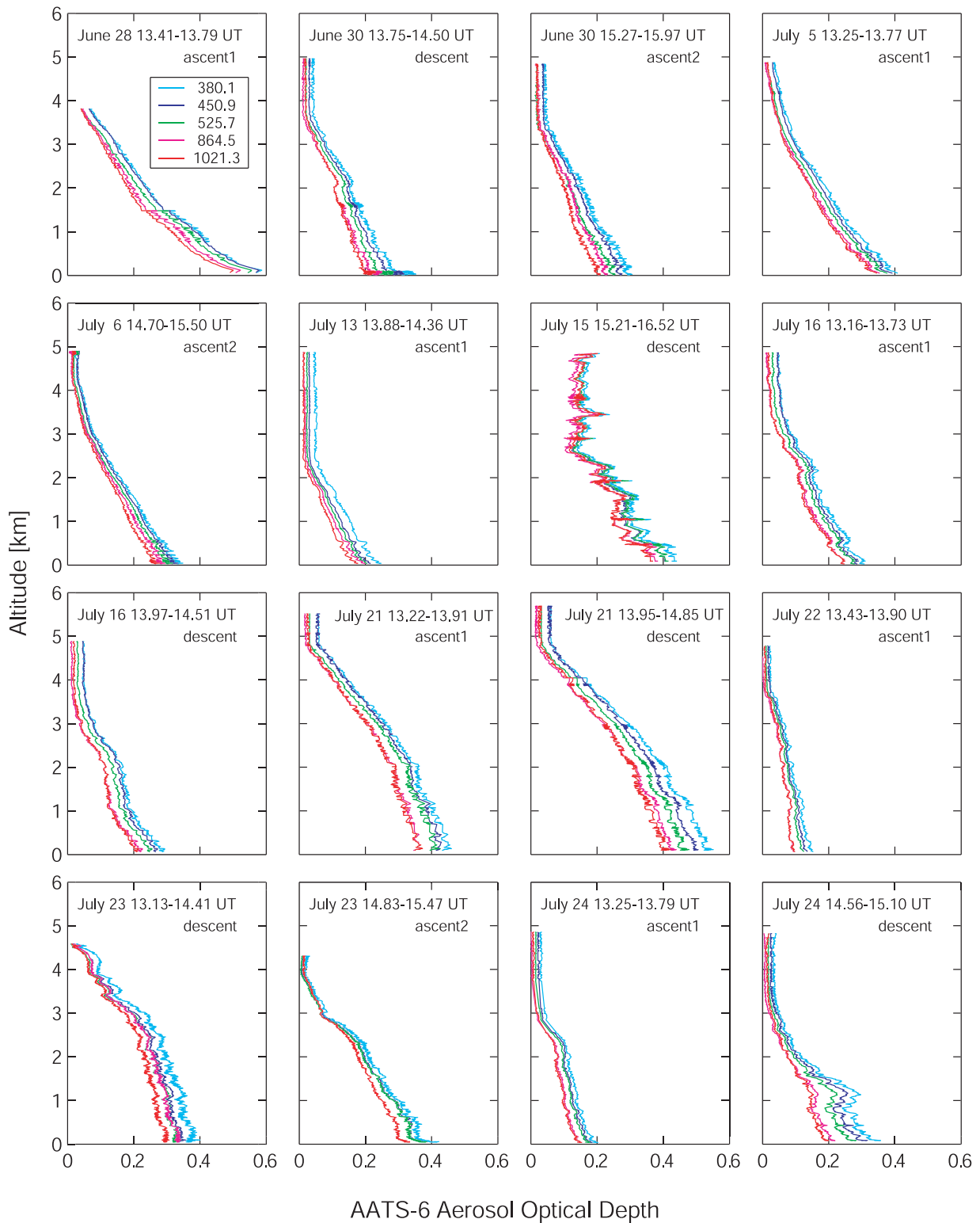
Figure 2. Vertical profiles of aerosol optical depth measured by AATS-6 during Navajo ascents and descents.
