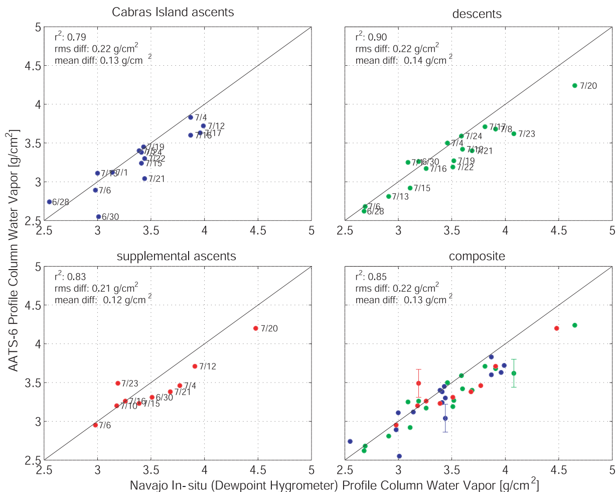
Figure 7. Comparison of columnar water vapor measured by AATS-6 and EdgeTech hygrometer during aircraft ascents and descents.
