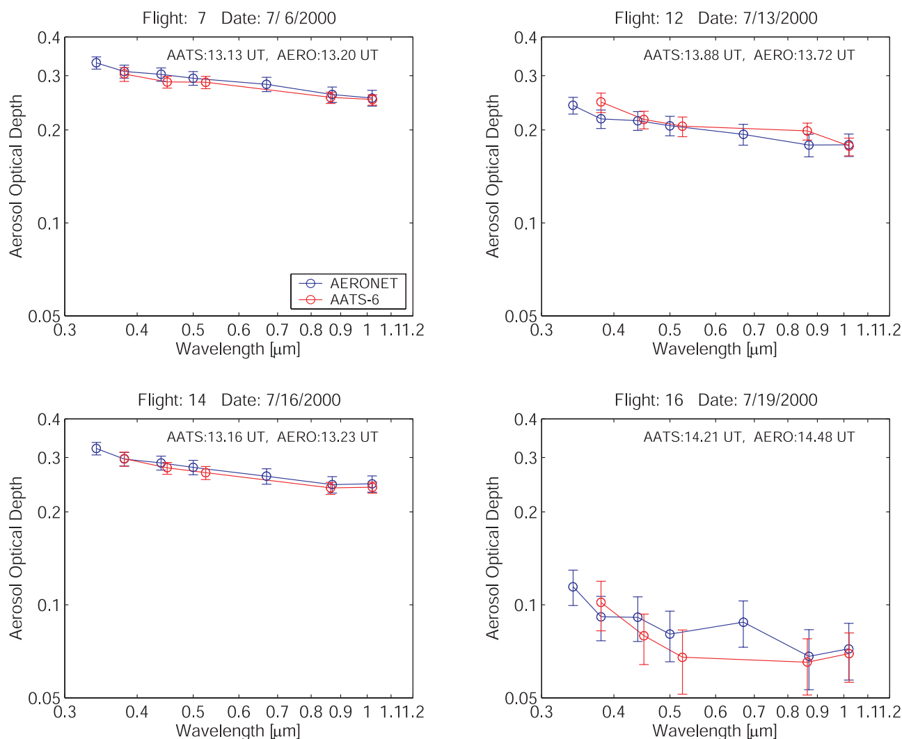
Figure 8. Comparison of aerosol optical depth spectra measured by AATS-6 and ground-based AERONET CIMEL during Navajo overflights of Cabras Island aerosol/radiation ground site.
