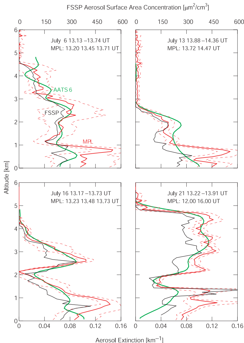
Figure 5. Comparison of aerosol extinction calculated from AATS-6 measurements (green line) at 525.7 nm during ascents over the Cabras Island aerosol/radiation ground site and corresponding extinction (solid red line) calculated from coincident backscatter measurements by the GSFC micropulse lidar located at the Cabras site; overlay of coincident total aerosol surface area concentration (solid black line) measured by the FSSP aboard the Navajo. Dashed red lines are mean measurement uncertainties in the MPL profiles.
