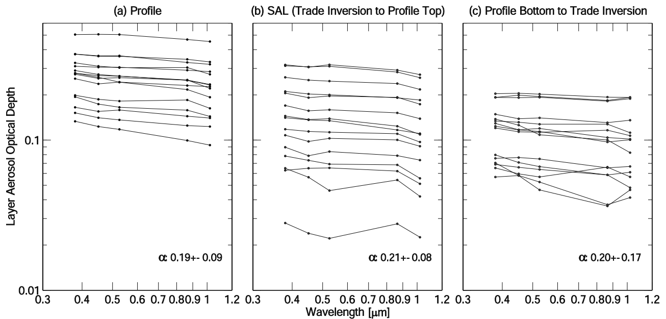
Figure 4. Aerosol optical depth layer spectra measured (a) for the entire profile sampled by the Navajo, (b) for the Saharan Air Layer, and (c) for the layer from the bottom of the profile to the top of the trade inversion.
