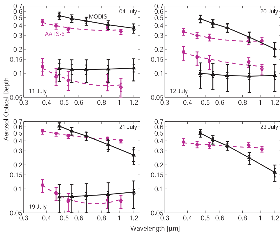
Figure 12. Aerosol optical depth spectra measured by AATS-6 during aircraft horizontal flight legs at altitudes 30–100 m above the ocean surface and corresponding spectra retrieved from coincident MODIS measurements. Dashed lines are quadratic fits to AATS-6 AOD spectra in log-log space. Solid lines merely connect the MODIS data points. Vertical bars with wide ticks are expected (MODIS) or calculated (AATS-6) measurement uncertainties; bars with narrow ticks are the spatiotemporal sample standard deviations.
