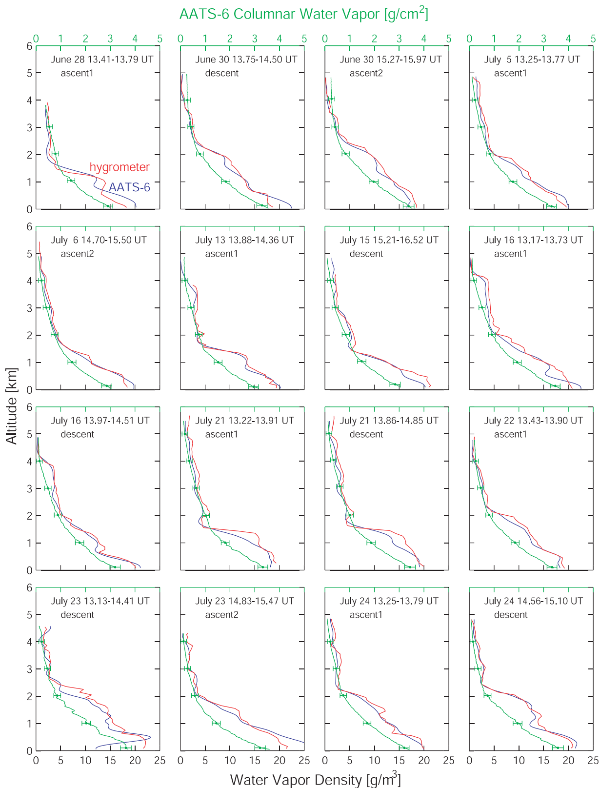
Figure 6. Vertical profiles of columnar water vapor (green line) and water vapor density (blue line) measured by AATS-6 for the same flights shown in Figures 2 and 3; corresponding profiles of water vapor density (red line) calculated from the aircraft in situ measurements of pressure, temperature, and dewpoint (EdgeTech hygrometer).
