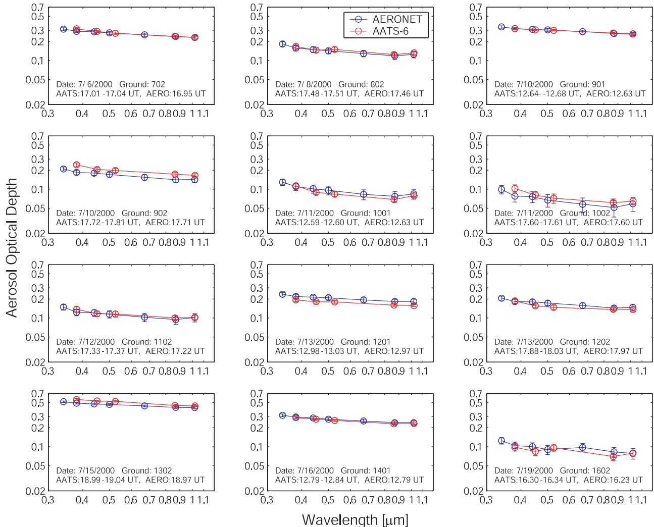
Figure 10. Comparison of ground-based measurements of aerosol optical depth spectra from the AERONET CIMEL at Cabras Island and the AATS-6 at Roosevelt Roads NAS.
