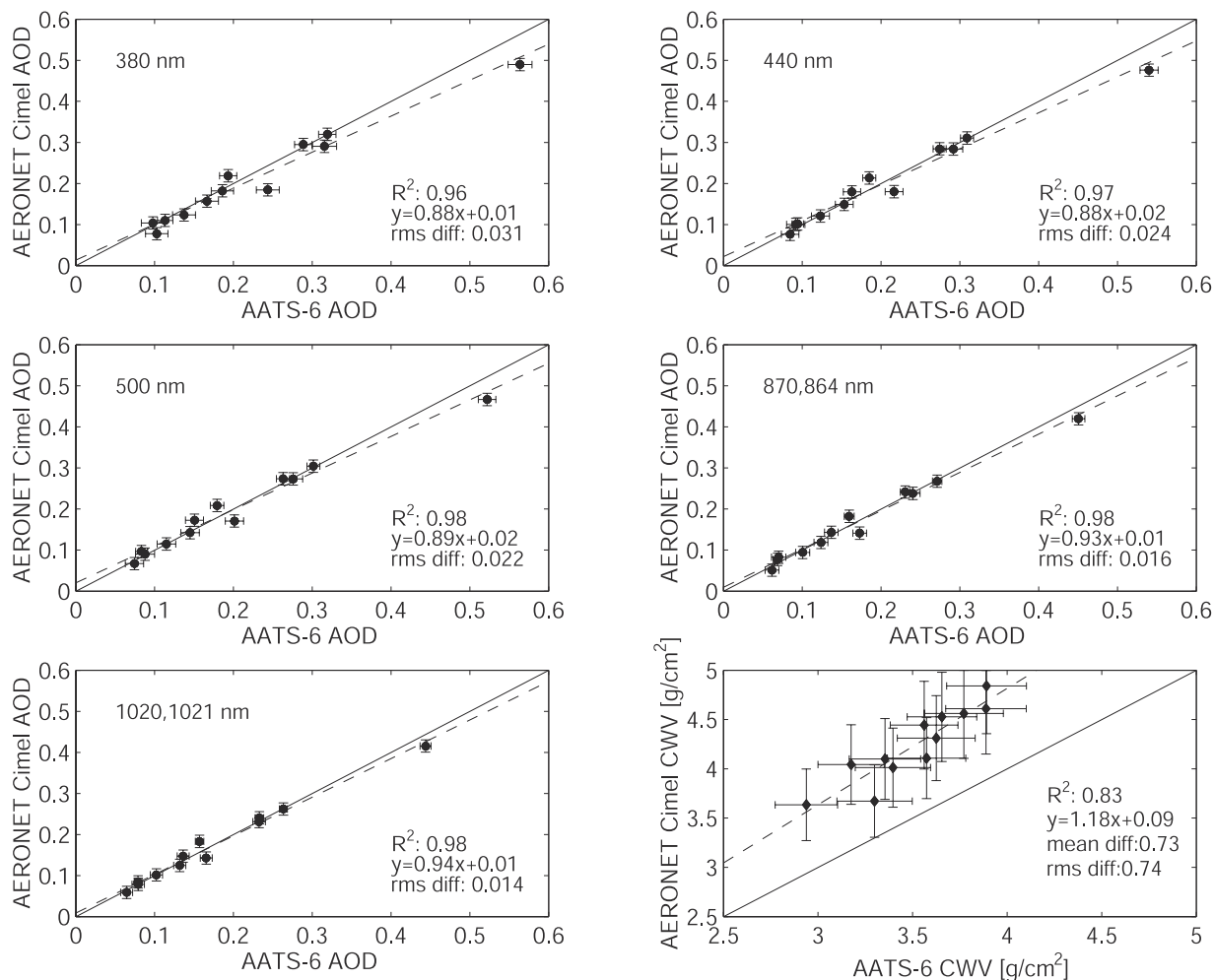
Figure 11. Scatterplots of aerosol optical depth and columnar water vapor measured by AATS-6 and ground-based AERONET CIMEL for the cases shown in Figure 10.
