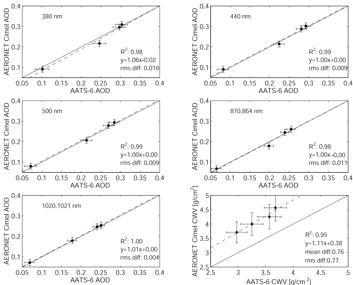
Figure 9. Scatterplots of aerosol optical depth and columnar water vapor measured by AATS-6 and ground-based AERONET CIMEL for the cases shown in Figure 8.
