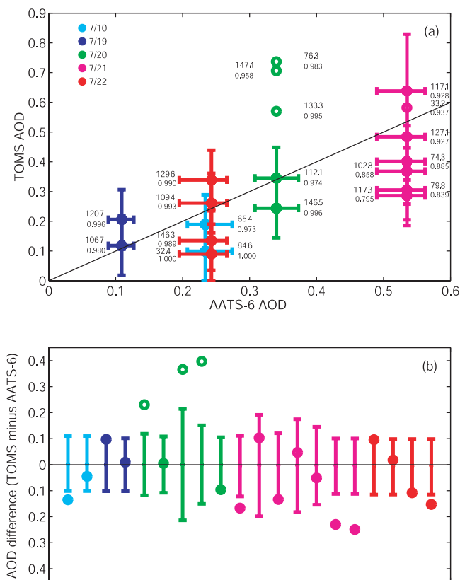
Figure 14. Comparison of 380-nm wavelength aerosol optical depth measured by AATS-6 during aircraft horizontal flight legs at altitudes 30–100 m above the ocean surface, and corresponding 380-nm aerosol optical depth retrieved from TOMS ultraviolet backscatter measurements taken within 150 km and one hour of the AATS-6 data: (a) AOD values and uncertainties and (b) AOD differences (TOMS minus AATS-6) and combined measurement uncertainties.
