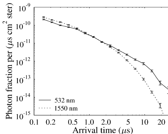
FIG. 15. Simulated in situ lidar time series for upward-pointing detectors at y = 2.8 \text{ km} in field StCu21 for lidars operating at 532- and 1550-nm wavelengths.
