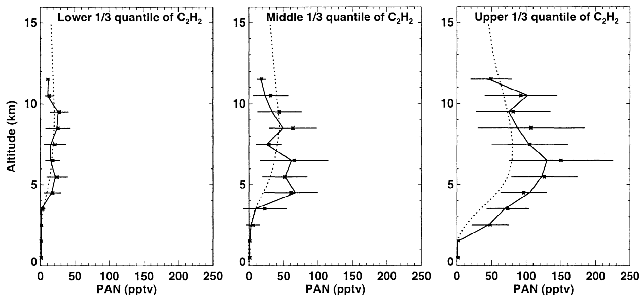
Figure 12. Same as Figure 3 but for peroxyacetylnitrate (PAN). Simulated PAN concentrations are from the standard model.
