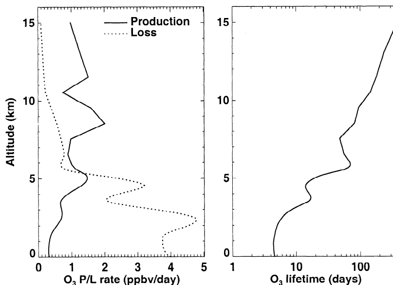
Figure 9. Simulated O_3 production and loss rate and its chemical lifetime as a function of altitude for the middle one-third quantile of C_2H_2 .
