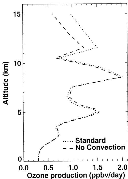
Figure 8. Same as Figure 7 but for the \text{O}_3 production rate.
