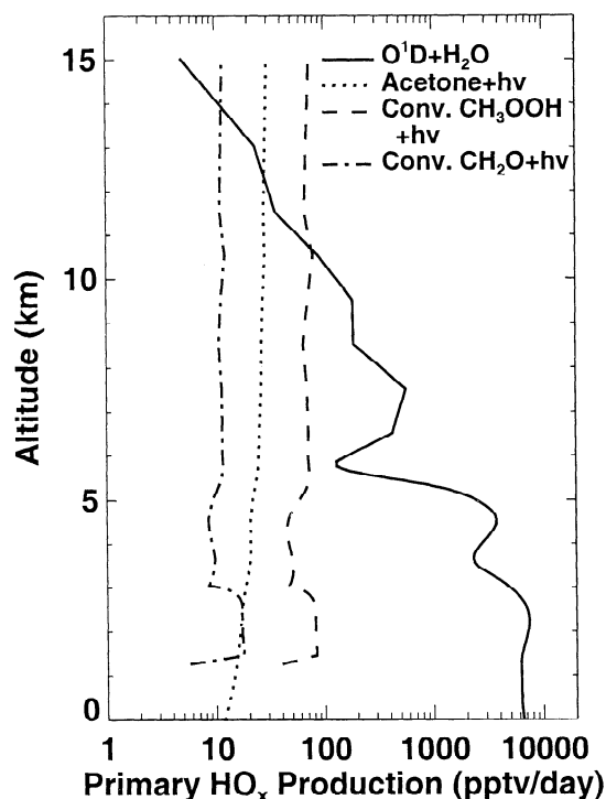
Figure 6. Simulated primary sources of \text{HO}_x , \text{O}^1\text{D}+\text{H}_2\text{O} , photolysis of acetone, and photolysis of \text{CH}_3\text{OOH} and \text{CH}_2\text{O} transported from the lower troposphere by convection, as a function of altitude for the middle one-third quantile of \text{C}_2\text{H}_2 . The \text{HO}_x yield of \text{CH}_2\text{O} photolysis is computed on line.
