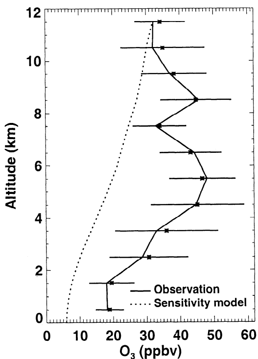
Figure 10. Comparison of observed and simulated vertical profiles O_3 for the middle one-third quantile of C_2H_2 . Symbols are the same as in Figure 1. The concentration of O_3 at 11–12 km is specified as observed in the sensitivity simulation.
