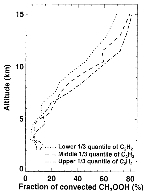
Figure 5. Fraction of \text{CH}_3\text{OOH} attributed to convective transport as a function of altitude for the lower, middle, and upper one-third quantiles of \text{C}_2\text{H}_2 .
