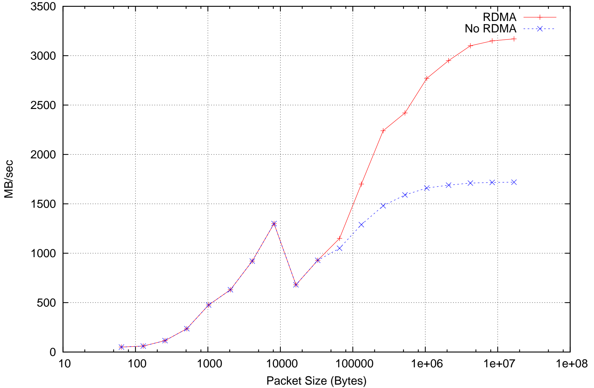
Bassi (HPS) PP Send/Receive BW (One-Way)
