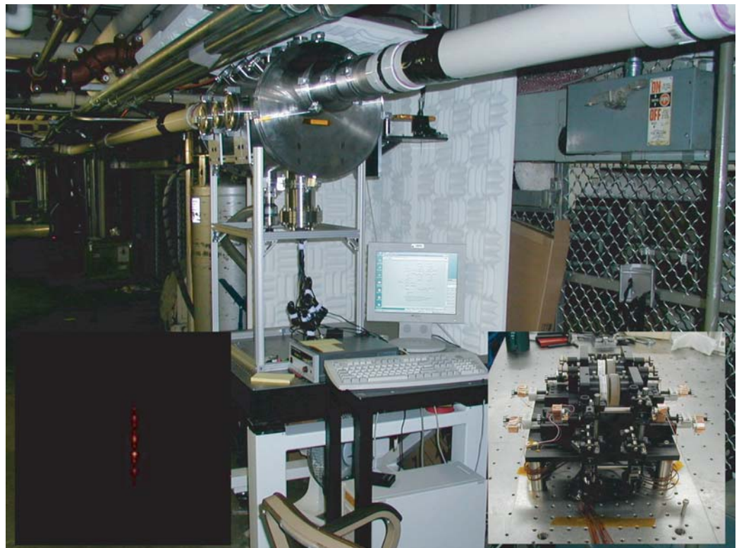
The Black Hole Imager makes use of X-ray interference (lower left), recently demonstrated in the laboratory.
