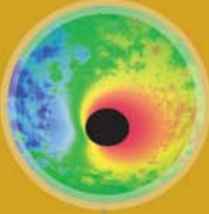
black holes
