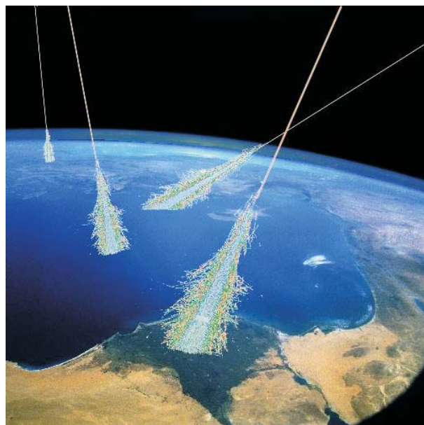
Simulations of particle showers produced by 10^{20} eV cosmic rays in the Earth's atmosphere.
