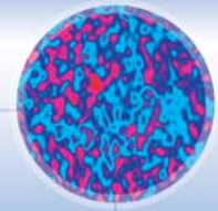
big bang
