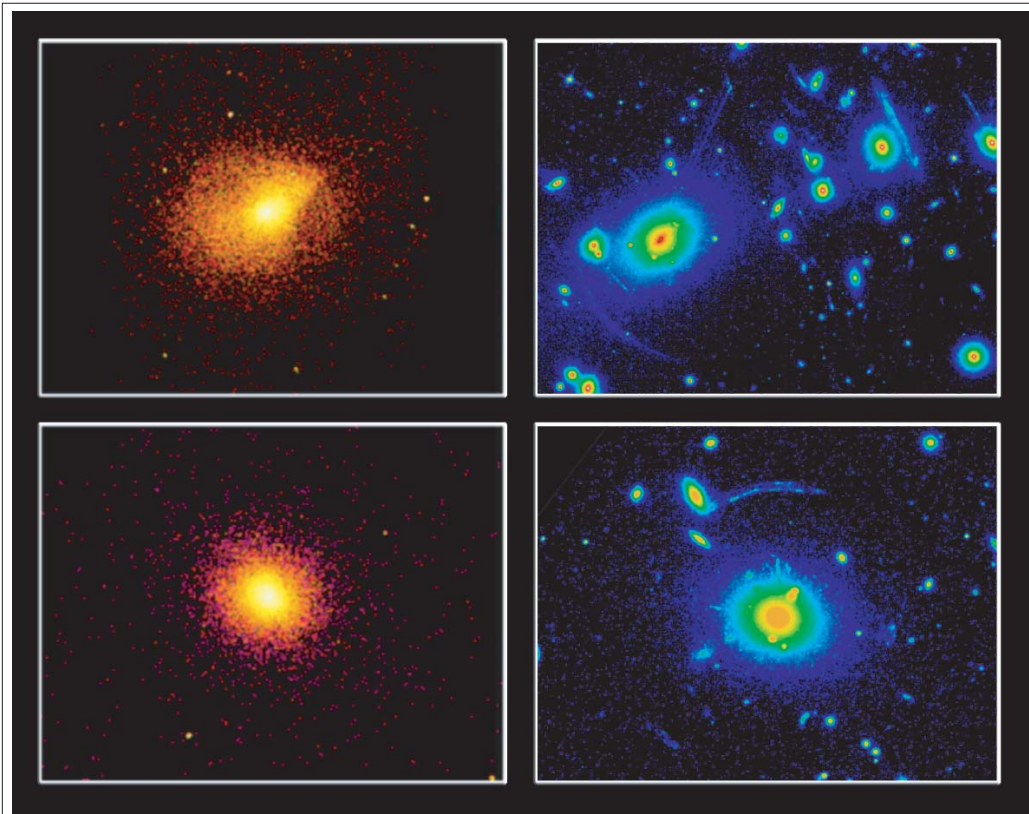
Observations of distant clusters of galaxies also provide independent evidence for dark energy. This montage shows two sets of Chandra X-ray Observatory images (left) and Hubble Space Telescope images (right) of two giant galaxy clusters. Most of the mass is in the form of dark matter. The X ray emission comes from the multimillion-degree gas that fills the clusters. Chandra provides detailed temperature maps for this gas to precisely determine the masses of the clusters. The gravity of the dark matter acts as a large cosmic lens on the light from distant background galaxies to produce the giant arcs seen in the images. The Hubble Space Telescope data place independent constraints on the masses of the clusters that confirm the Chandra results.
