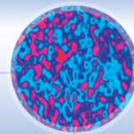
big bang
