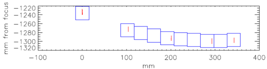
Raytrace determination of CCD position at the focal plane. Blue boxes are 30 mm x 30 mm CCDs (one for zero order camera), red lines are zero order, 12 Å, 24 Å, 36 Å, and 41 Å
