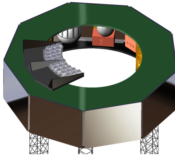
Grating Mirror Assembly Platform mounted to S/C Platform 13.5 m from telescope focus
