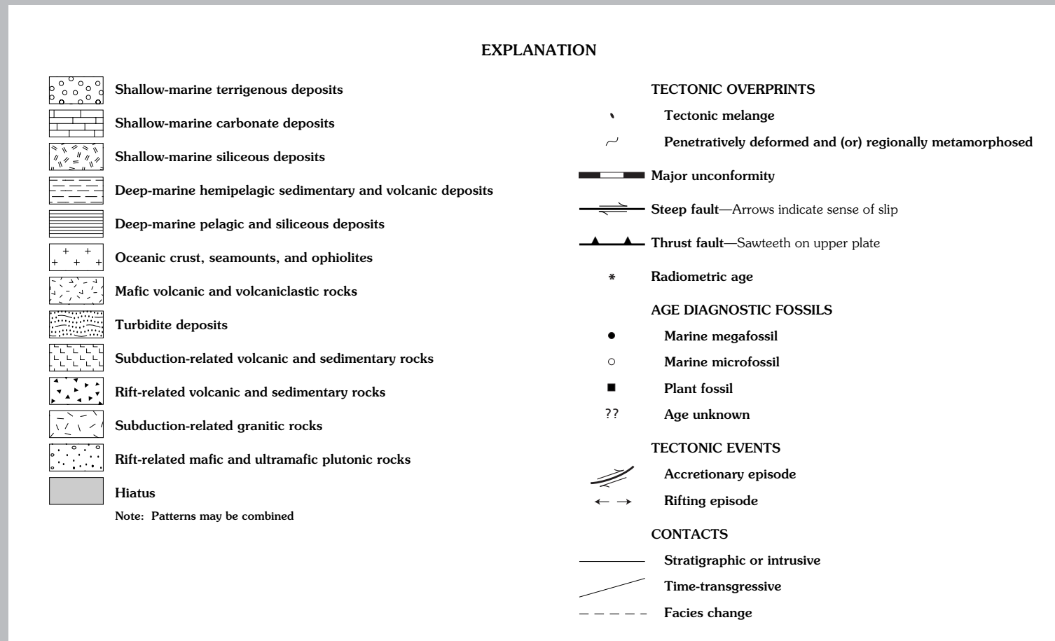
Figure 14 (below and pages 24–25). Geologic characteristics of lithotectonic terranes in the Wrangell–Saint Elias region. ( Modified from Nokleberg and others, 1994, and Plafker, Moore, and Winkler, 1994. )
