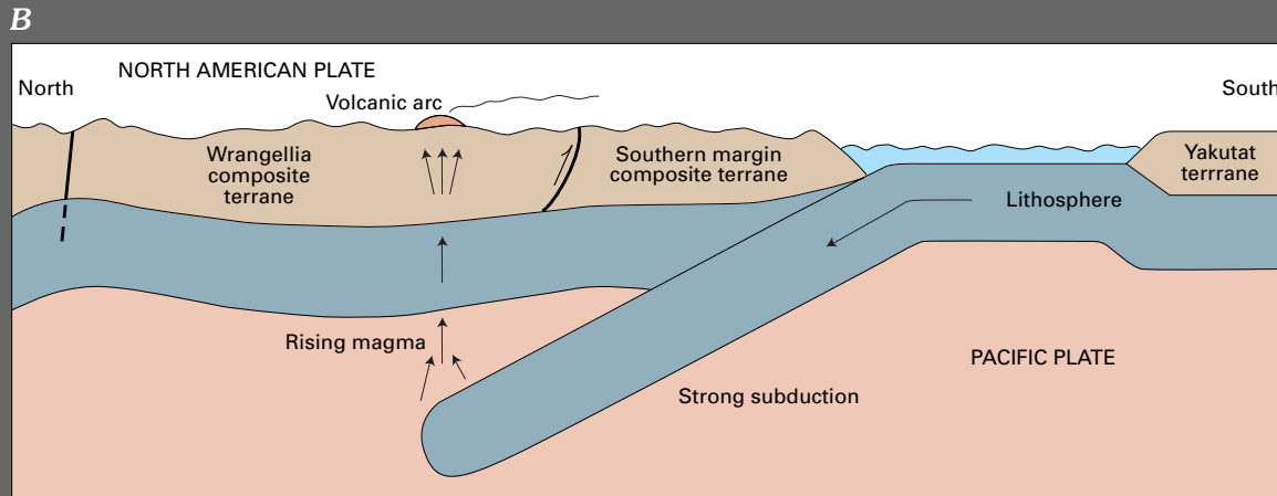
Figure 10. Diagrammatic cross sections through the Earth's crust and upper mantle, showing plate-tectonic features developed in ocean basins and at continental margins. A , General features and nomenclature. B , The Wrangell–Saint Elias region and the northern Pacific Ocean, about 26 m.y. ago, showing collision of oceanic and continental plates, the Pacific and North American plates, with strong subduction causing formation of an active volcanic arc. C , The Wrangell–Saint Elias region and the northern Pacific Ocean at the present time, showing that collision of continental plates, the Yakutat terrane and the North American plate, has jammed the subduction zone and quieted the volcanism. (Modified from Richter, Rosenkrans, and Steigerwald, 1995.)
