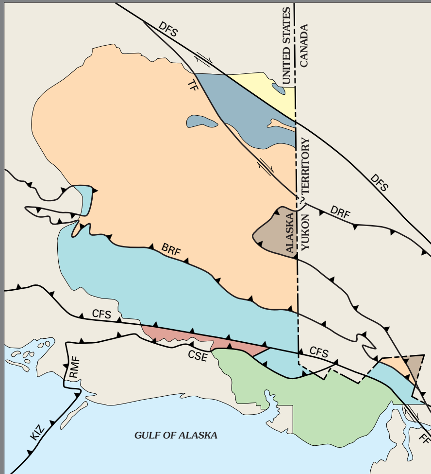
Figure 12 . Map showing lithotectonic terranes and major faults of Wrangell-Saint Elias National Park and Preserve.
