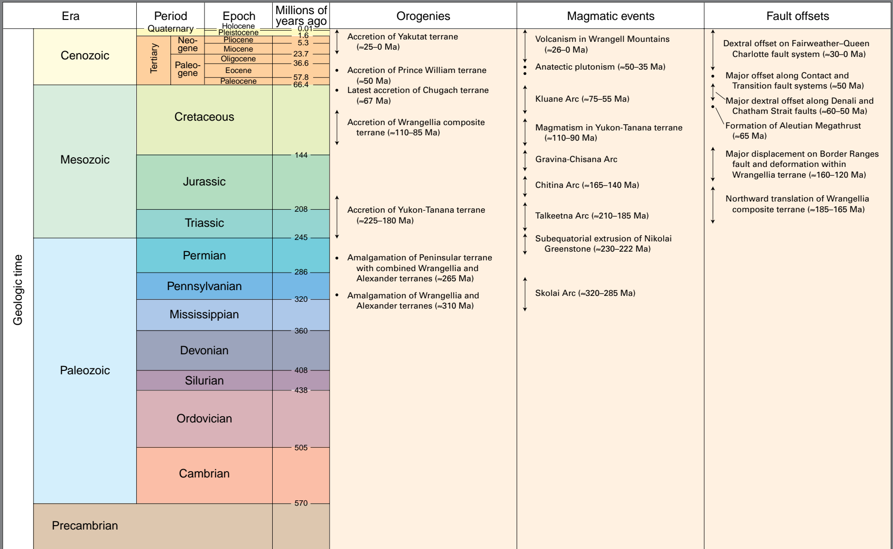
Figure 11. Geologic time scale, showing timing of major geologic events in the Wrangell–Saint Elias region. (Time subdivisions and dates are from the Decade of North American Geology 1983 geologic time scale.)
