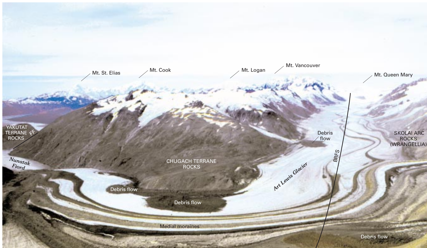
Figure 23. The Border Ranges fault system (BRFS) underlies the trough of Art Lewis Glacier, on the right; Nunatak Fiord is on the left; view is to the northwest from near the extreme southeast corner of Wrangell–Saint Elias National Park and Preserve. Here, the Border Ranges fault separates upper Paleozoic rocks of the Skolai arc (the Wrangellia terrane) on the right from metamorphosed sedimentary and volcanic rocks of the Mesozoic Chugach terrane on the left. The Fairweather fault (FF) is located at the base of the mountain front near the left edge. The Fairweather fault currently acts as the boundary between the North American and Pacific crustal plates. The high peaks in the background are, from left to right, Mt. St. Elias (18,008 ft), Mt. Cook (13,760 ft), Mt. Logan (in Canada, 19,850 ft), Mt. Vancouver (15,700 ft), and Mt. Queen Mary (in Canada, 12,800 ft). Note the strongly curving moraines near the right edge of Art Lewis Glacier, deformed by surges in tributary glaciers entering the valley glacier from the east. Note also several patches of brown-colored debris on the surface of Art Lewis Glacier near its edges. These may have formed as earthquake-induced debris flows (landslides) along the oversteepened margins of the glacier, but have now moved downglacier from their sources. If their age of formation were known, approximate rates of glacier movement could be determined. (M.D. Wilson)
