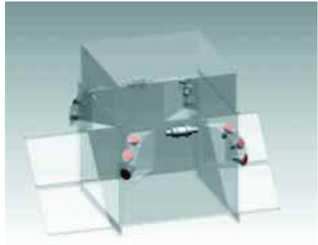
Figure 11-3 Schematic layout of the 12 NaI and two BGO detectors on the GLAST spacecraft. The actual mounting scheme will be defined when the spacecraft design is selected.
