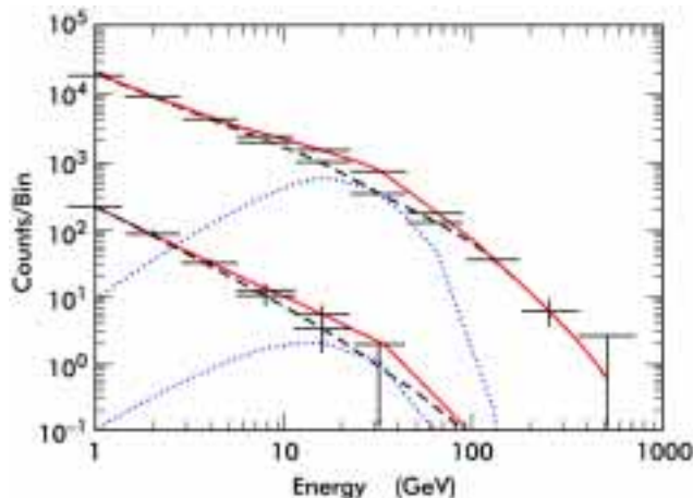
Figure 5-1 Simulated diffuse extragalactic gamma-ray flux measurements for GLAST (upper points) and EGRET (lower points). The dashed lines show the flux from unresolved AGNs, the dotted lines the contributions from WIMP decays in the early Universe, and the solid line shows the total (Willis 1996).
