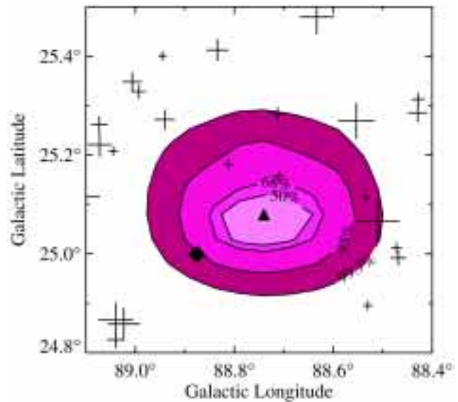
Figure 4-3 EGRET source location map for 3EG J1835+5918 (Hartman et al. 1999), an intense, apparently steady source with no X-ray or radio counterpart. The crosses are positions of radio continuum sources in the 1.4 GHz NRAO VLA Sky Survey (Condon et al. 1996). The sizes of the crosses are related to the fluxes; the faintest are only ~10 mJy. The diamond indicates the location of the X-ray source RX J1836.2+5925 proposed to be the neutron star responsible for the gamma-ray emission (Mirabal & Halpern 2001).
