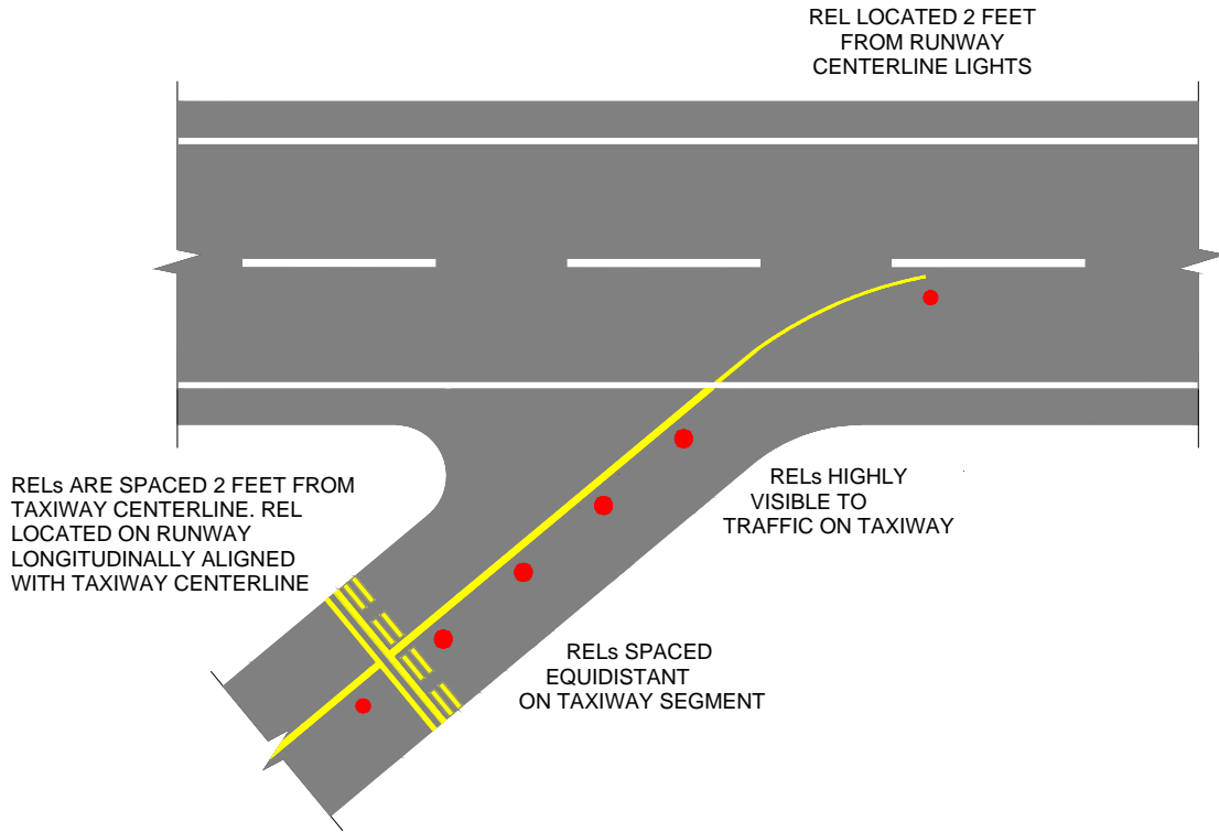
Figure 144. Angled Configuration
