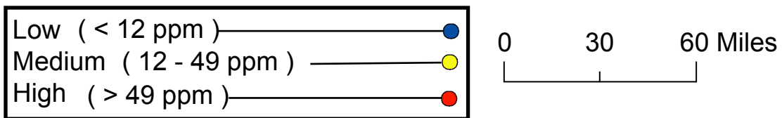
Figure PQ-14. Manganese concentration in the Wyodak-Anderson coal zone, Powder River Basin, Wyoming and Montana.
