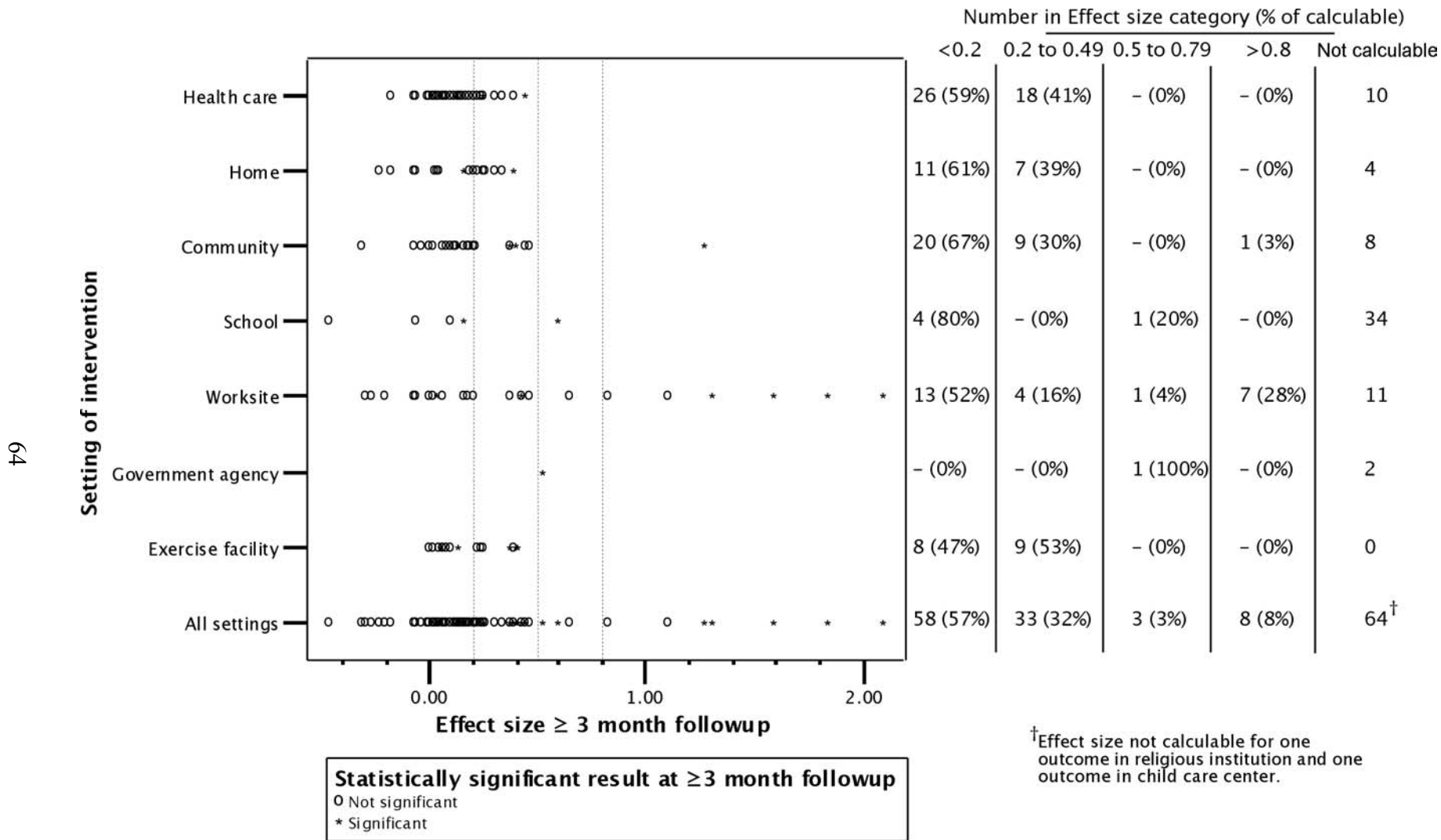
Figure 7. Effect size by intervention setting for all outcomes
