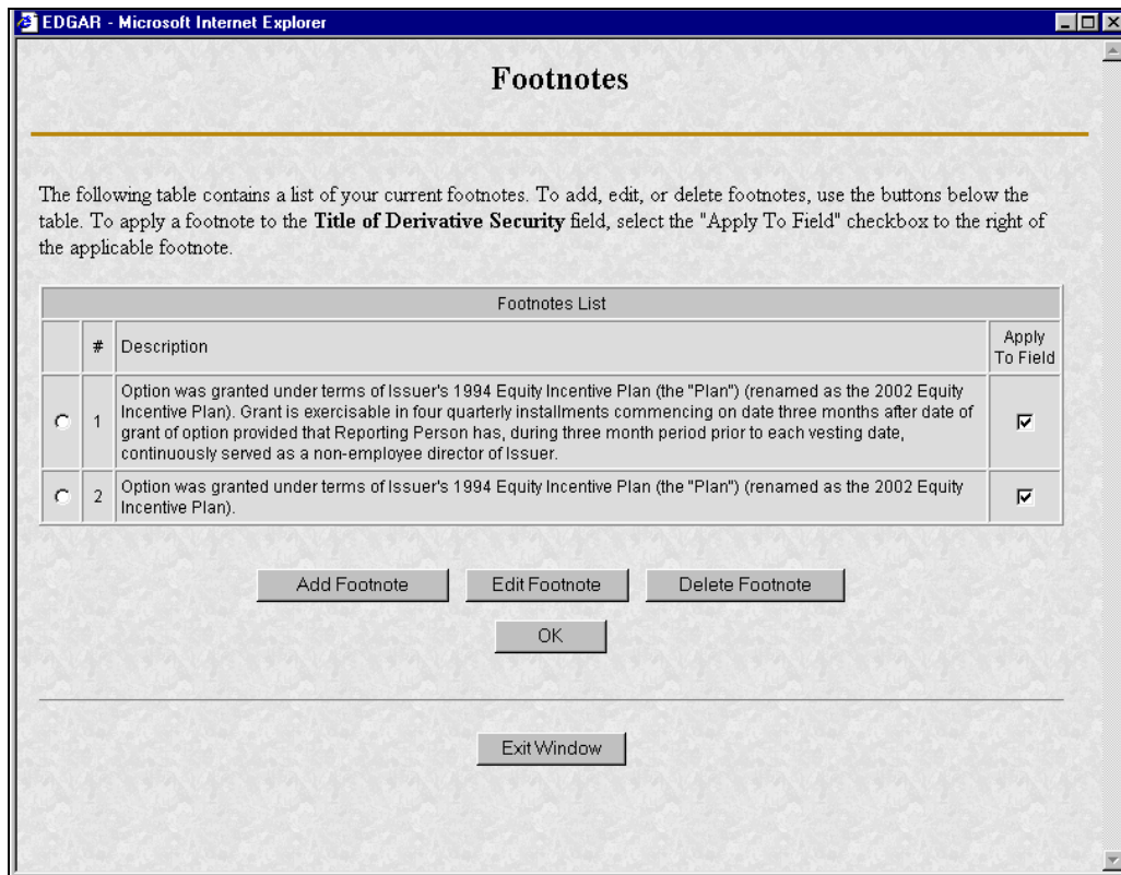
Figure 8-11: Footnotes Page
