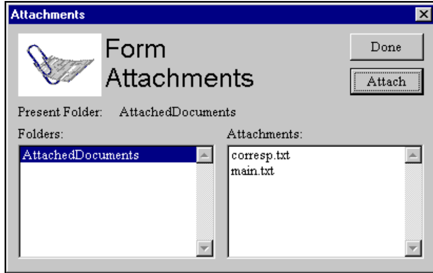
Figure 6-21: Attachments Window
