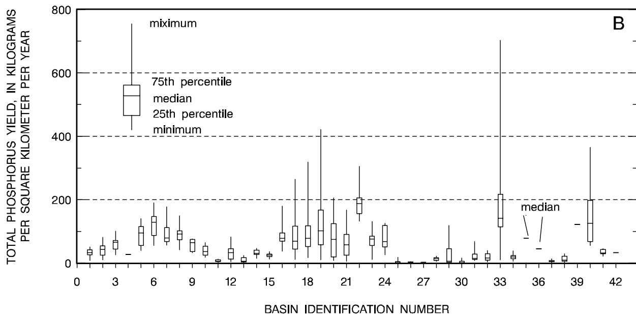
Figure 4.9 (A) Spatial distribution of total phosphorus yields in the 42 interior basins, and (B) box plots showing distribution of total phosphorus yields in the 42 interior basins. Dashes (-) show median yields for several sites where other statistics could not be calculated.
