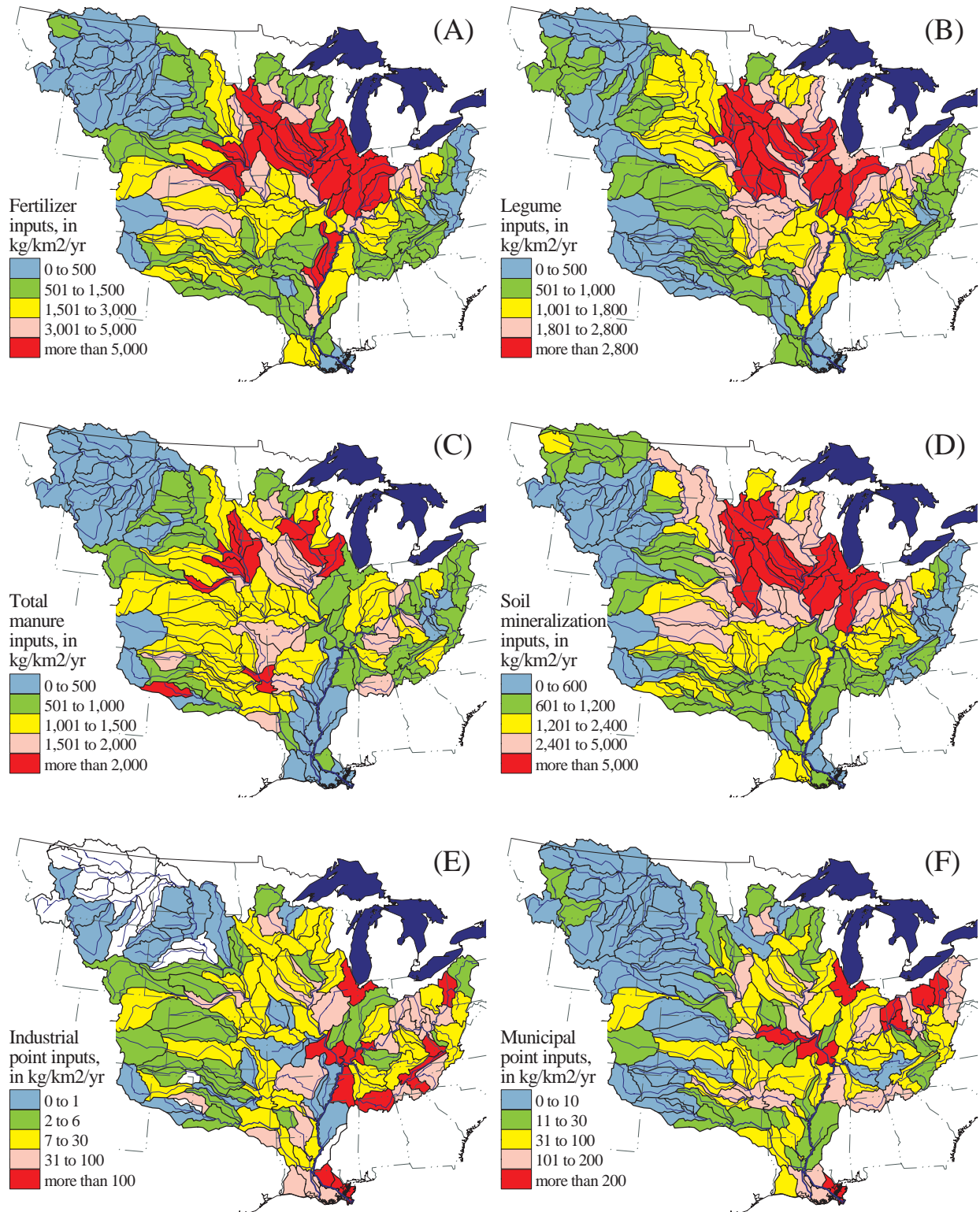
Figure 5.8 Nitrogen inputs in hydrologic accounting units in 1992 from (A) fertilizer, (B) legumes, (C) livestock manure (D) soil mineralization, (E) industrial point sources, and (F) municipal point sources.
