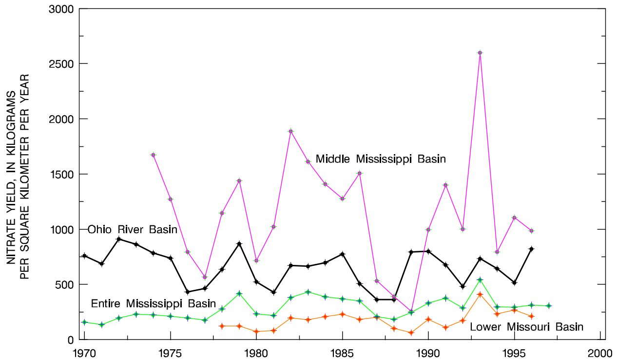
Figure 4.6 Temporal patterns in nitrate yields in the Middle Mississippi, Ohio, Lower Missouri, and entire Mississippi River basin, 1970-96 (see figure 2.1 for site locations).
