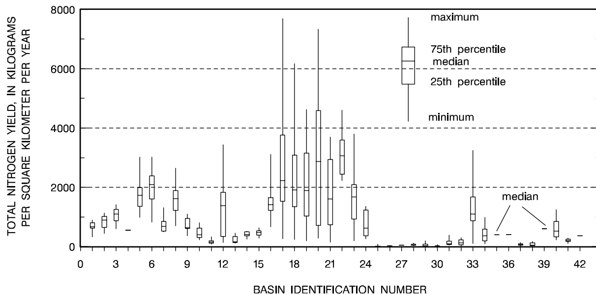
Figure 4.8 (A) Spatial distribution of total nitrogen yields in the 42 interior basins, and (B) box plots showing distribution of total nitrogen yields in the 42 interior basins. Dashed (-) show median yields for several sites where other statistics could not be calculated.
