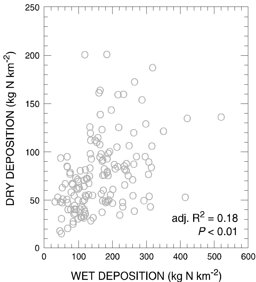
Figure 5.4 Dry deposition data from CASTNet (Clean Air Status and Trends Network, Clarke and others, 1997) as a function of wet deposition data from the National Atmospheric Deposition Program (NADP, http://nadp.sws.uiuc.edu/ ) at 14 sites in the Mississippi River basin where dry and wet deposition measurement stations are co-located. Values represent seasonal total (winter, December-February; spring, March-May; summer, June-August; fall, September-November) from January 1989-November 1994.
