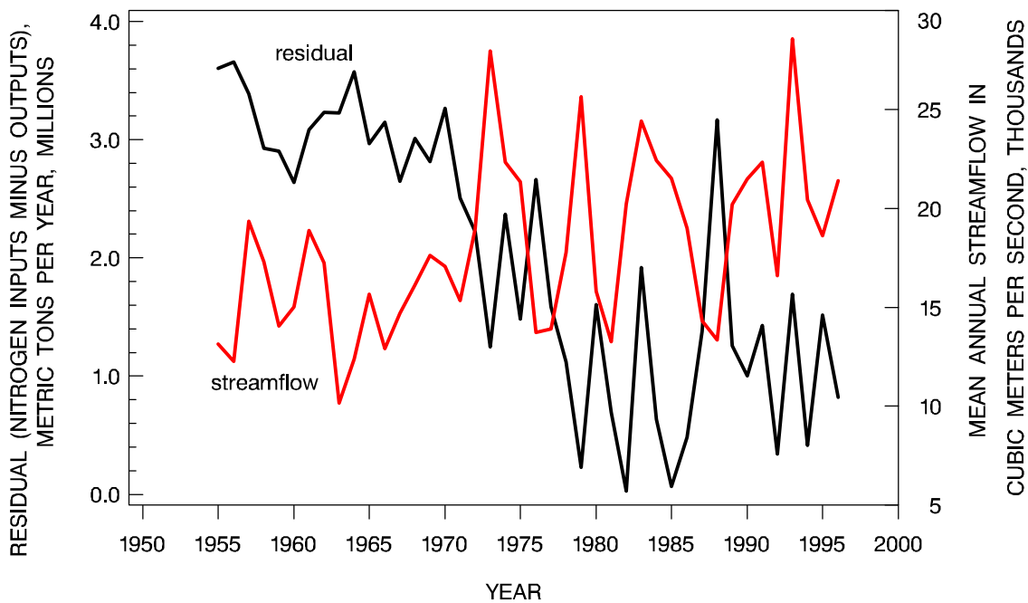
Figure 6.6 Graphs showing the relation between the annual nitrogen residual from mass balance and the average annual streamflow from the Mississippi-Atchafalaya River basin to the Gulf of Mexico.
