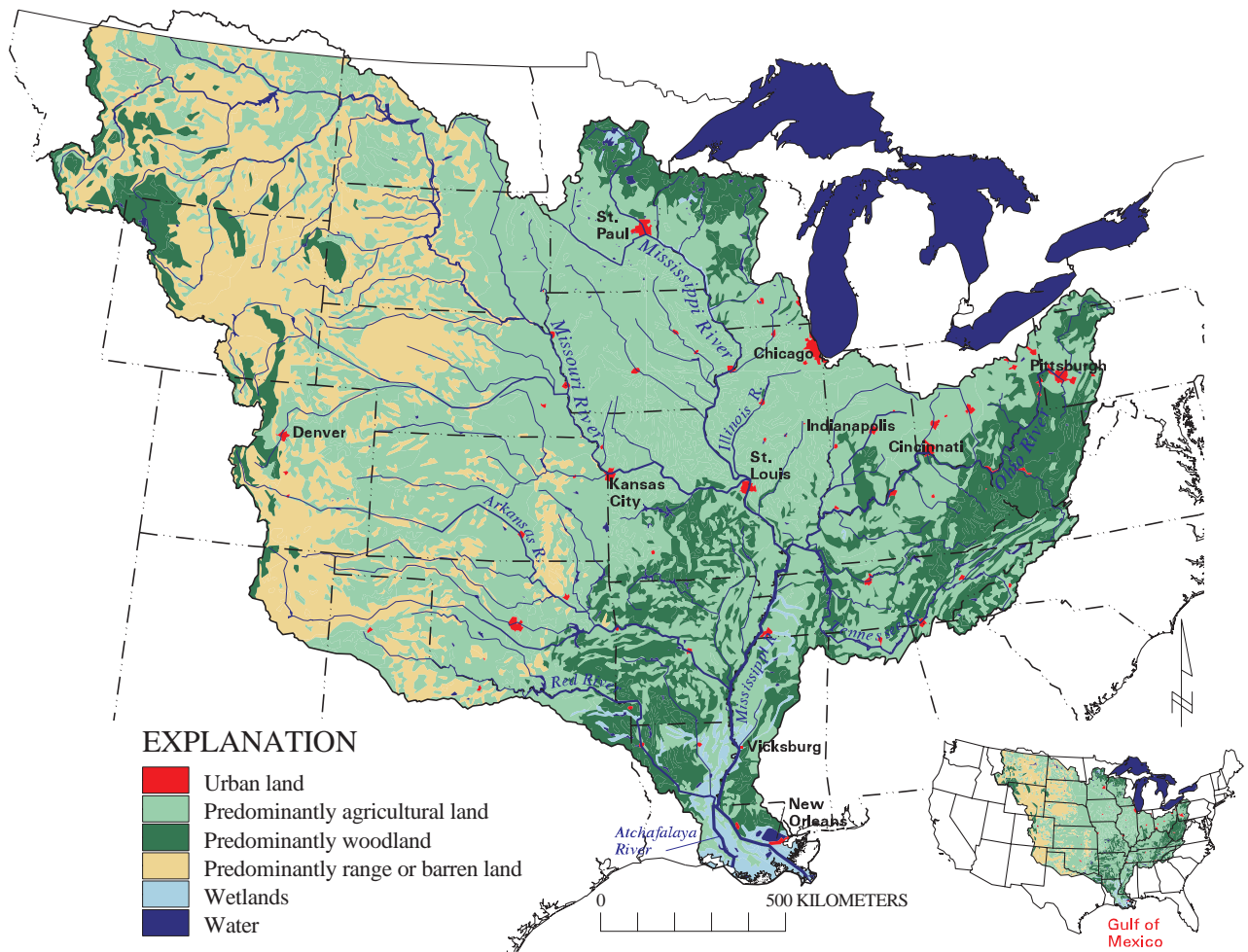
Figure 1.1 Location map showing drainage and land use in the Mississippi-Atchafalaya River basin.
