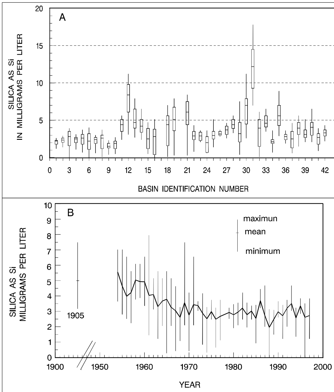
Figure 3.6 (A) Box plots showing distribution of silica concentrations in the 42 interior basins, and (B) long-term pattern in silica concentrations in the Mississippi River at St. Francisville, LA, 1955-96.
