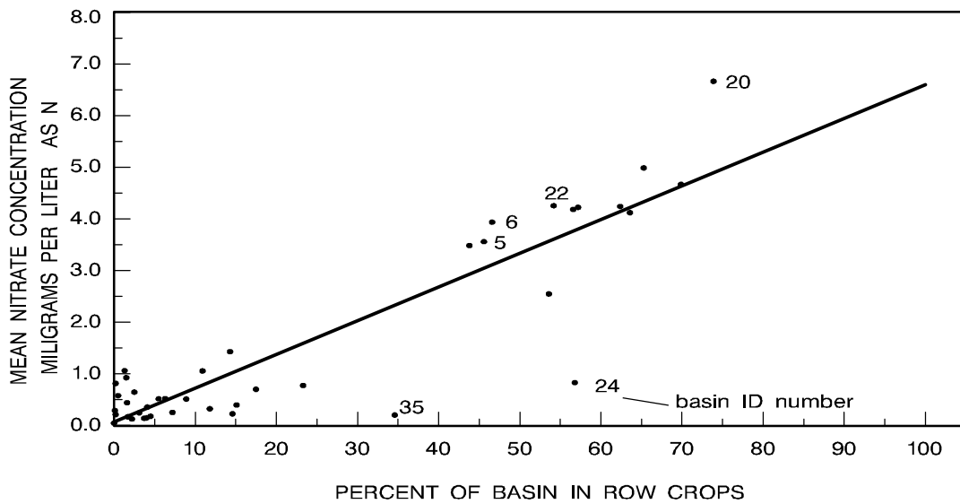
Figure 3.2 Relation between mean nitrate concentrations and percent of basin in row crops (data presented in tables 2.3 and 3.3).
