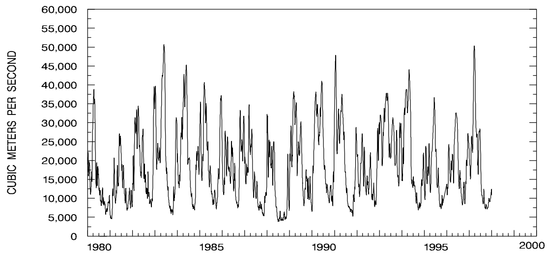
Figure 1.2 Daily mean streamflow for the Mississippi River at Vicksburg MS (source of data: U.S. Army Corps of Engineers, Vicksburg, MS).
