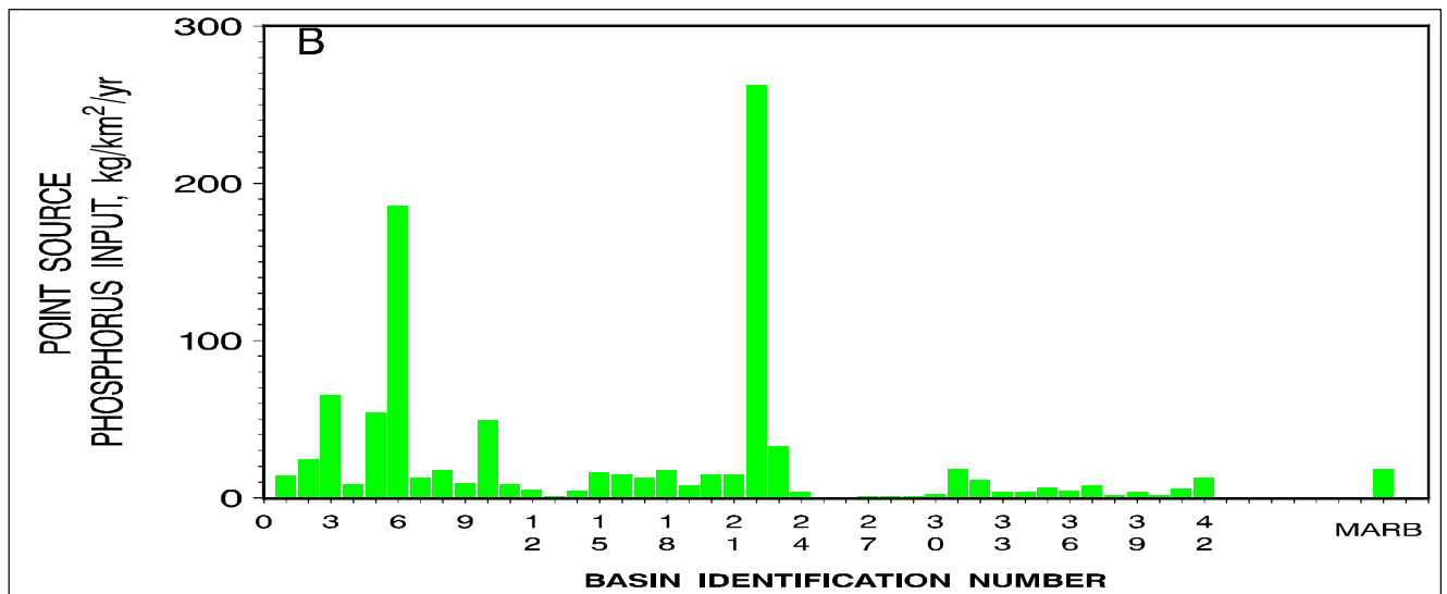
Figure 6.3 Bar graphs showing (A) yields of orthophosphate, suspended and total phosphorus and (B) phosphorus inputs from point sources in 42 interior basins and the entire Mississippi-Atchafalaya River basin.
