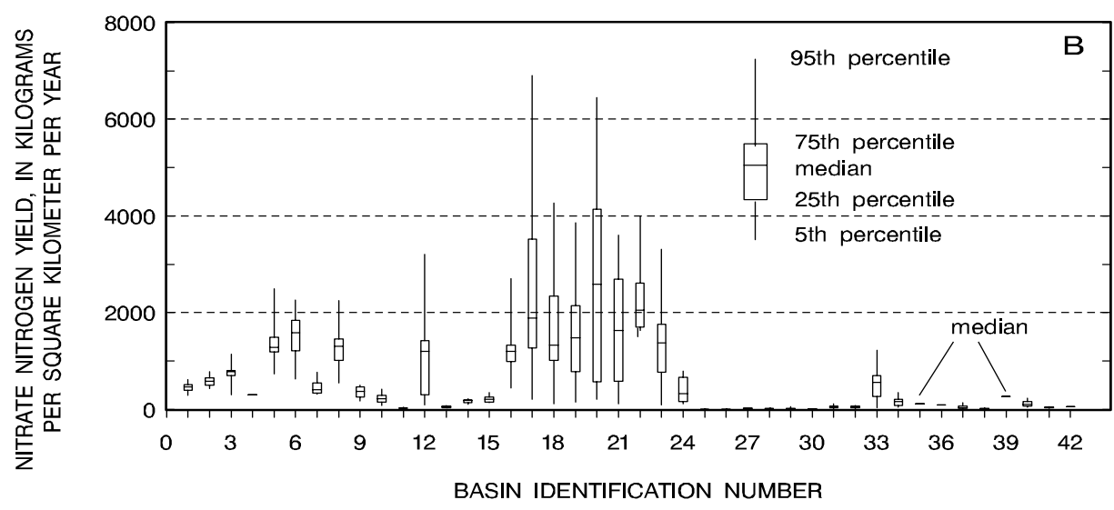
Figure 4.7 (A) Spatial distribution of nitrate yields in the 42 interior basins, and (B) box plots showing distribution of nitrate yields in the 42 interior basins. Dashes (-) show median yields for several sites where other statistics could not be calculated.
