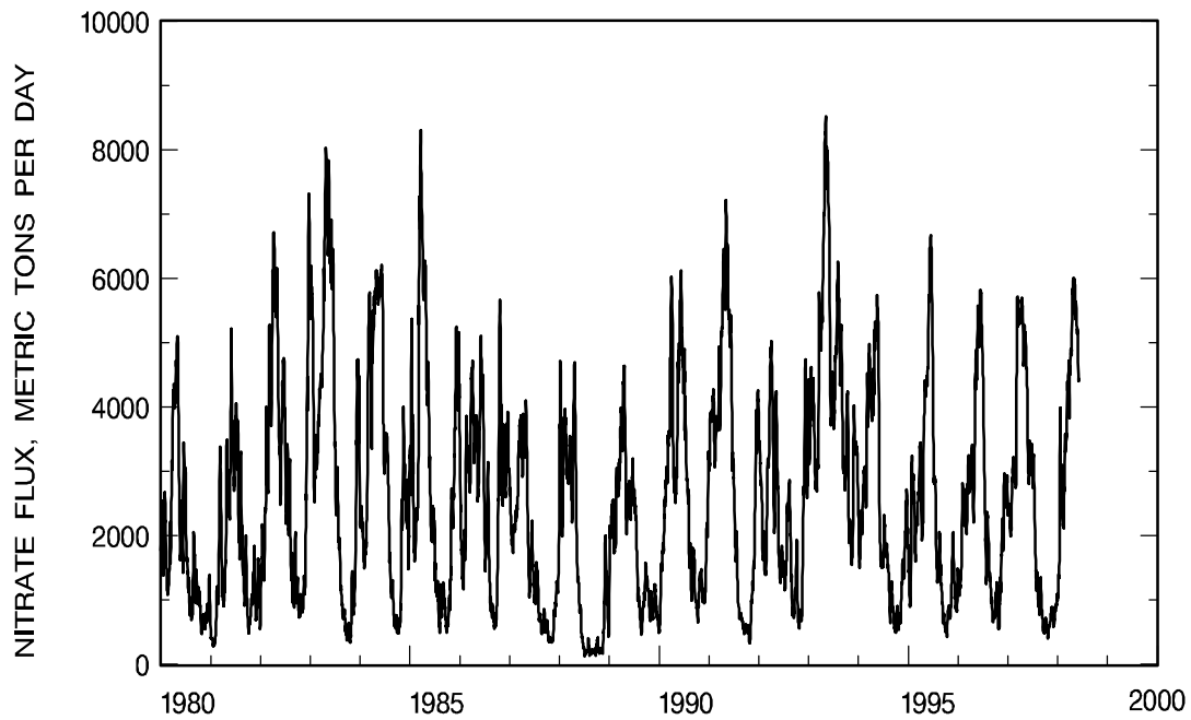
Figure 4.1 Hydrograph of the daily flux of nitrate in the Mississippi River at St. Francisville, LA, 1980-98.
