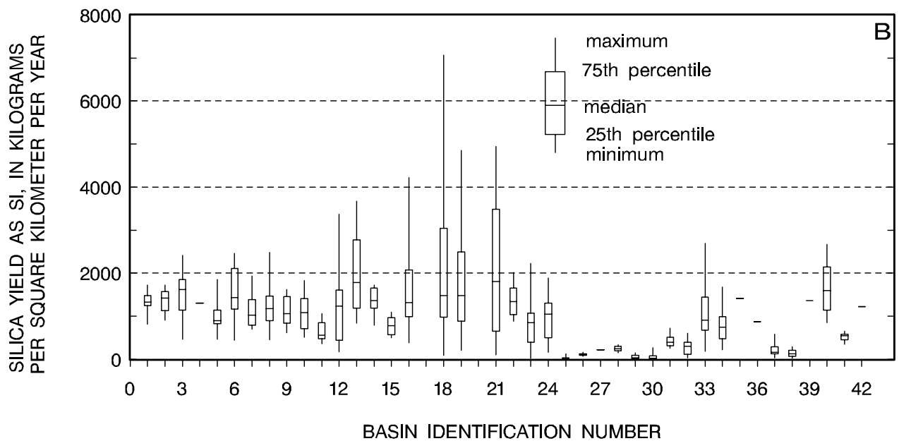
Figure 4.11 (A) Spatial distribution of silica (Si) yields in the 42 interior basins, and (B) box plots showing distribution of silica (Si) yields in the 42 interior basins. Dashes (-) show median yields for several sites where other statistics could not be calculated.
