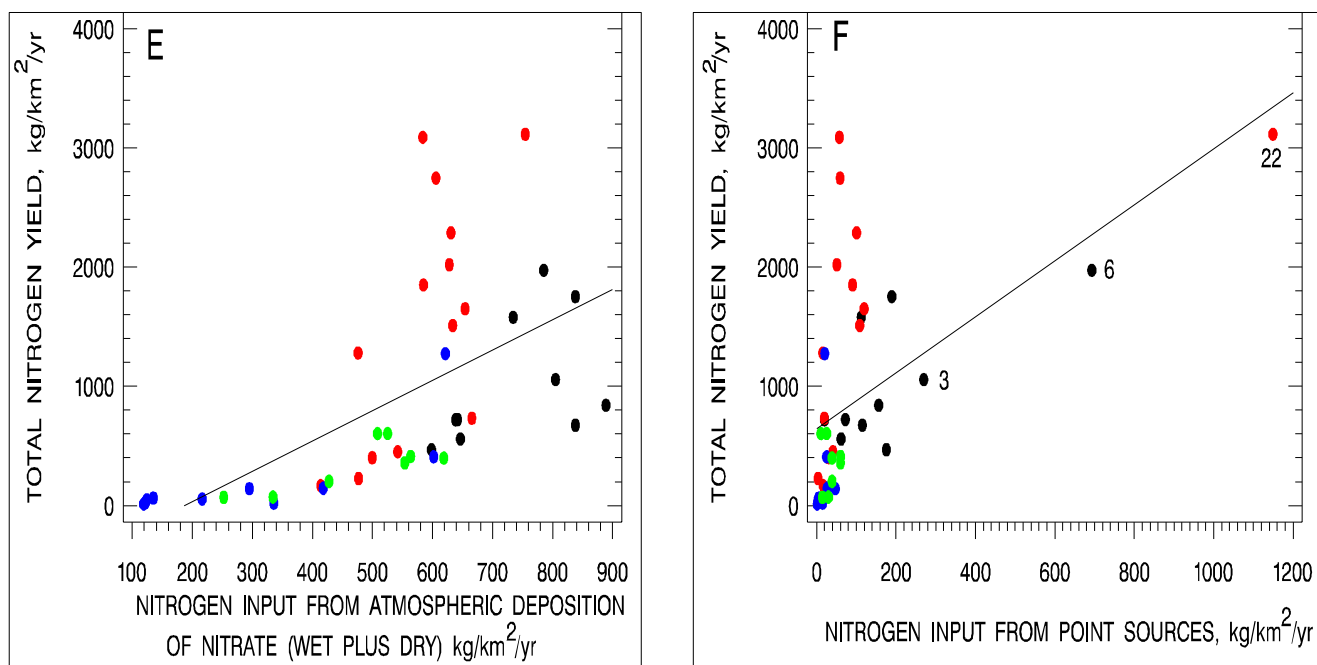
Figure 6.1 Scatterplots showing relations between total nitrogen yield and nitrogen inputs from (A) fertilizer, (B) mineralized soil, (C) legumes, (D) manure, (E) atmospheric deposition of nitrate (wet plus dry), and (F) municipal and industrial point sources.
