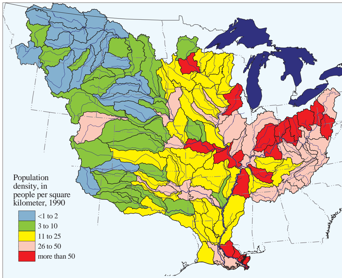
Figure 1.5 Density of population within hydrologic accounting units in the Mississippi basin.
