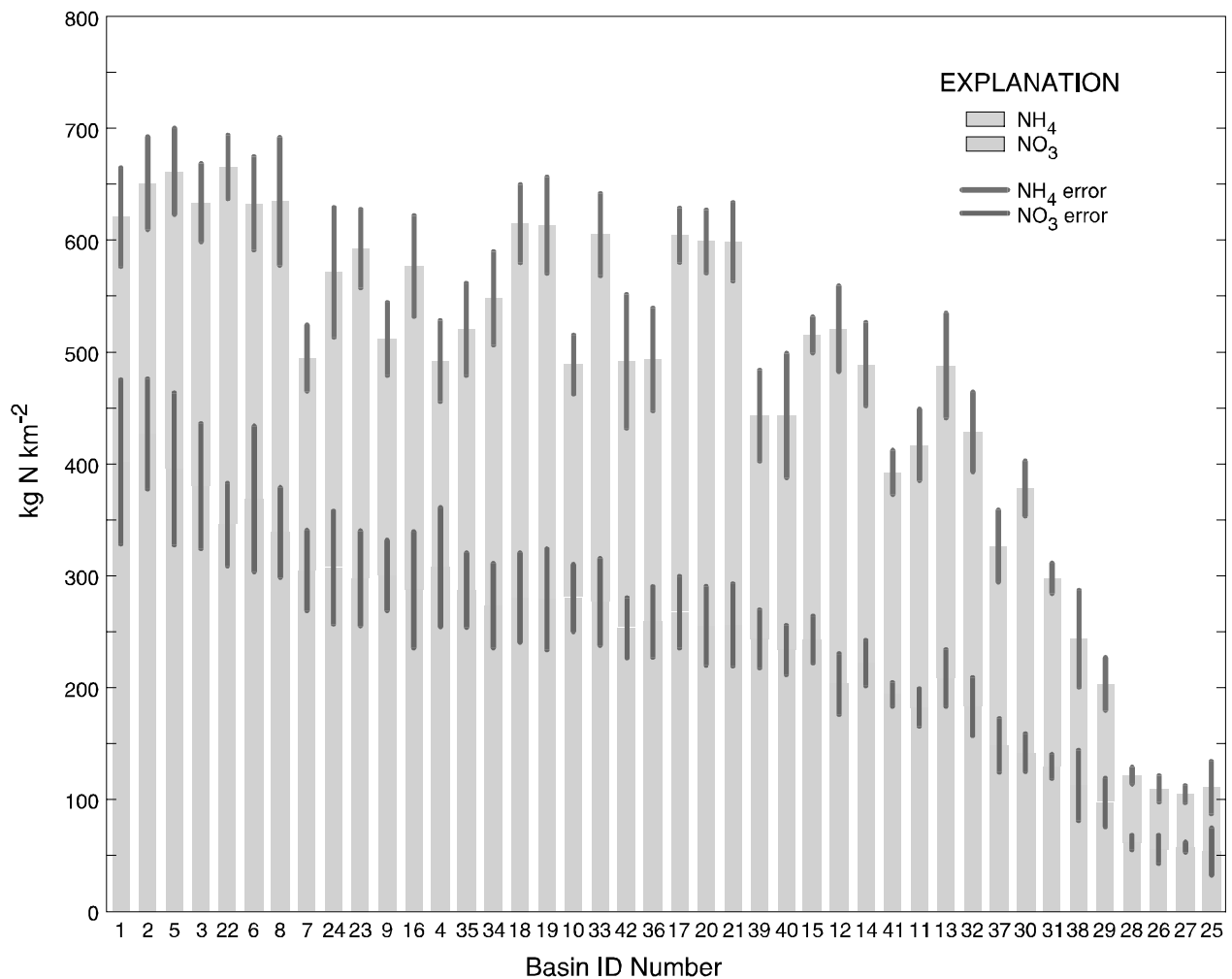
Figure 5.3 Wet deposition of \text{NO}_3 and \text{NH}_4 in 42 subbasins of the Mississippi River basin, averaged for 1990-96 data from the National Atmospheric Deposition Program (NADP, http://nadp.sws.uiuc.edu/ ). Vertical lines represent 1 standard deviation.
