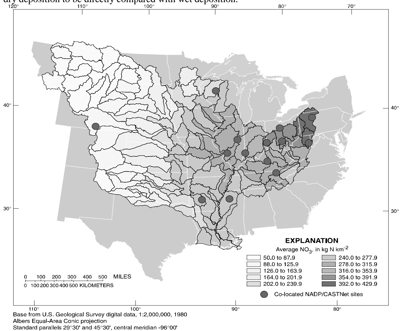
Figure 5.1 Wet deposition of NO 3 , averaged for 1990-96 data from the National Atmospheric Deposition Program (NADP, http://nadp.sws.uiuc.edu/ ), in each the 133 accounting units that make up the Mississippi River basin. Blue circles indicate where NADP and CASTNet (Clean Air Status and Trends Network) sites are co-located.
