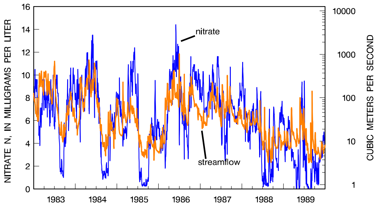
Figure 3.3 Daily streamflow and daily nitrate concentrations in the Raccoon River at Des Moines, IA during 1983-89 (nitrate data provided by Des Moines Water Treatment Plant).
