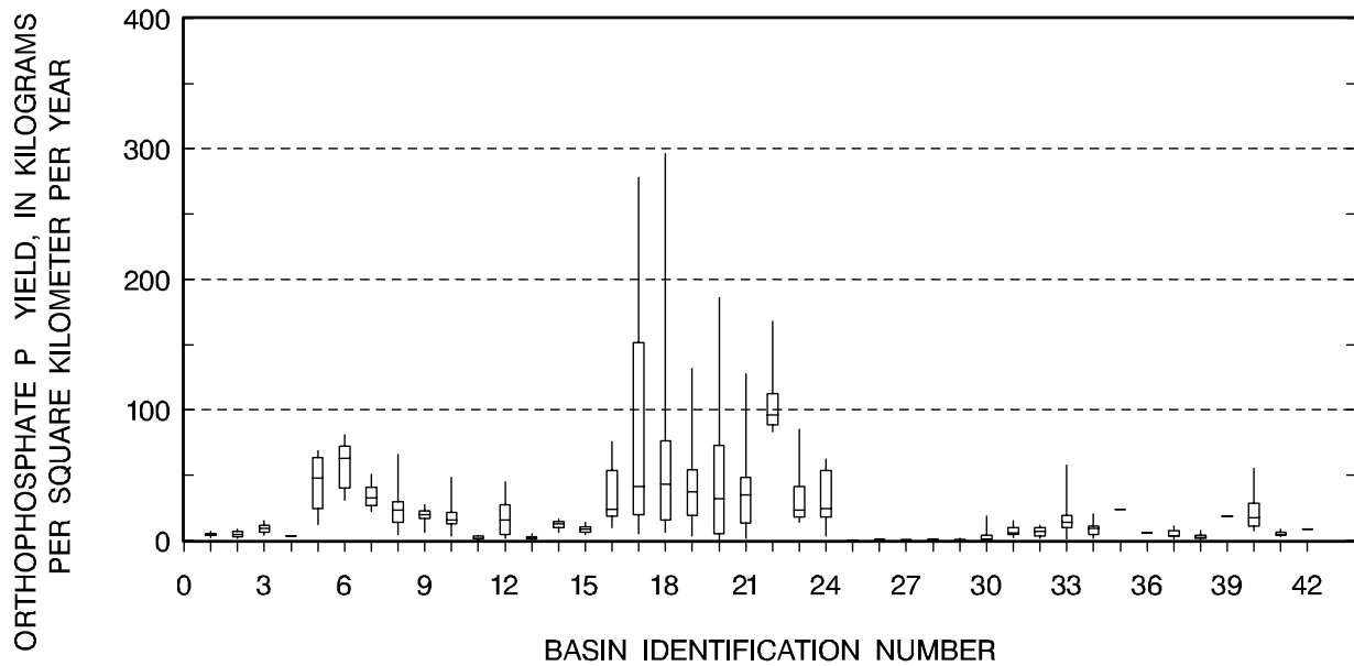
Figure 4.10 (A) Spatial distribution of orthophosphate yields in the 42 interior basins, and (B) box plots showing distribution of orthophosphate yields in the 42 interior basins. Dashes (-) show median yields for several sites where statistics could not be calculated.
