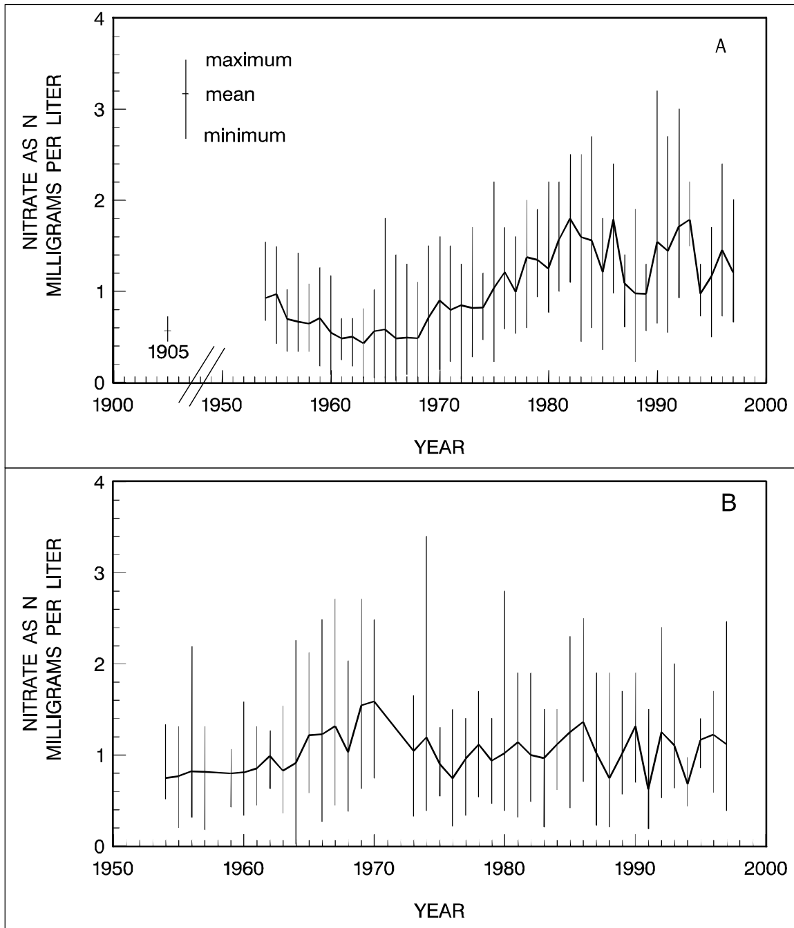
Figure 3.4 Long-term patterns in nitrate concentrations in (A) Mississippi River at St. Francisville, LA and (B) Ohio River at Grand Chain, IL.
