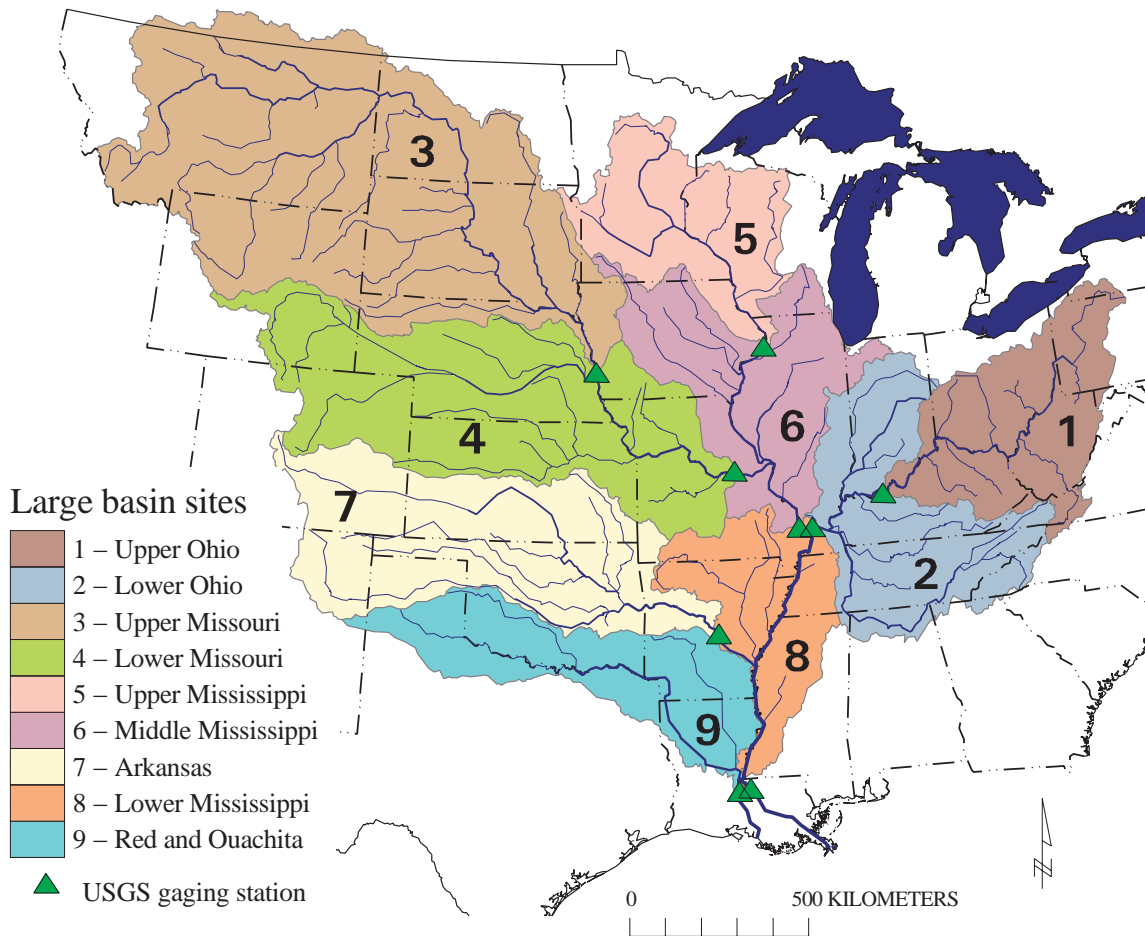
Figure 2.1 Location of nine large basins used for nutrient flux and yield estimates (see table 2.2 for descriptions).
