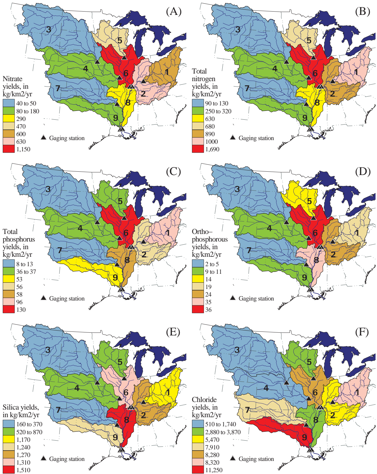
Figure 4.5 Spatial distribution of the average nutrient and chloride yields in nine large basins during 1980-96: (A) nitrate nitrogen, (B) total nitrogen, (C) total phosphorus, (D) orthophosphate phosphorus, (E) silica as Si, (F) chloride.
