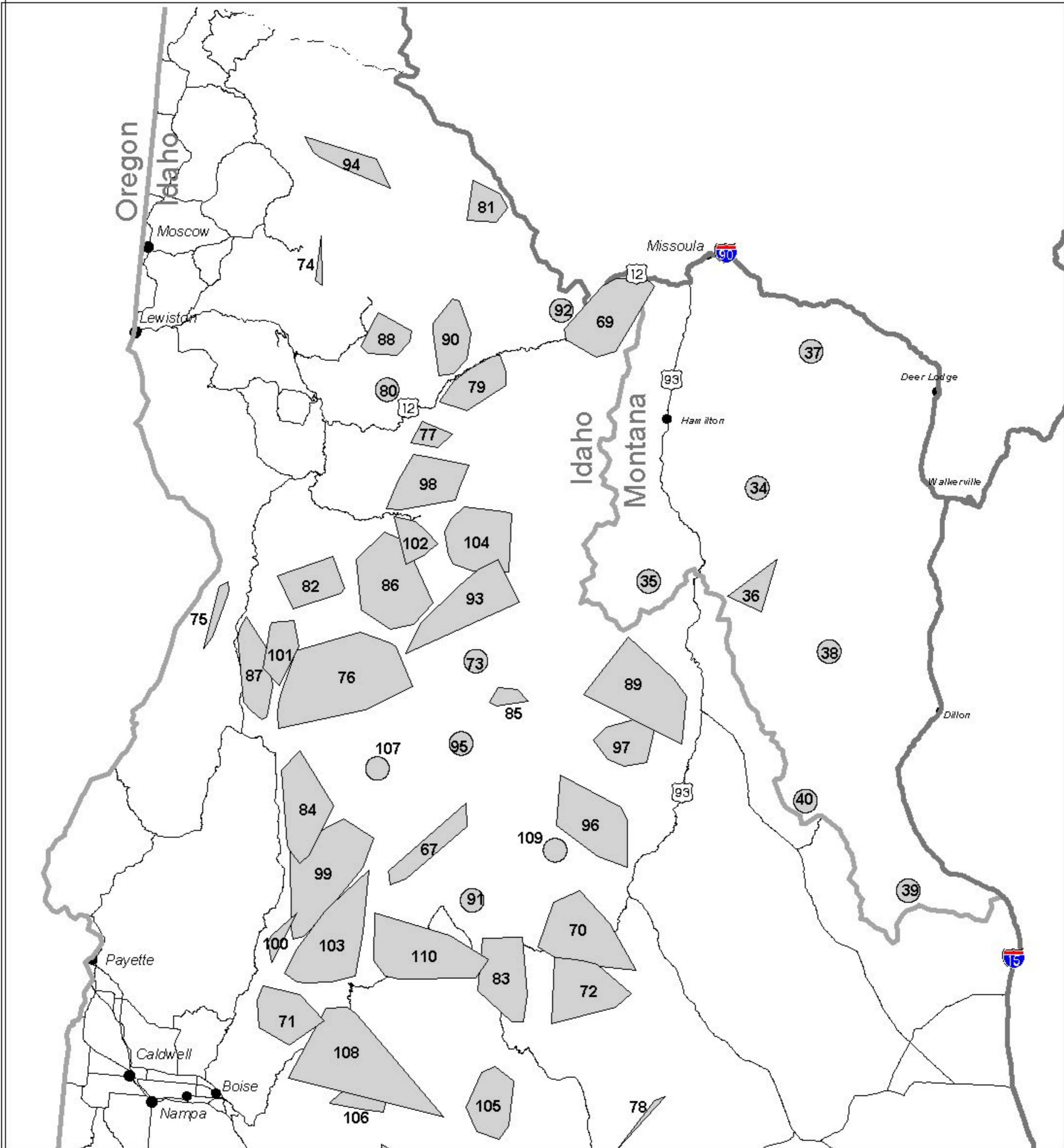
Figure 4. Central Idaho Wolf Recovery Area
