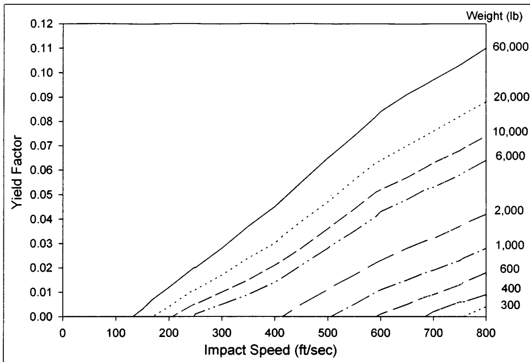
Figure 417.231-2. Chunk Impact on Soil
