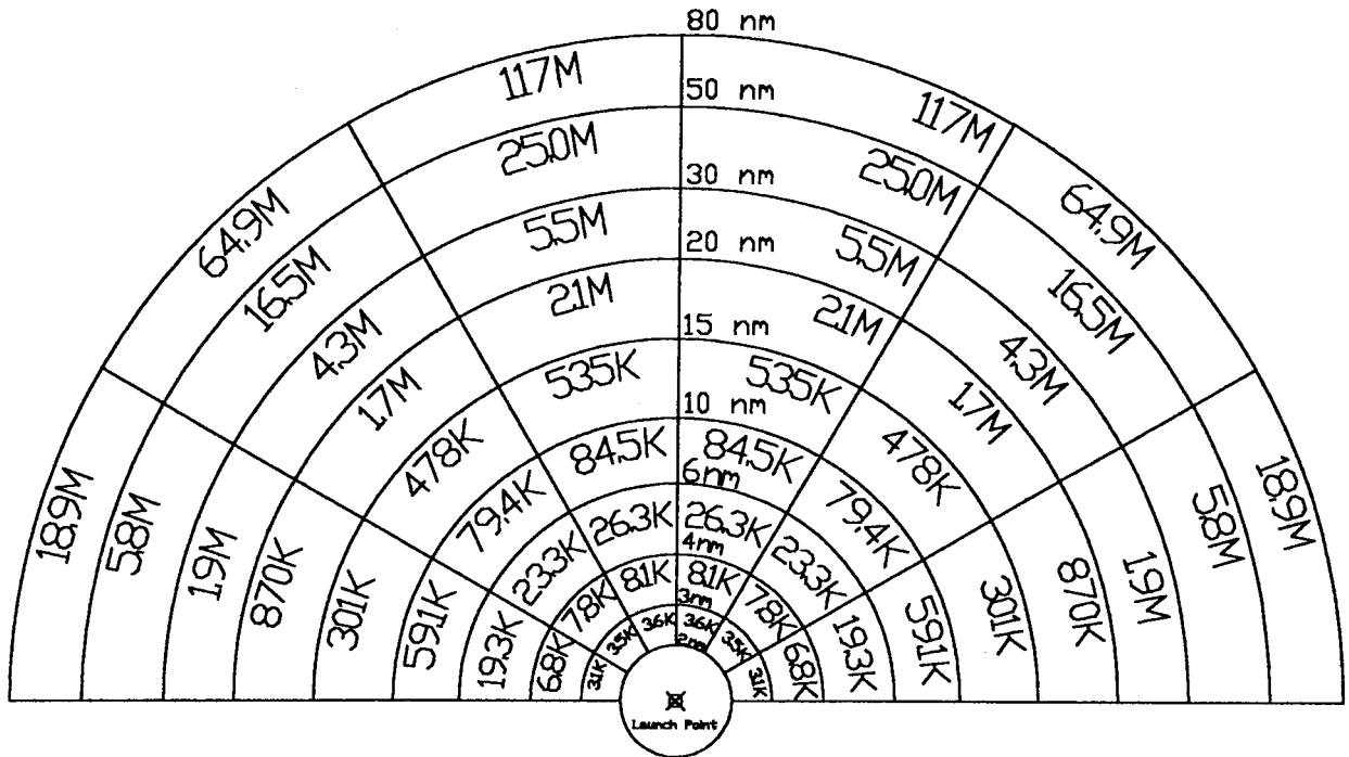
Figure B417.7-1, Population Limits for Large Mature Launch Vehicles
