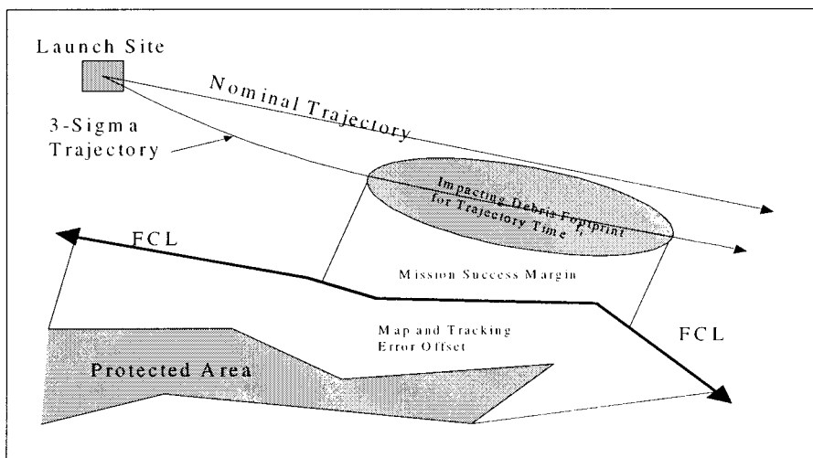
Figure 417.211-1, Illustration of Flight Control Line (FCL) Offsets and
