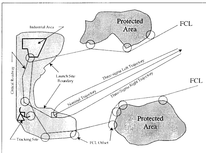
Figure 417.211-2, Illustration of Flight Control Line (FCL) Offsets
