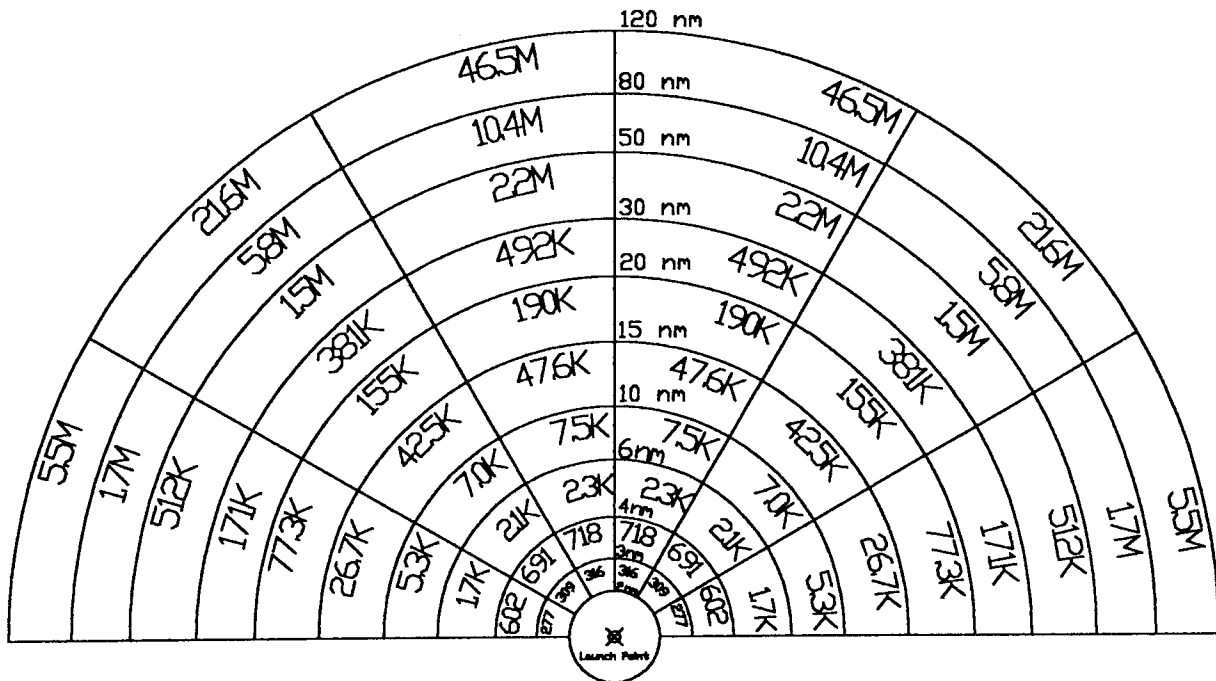
Figure B417.7-3, Population Limits for Large New Launch Vehicles
