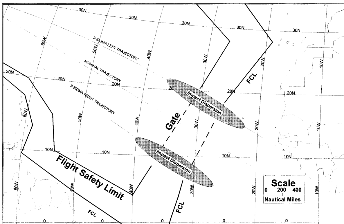
Figure 417.219-2, Example Gate Depiction (Large Scale)
