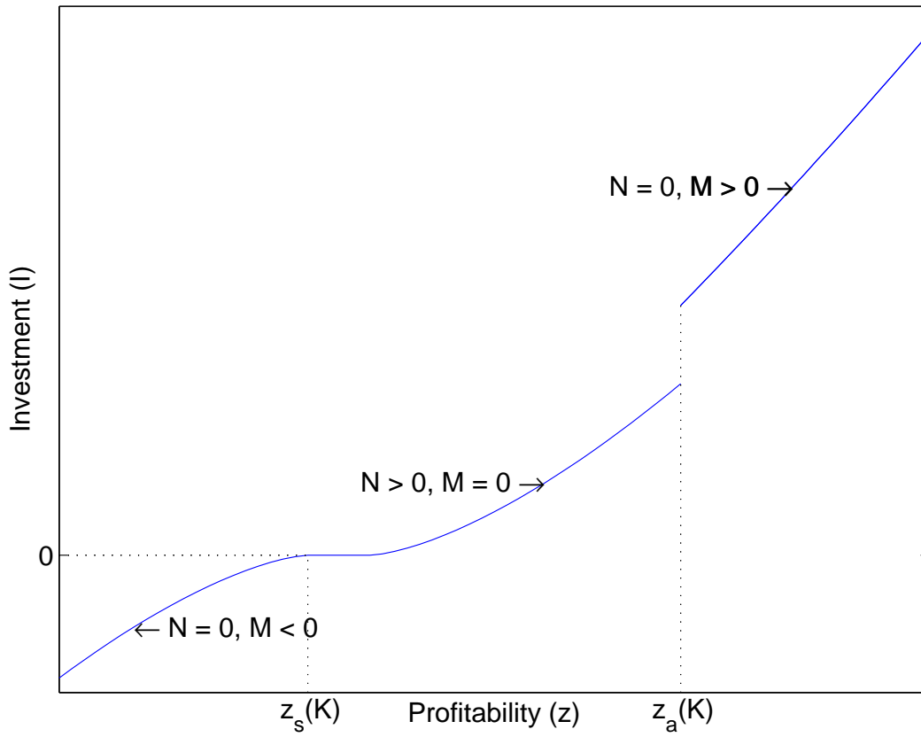
Figure 1: The figure plots optimal investment as a function of profitability z for a firm of fixed size K . z_a(K) denotes the profitability threshold above which the firm buys existing assets from another and z_s(K) denotes the profitability threshold below which the firm sells assets.
