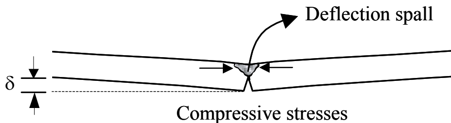
Figure 58. Schematic of deflection spalling mechanism.
