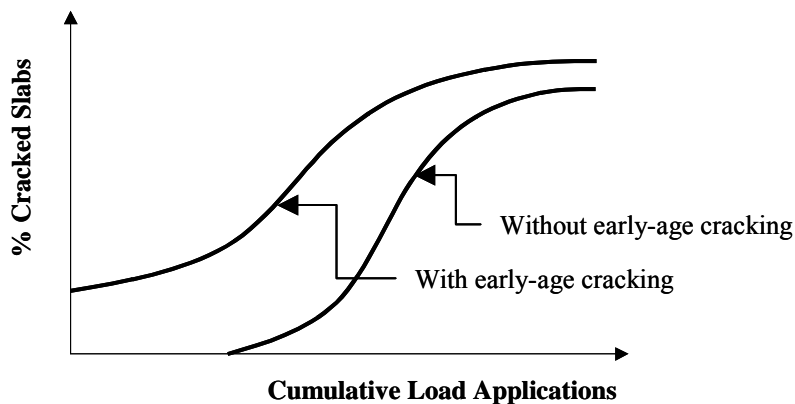
Figure 41. Schematic of long-term performance of JPCP: Percent cracked slabs vs. time.
