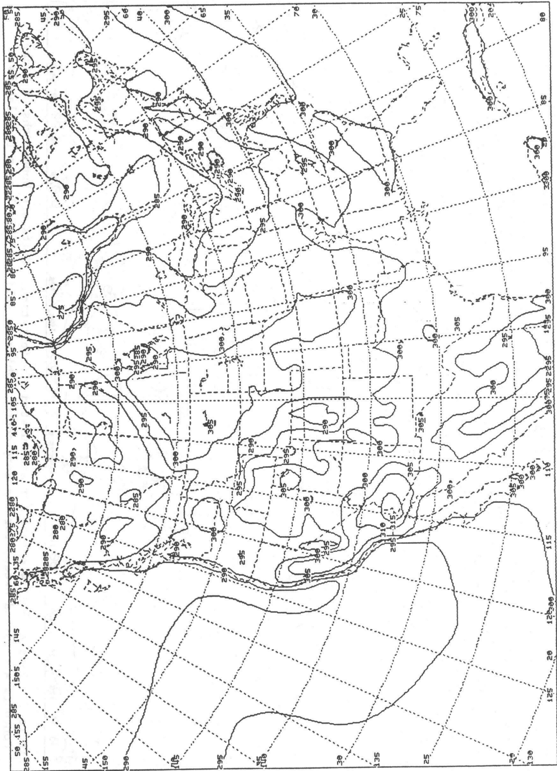
Figure 6. Same as Fig. 4 except for surface temperature. Units are degrees Kelvin.
