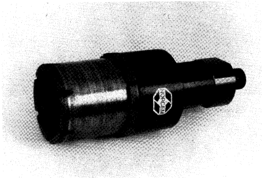
Figure 12. Core drill bit for drilling a core for break-off testing.
