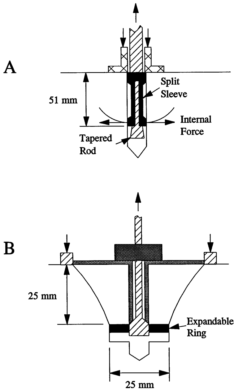
Figure 10. A) Drilled-in test using split-sleeve and tapered bolt. B) CAPO test using rounded shoulder and expandable washer.
