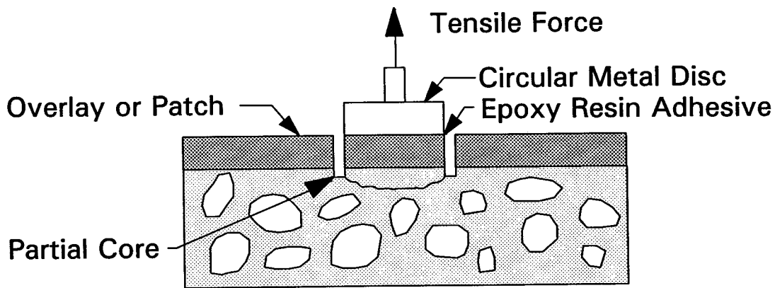
b) Method for testing partially cored concrete
