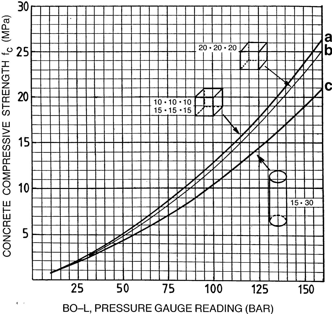
Figure 18. Strength diagram for "L-level."
