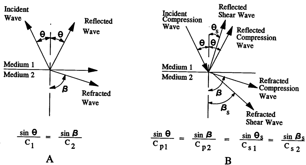
Figure 27. The behavior of a P-wave incident upon an interface between two dissimilar media: (A) reflection and refraction; (B) mode conversion.
