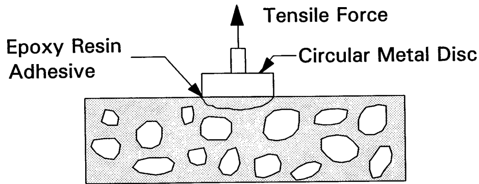
a) Method for testing uncured concrete
