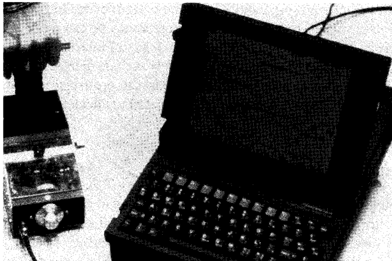
Figure 29. Impact-echo equipment. Impact source and receiving transducer housed in unit to the right of the laptop computer (waveform analyzer).
