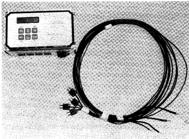
Figure 23. System 4101 maturity meter.
