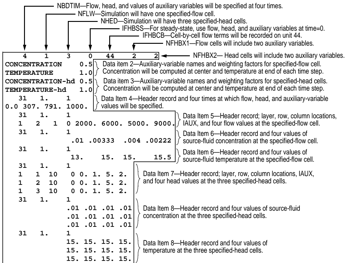
Figure 8. Annotated example input data set for FHB1. Input data are enclosed in border.
