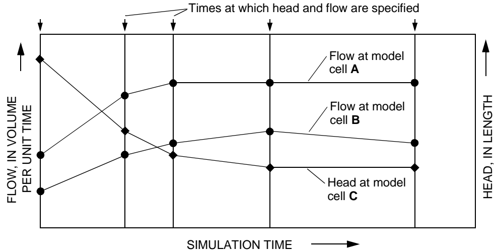
Figure 1. An example of definition of functions of flow and head for individual model cells. With this procedure, the total volume of flow at each specified-flow cell for a simulation does not vary with number and length of time steps used in the simulation.
