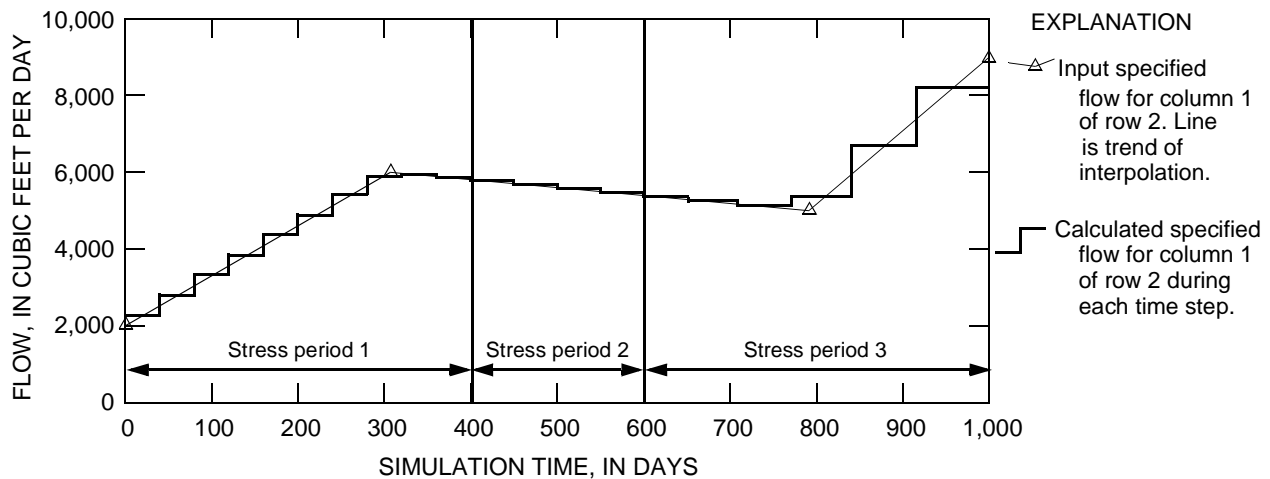
Figure 6. Input and calculated specified flow for cell in column 1 of row 2.
