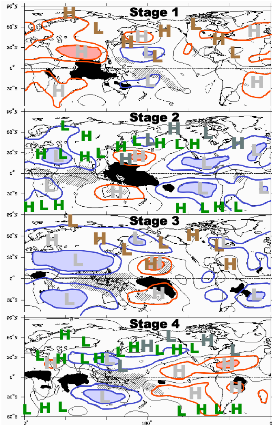
Figure 13. The four stages of the global synoptic-dynamic model (SDM) of subseasonal variability for the northern hemisphere cold season (November-March). The red (blue) isopleths and shading depict subtropical anticyclonic (cyclonic) 200mb streamfunction anomalies (inter-hemispheric sign reversal understood) that accompany MJO tropical convection anomalies as they move east. The black (hatched) shading shows the areas of enhanced (suppressed) convection with the MJO. The “Hs” and “Ls” are used to show the associated anomalous anticyclonic (or “high pressure”) and cyclonic (or “low pressure”) gyres. The lighter gray “Hs” and “Ls” are for the MJO while the heavier gray ones illustrate a west Pacific wavetrain linked to the MJO at Stage 2. The brown “Hs” and “Ls” depict teleconnection patterns associated with the frictional torque, and the green ones show synoptic-scale wavetrains. See text for additional details.
