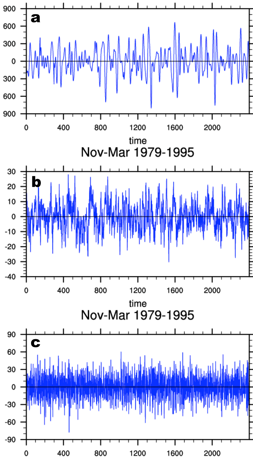
Figure 8. Indices for 16 winter segments from November-March 1979-1980 to 1994-1995 for (a) the first EOF of 20-100 day filtered outgoing longwave radiation (OLR) represents the MJO, (b) the daily global frictional torque with the MJO linearly removed represents teleconnection patterns, and (c) the <30 day filtered global relative AAM tendency represents wave energy dispersion over the mountains. The abscissas are time expressed as days while the ordinates are non-dimensional measures of amplitude.
