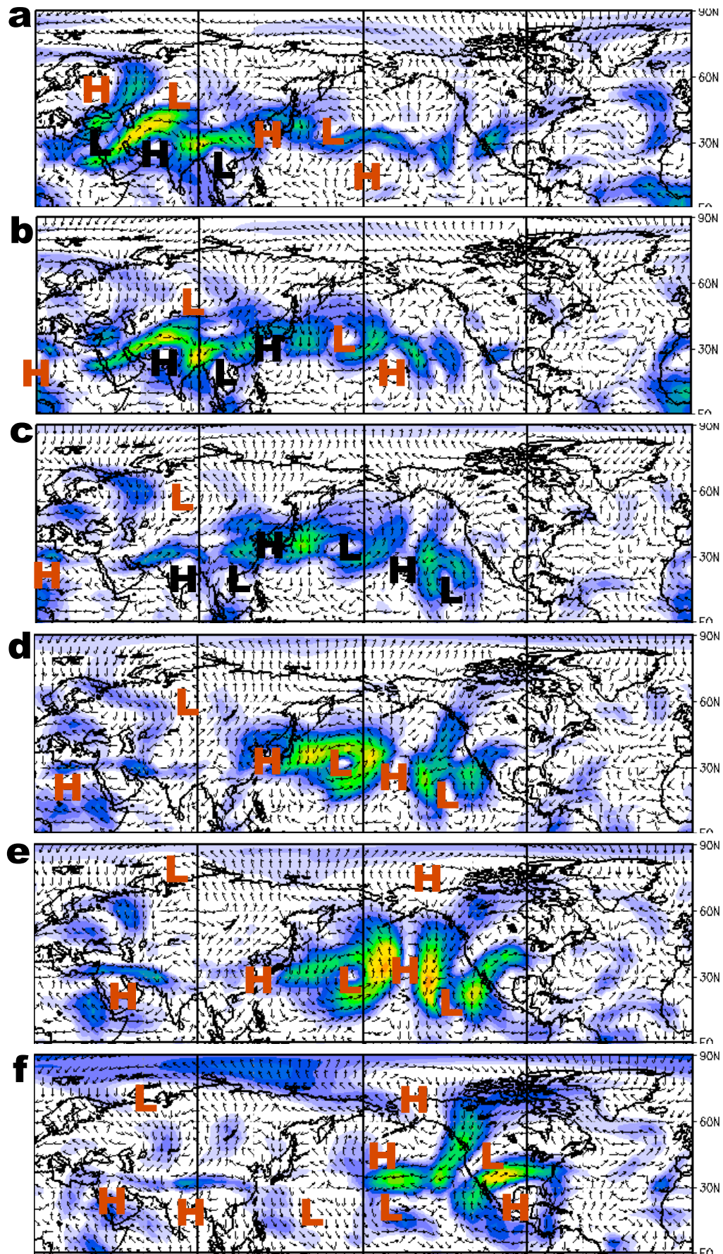
Figure 6. Same as Fig. 5 but for T2, the transition to Stage 1 of the GSDM. Dates are (top to bottom): January 12, 13, 14, 15, 16 and 18.
