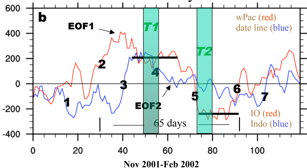
Figure 4. Time series plots (same format as Fig. 3) for the period of 1 November-28 February. a) the first EOF of the zonal integral of the mountain and frictional torque (top panel; red is mountain torque/blue is frictional torque). b) the first 2 EOFs of 20-100 day filtered OLR (red is EOF1/blue is EOF2). The text indicates the location of anomalous convection corresponding to positive and negative values of each EOF. IO refers to Indian Ocean. Shaded vertical bars represent T1 and T2. Additional details are in the text.
