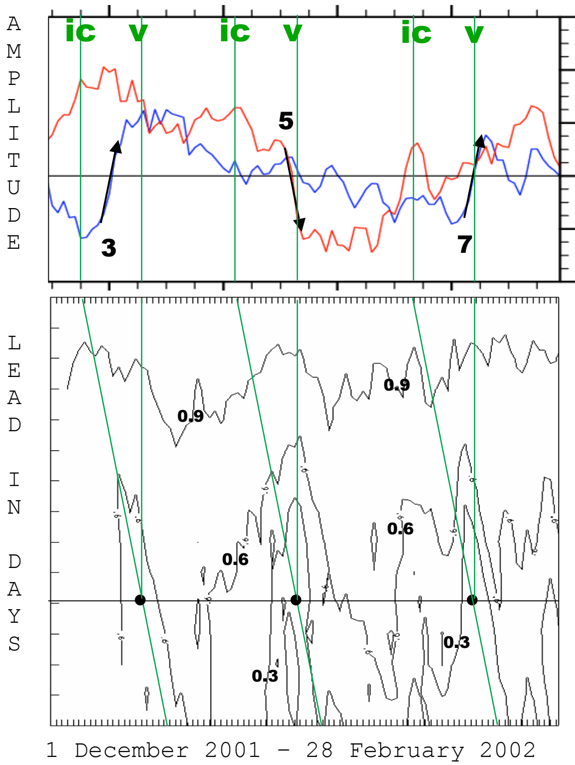
Figure 7. Time series plots of OLR EOFs 1 and 2 (as in Fig. 4), top panel, and forecast skill for a forecast model ensemble mean, bottom panel, during the period of 1 December 2001-28 February 2002 (abscissa, days increasing from left to right). “ic” and “v”, and the vertical lines highlight the model initial condition and verification times for the three cases discussed in the text. Verification is expressed in terms of anomaly correlation coefficient over the entire northern hemisphere of 150-mb streamfunction anomalies. The contour interval on the bottom panel is 0.3, and the black dots show the dates of lowest day 11 forecast skill. The slanted lines indicate the model forecast cycle (day 1 to day 15 lead). The horizontal line highlights day 11 lead.
