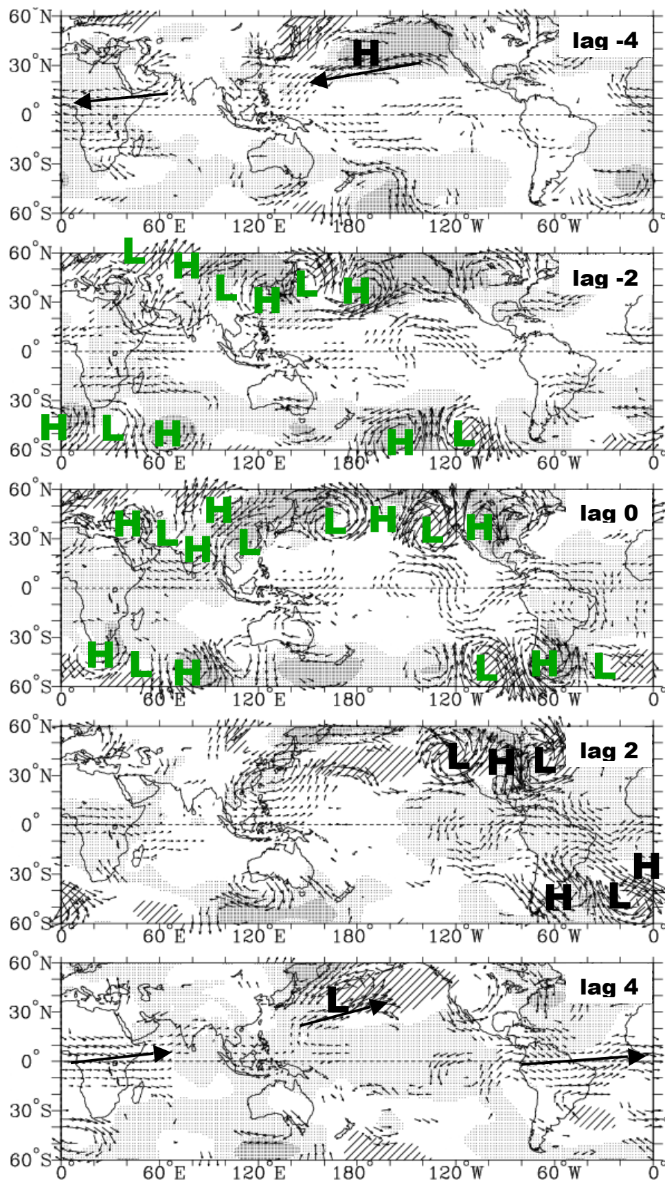
Figure 12. Same as Fig. 10 except lag regressions on the <30 day filtered, global relative AAM tendency index given on Fig. 8c (sequence 3). The green Hs and Ls are placed on Fig. 13 as part of Stage 2 and Stage 4 (opposite phase) of the GSDM.
