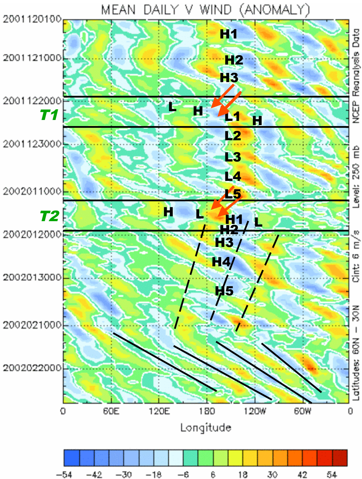
Figure 2. Hovmoller plot of 250mb meridional wind anomalies averaged from 30-60N during the period of 1 December 2001-28 February 2002. The solid horizontal lines depict the periods for T1 and T2, and the “Hs” and “Ls” highlight positions of anomalous synoptic-scale troughs and ridges, respectively. The red arrows indicate retrogression of existing anomalies while the light dashed lines show a slow westward regime shift. The slanted solid black lines indicate progressive circulation anomalies after 1 February 2002.
