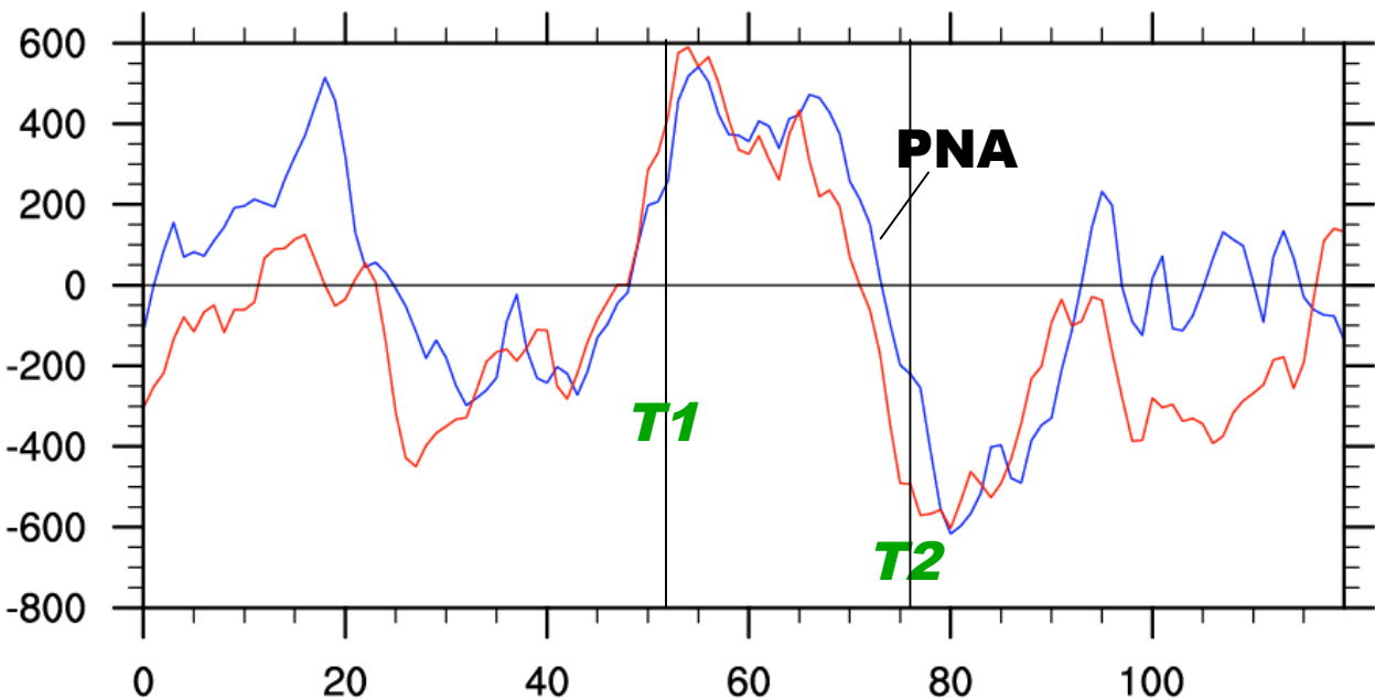
Figure 3. Time series plots of indices describing low frequency variations for the period of 1 November 2001-28 February 2002. The days are on the abscissa, where day 0 is for 1 November and increasing from left to right. The numbers on the ordinate of the upper panel are AAM units = 1.0 \times 10^{24} \text{kgm}^2 \text{s}^{-1} and on the lower panel are dimensionless measures of amplitude. The top panel is for the global integral of AAM while the bottom shows the plots for the first EOF of the combined 200/850mb vector wind field (red) and the PNA (blue). The vertical lines depict the center date for T1 and T2.
