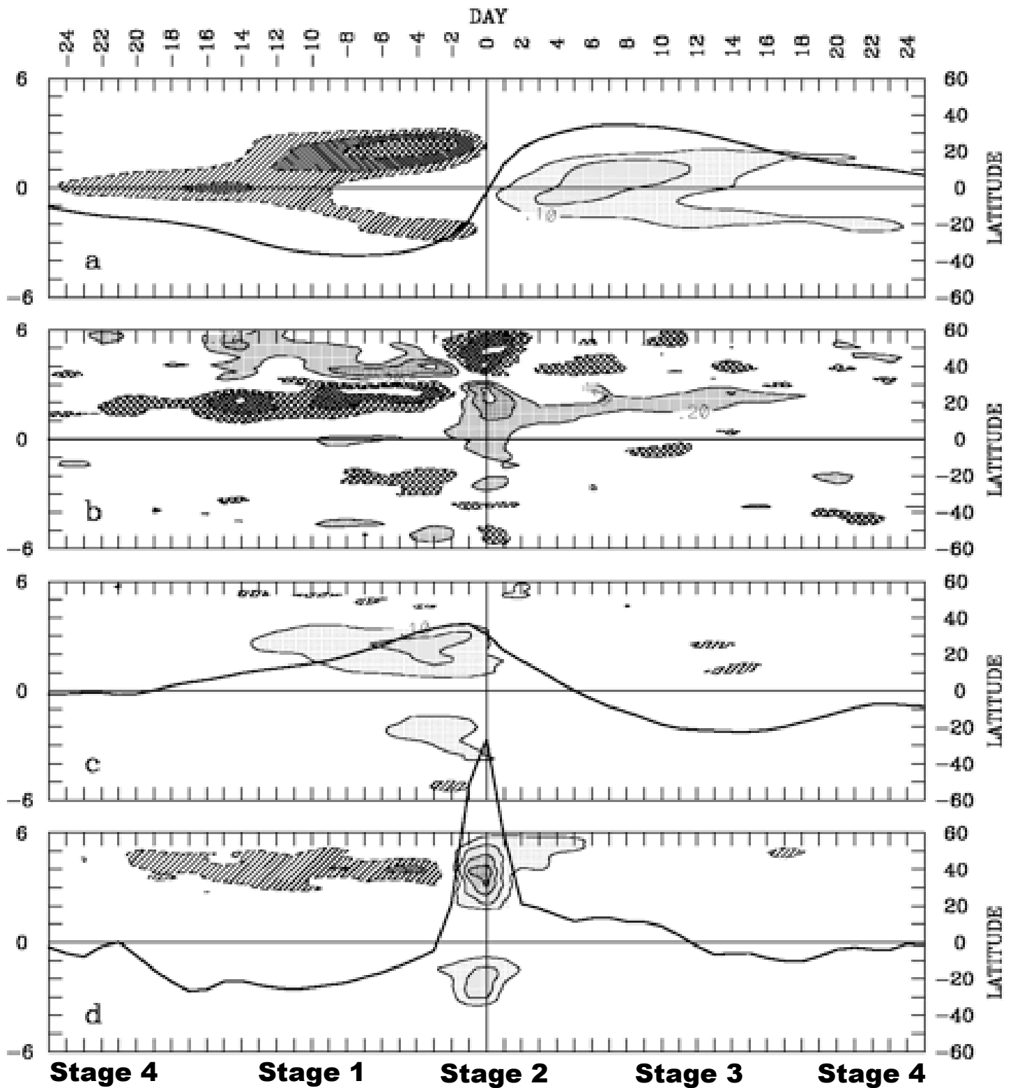
Figure 14. Zonal (contours and shading) and global (curves) anomalies obtained by lag regression onto the daily global relative AAM tendency for November- March 1979-80 to 1994-95. (a) Total AAM: contour interval is 0.1 \times 10^{24} \text{ kgm}^2 \text{ s}^{-1} , left ordinate labels are for global curve in AAM units (1 unit = 1.0 \times 10^{24} \text{ kgm}^2 \text{ s}^{-1} ). (b) The flux convergence of relative AAM: contour/shading interval is 0.2 Hadleys, left ordinate labels are Hadleys. (c) the frictional torque: same as b) except contour/shading interval is 0.1 Hadleys. (d) the mountain torque, same as c). Note that the contour interval in b) is twice that in c) and d). The right ordinate labels are latitude for the zonal contours.
