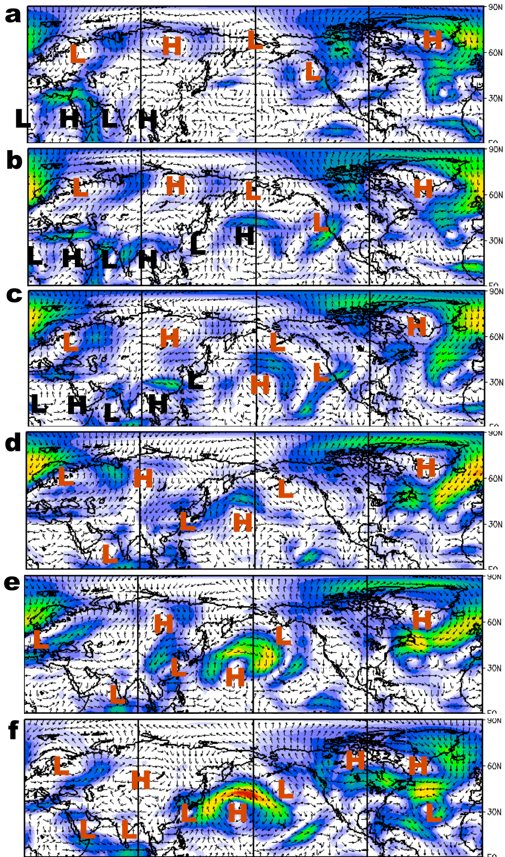
Figure 5. The daily evolution of 150mb vector wind anomalies for T1, the transition to Stage 3 of the GSDM. “Hs” and “Ls” refer to anomalous anticyclonic and cyclonic circulations. From top to bottom the dates are: December 19, 20, 21, 22, 23 and 25. The vertical lines highlight 90E, 180E and 90W.
