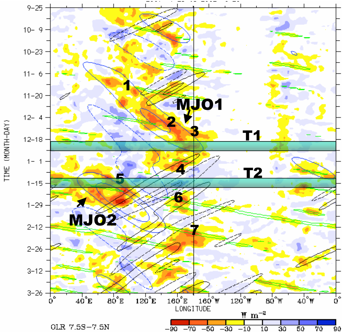
Figure 1. Hovmoller plot (time-longitude section) of OLR anomalies averaged between 7.5 deg. N-S, where the contours illustrate space-time filtered coherent tropical convection modes for 25 September 2001-26 March 2002. The blue contours represent the MJO (solid blue for enhanced convective phase/dashed for suppressed phase). The green contours are for Kelvin waves and the brown contours isolate an equatorial Rossby mode. See Wheeler and Kiladis (1999) for additional details. MJOs 1 and 2, T1 and T2, and the 1-7 numbering refer to important developments discussed in the text and listed in Table 1. The lightly shaded horizontal bars highlight the transitions for the case study, with T1 (T2) from 19-25 December 2001 (12-18 January 2002).
