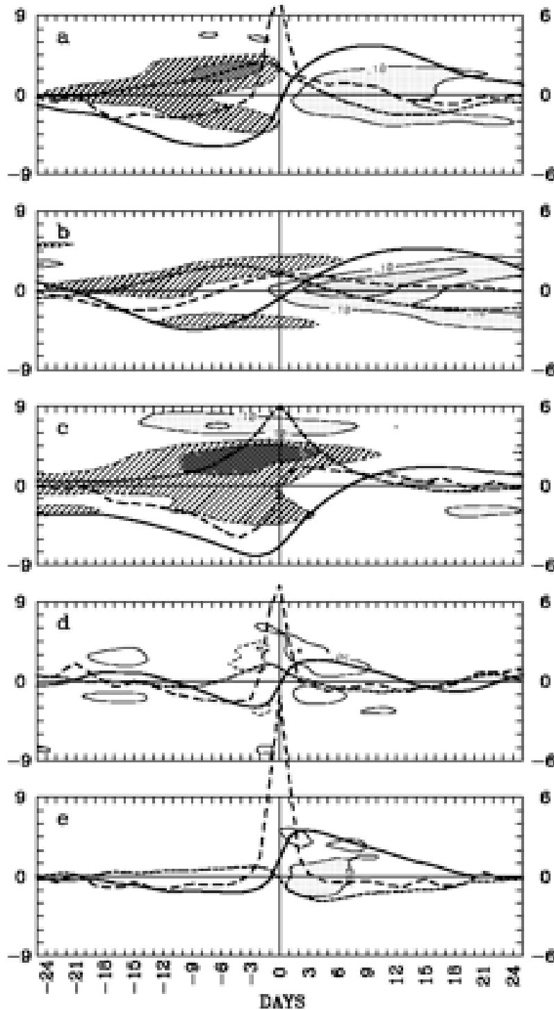
Figure 9. The total global atmospheric angular momentum (solid curve), the global mountain torque (long dash curve) and the global frictional torque (short dash curve) anomalies obtained by lag regressions onto various indices using sixteen northern winter seasons (November-March 1979-95). The left ordinate labels are Hadleys (1 Hadley = 1.0 \times 10^{18} \text{ kgm}^2 \text{ s}^{-2} ) and the right labels are AAM units (1 unit = 1.0 \times 10^{24} \text{ kgm}^2 \text{ s}^{-1} ). The abscissa is lag where negative (positive) values mean the regressed quantity leads (lags) the index. For the contours, the right labels also represent latitude/10, i.e., 6=60N, etc. The contour and shading interval is 0.1 \times 10^{24} \text{ kgm}^2 \text{ s}^{-1} (the value corresponds to a vertical and zonal mean zonal wind anomaly of 0.3 \text{ ms}^{-1} at 30N). The contours start at 0.05 \times 10^{24} \text{ kgm}^2 \text{ s}^{-1} in Fig. 9d. The indices used are: a) the daily global AAM tendency, b) the first EOF of 20-100 day filtered outgoing longwave radiation, c) the global frictional torque minus the MJO (see text), d) the global relative AAM filtered to retain < 30 day periods and e) the global mountain torque.
