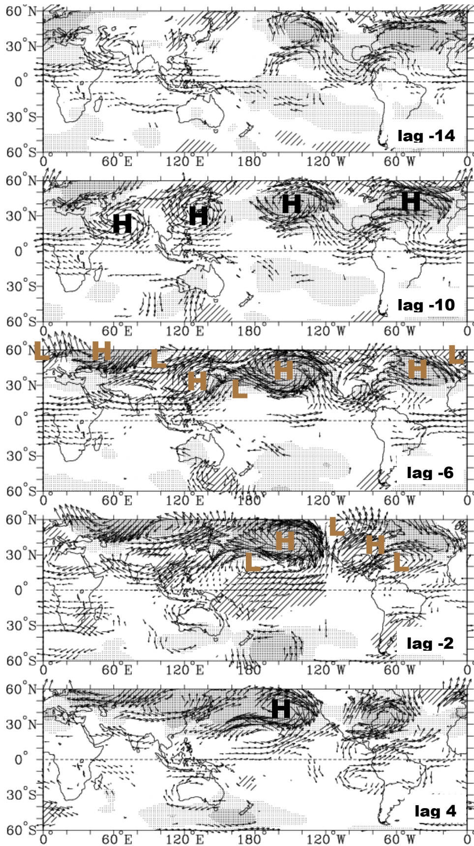
Figure 11. Same as Fig. 10 except lag regressions onto the daily global frictional torque shown in Fig. 8b (sequence 2). The brown Hs and Ls are placed on Stage 1 and Stage 3 (opposite phase) of the GSDM.
