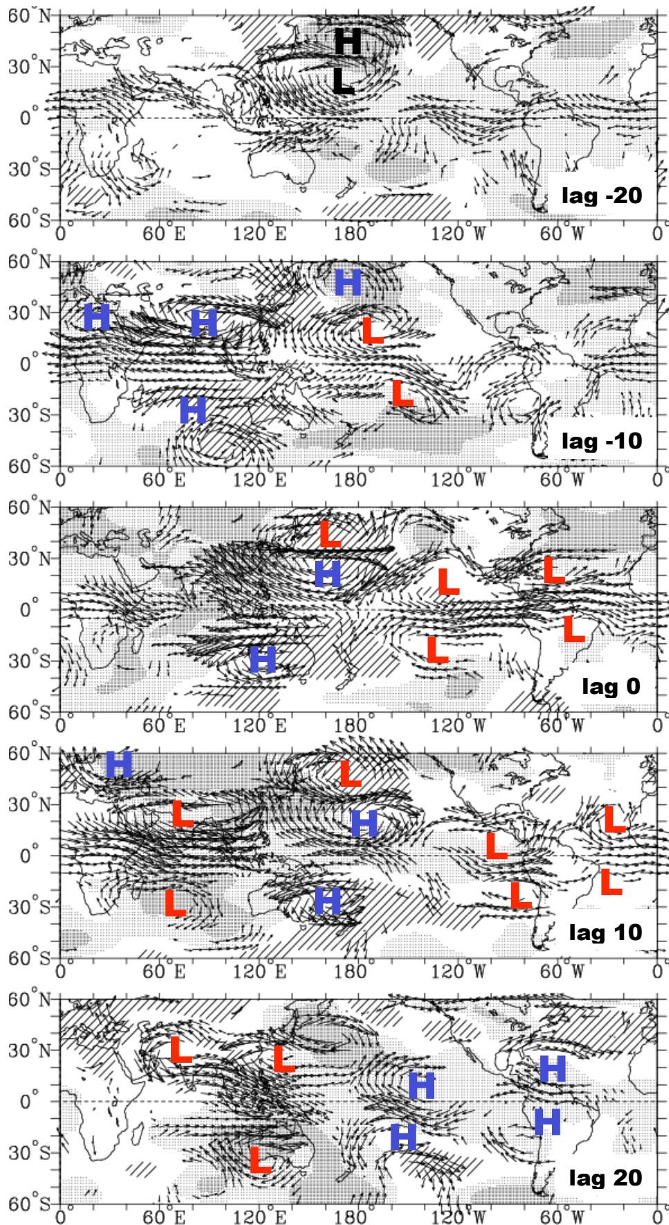
Figure 10. 200mb vector wind (arrows) and sea-level pressure anomalies (shading) obtained by lag regression onto EOF 1 of 20-100 day filtered OLR shown in Fig. 8a (sequence 1). For the sea-level pressure anomalies, stippling (hatched) represents anomalously high (low) pressure. The “Hs” and “Ls” depict anticyclonic (cyclonic) 200mb vector wind anomalies. Only wind anomalies locally significant at 95% are plotted. The red and blue Hs and Ls approximately correspond to the light gray Hs and Ls on Fig. 13 (see also Table 2).
