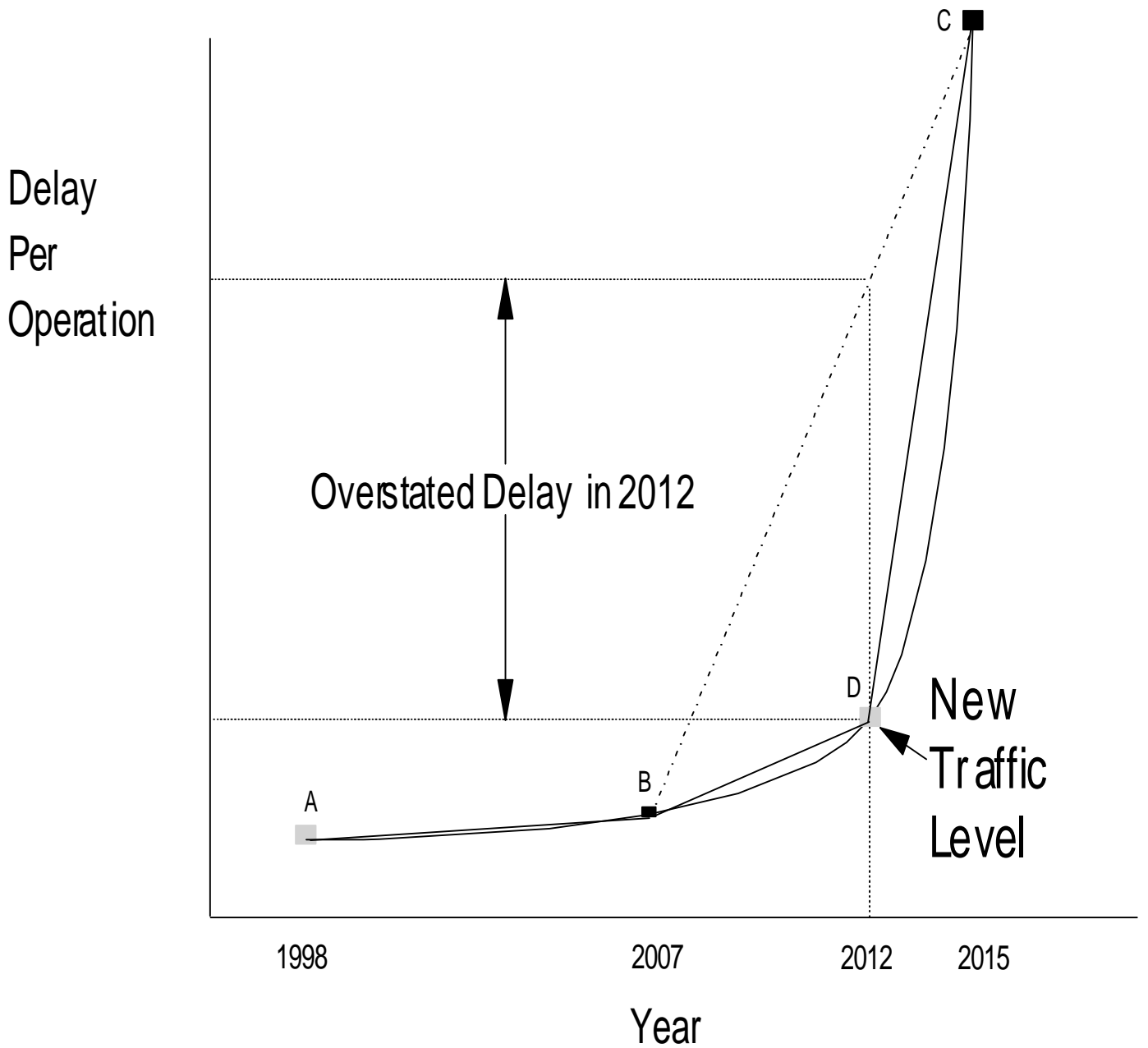
Figure 10.1: Approximation of Exponential Delay Curve
