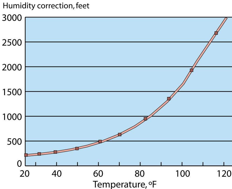
Figure 2. Humidity correction versus temperature plotted over the range of 32°F to 110°F.
