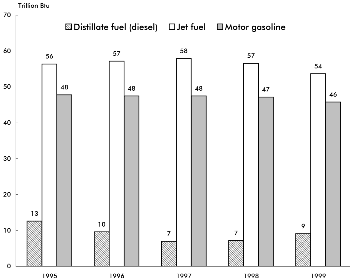
Figure 7-2: Hawaii Transportation Energy Consumption
