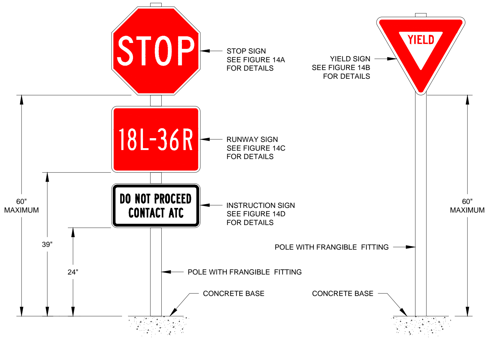
Figure 14. STOP and YIELD Sign Assemblies.
