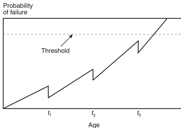
FIGURE 1 Probability of Failure of a Single Aircraft
