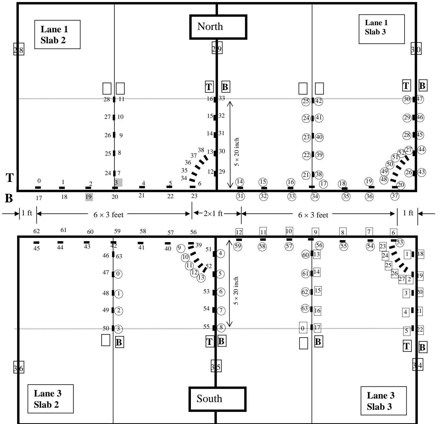
CONCRETE STRAIN GAGE LOCATIONS IN ITEM LRS
