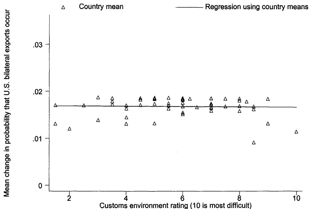
Figure C-1 Mean predicted change, due to a 1-unit improvement in the customs rating, in the probability that a country imports a product from the U.S., relative to the customs environment rating in a given country
