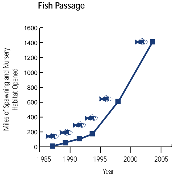
Chesapeake Bay Program-fish passage improvement. As of 1994, 160 river miles of nursery and spawning grounds have been reopened. Five year goal of 582 total miles.
