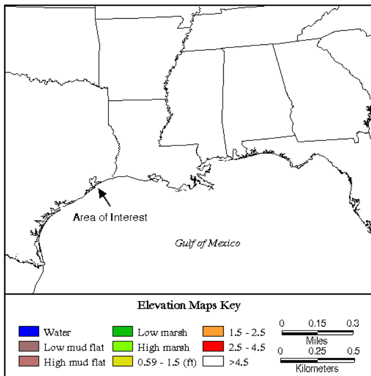
Figure 2. Alternative Ways of Characterizing Elevations Using Digital Elevation Models and National Wetland Inventory; Bolivar Peninsula, Galveston, Texas.
