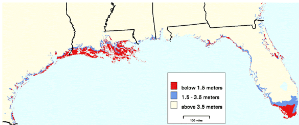
Figure 4. Lands Close to Sea Level: U.S. Gulf Coast
