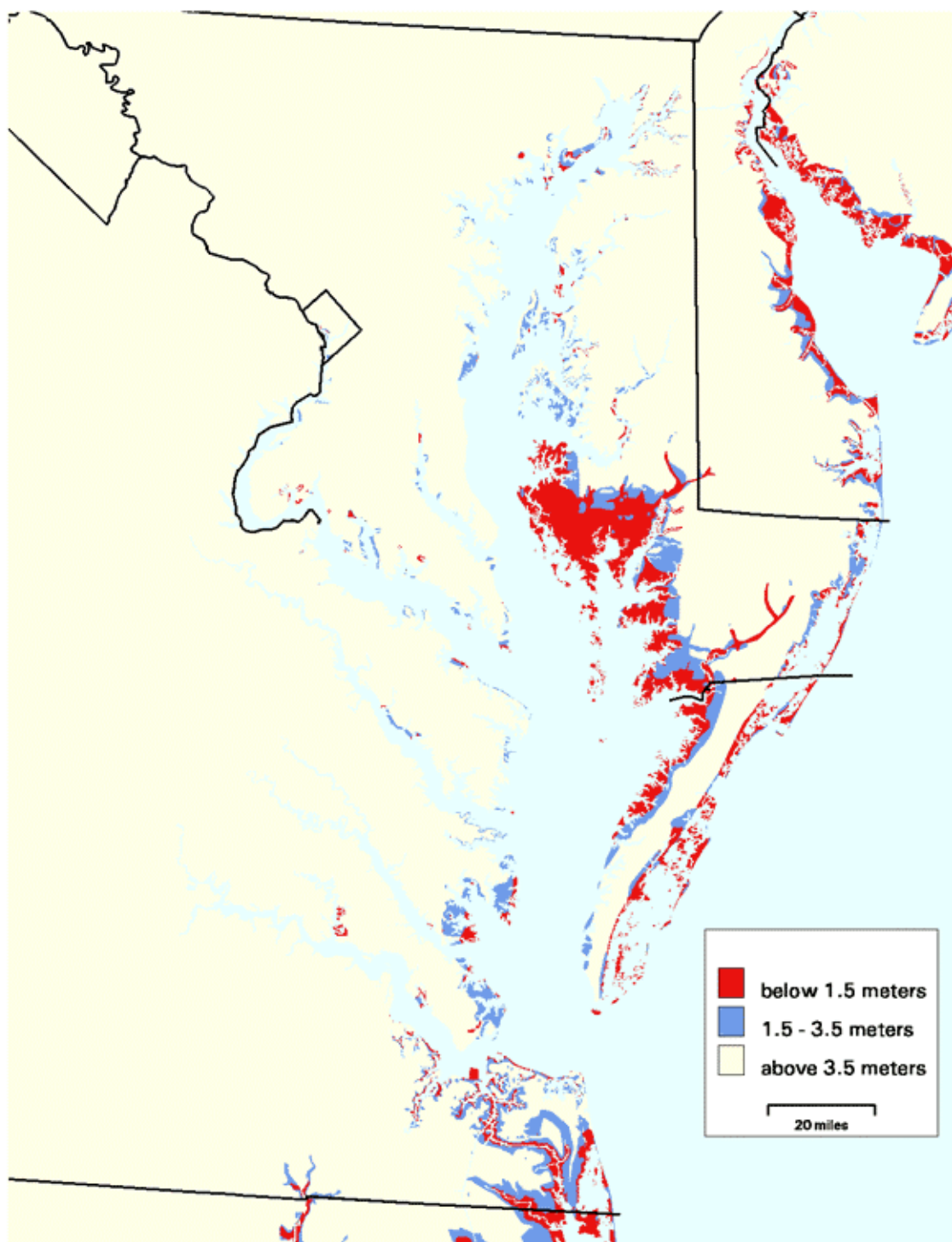
Figure 6. Lands Close to Sea Level: Chesapeake and Delaware Bays
