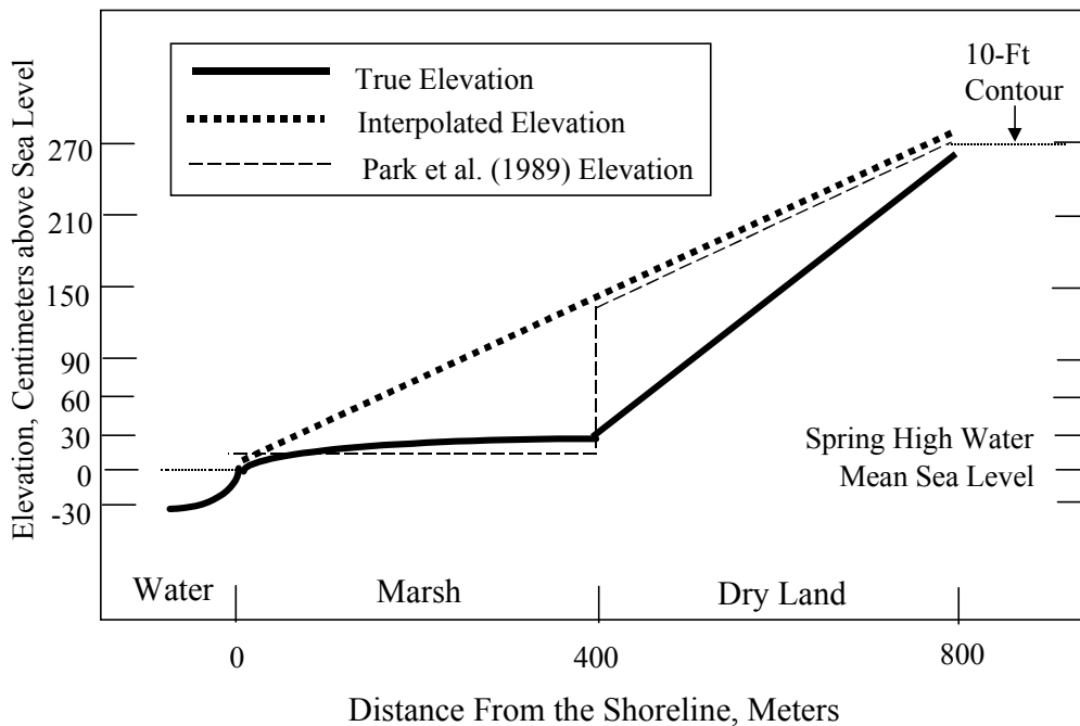
Figure 1. Potential Errors from Interpolating Elevations in Coastal Areas.
