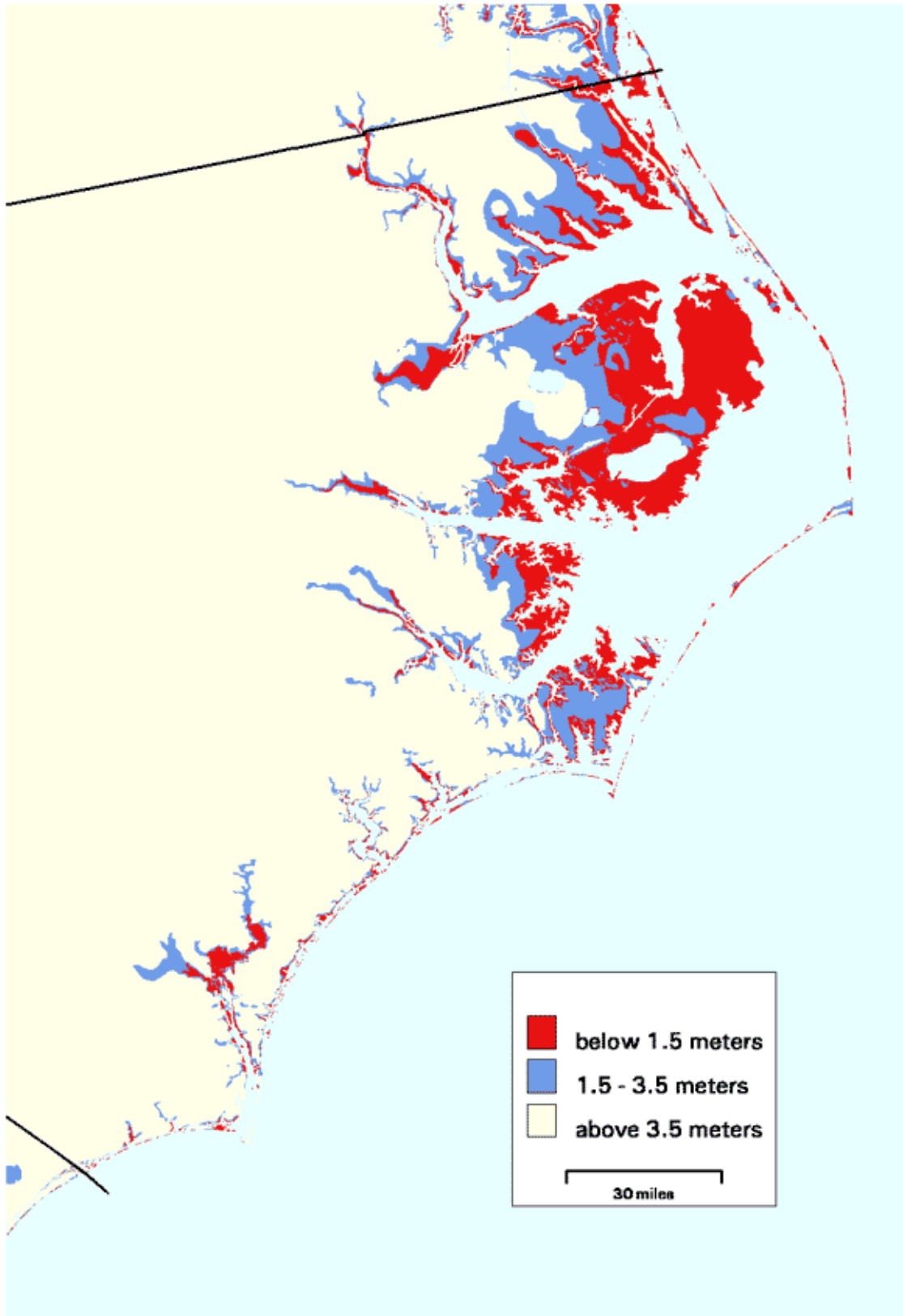
Figure 5. Lands Close to Sea Level: North Carolina
