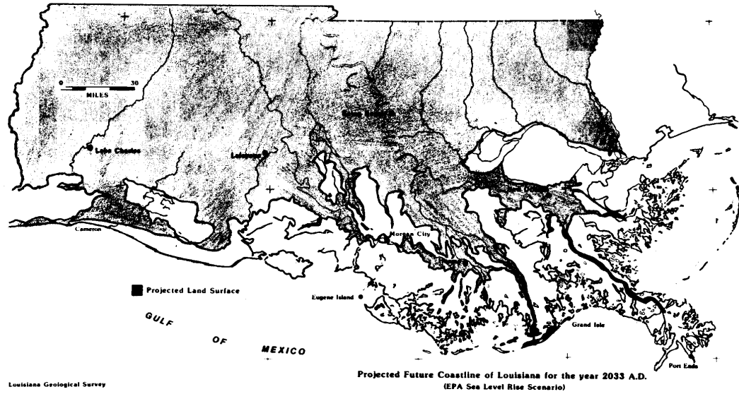
FIGURE 1-12 PROJECTED FUTURE COASTLINE OF LOUISIANA FOR THE YEAR 2033 GIVEN A RISE IN SEA LEVEL OF 54.9 CM
