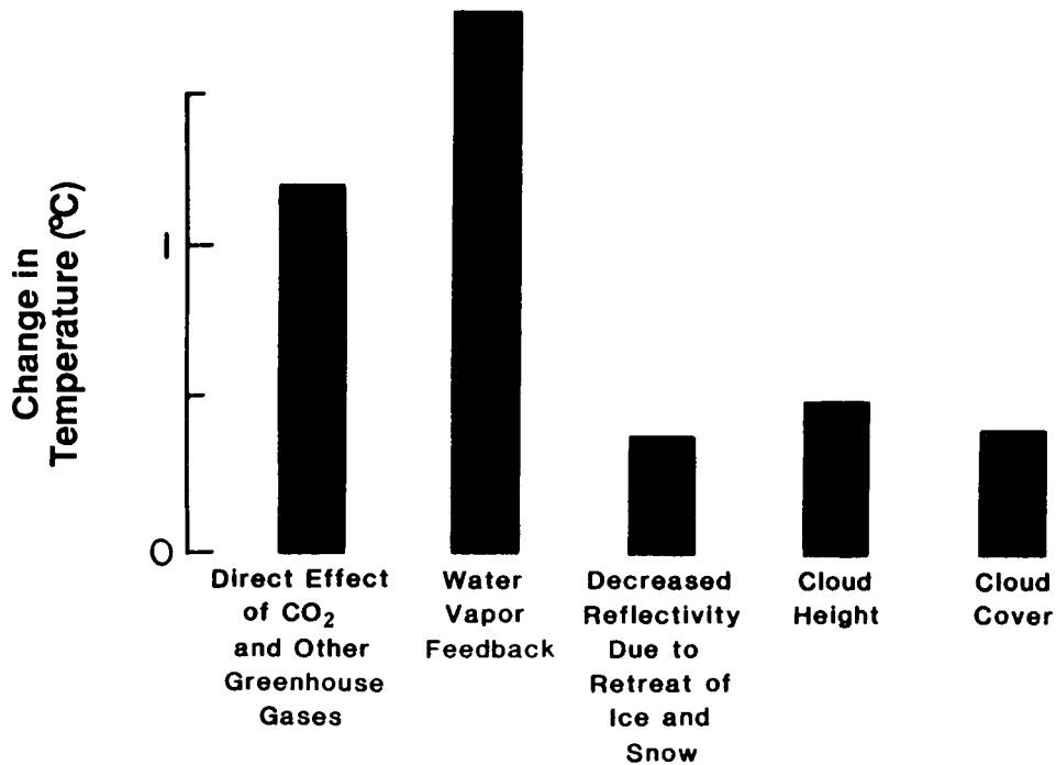
FIGURE 1-3 ESTIMATED GLOBAL WARMING DUE TO A DOUBLING OF GREENHOUSE GASES: DIRECT EFFECTS AND CLIMATIC FEEDBACKS
