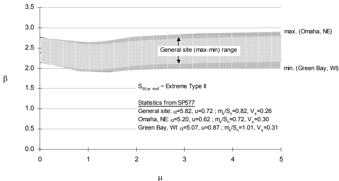
Figure 2.3 Effect of Considering Site-Specific Snow Load Statistics on Reliability of Flexural Members (D+S), LRFD, \Delta t = 14 days
