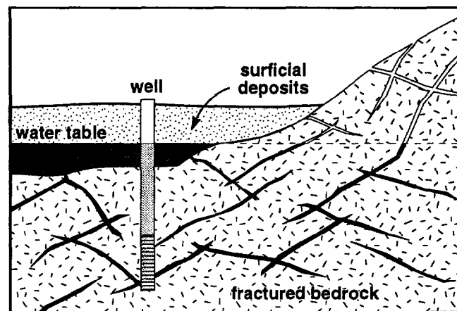
Figure 2-3. A fractured rock aquifer.
