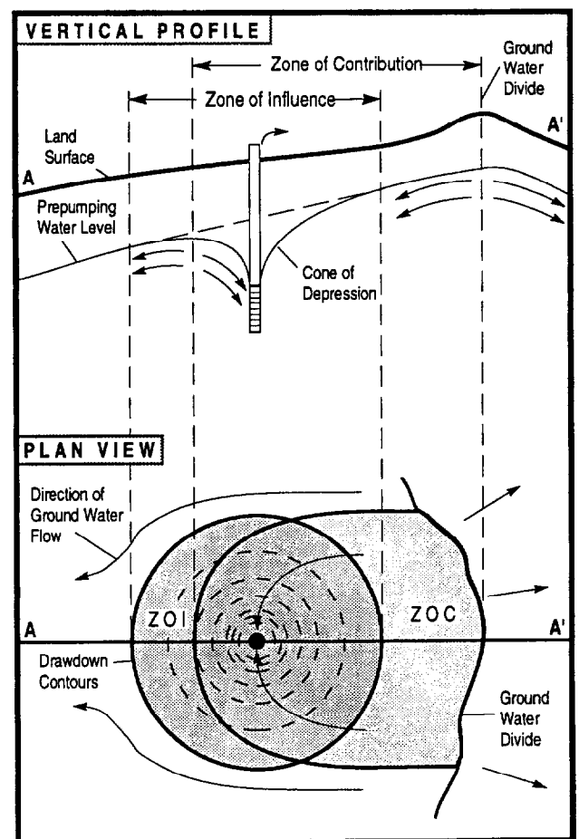
Figure 2-4. The zone of contribution, zone of influence, and cone of depression. Prepared by Horsley and Witten, Inc.
