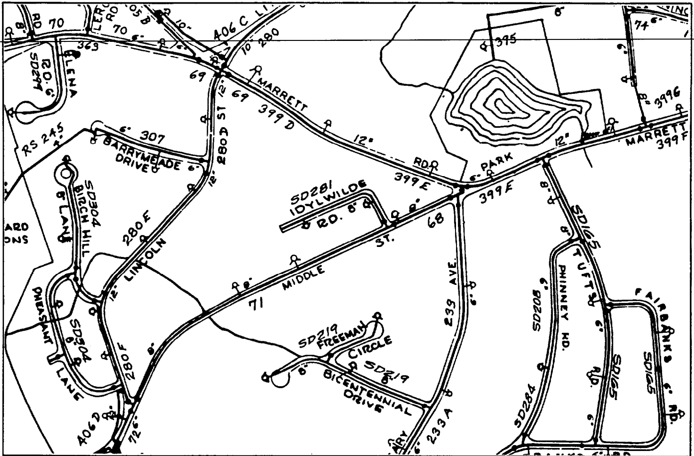
Figure 4-8. Utility map depicting existing drainage piping network.
