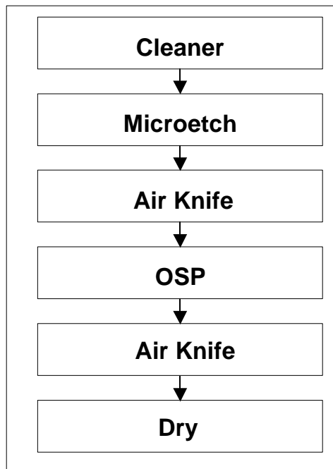
Figure 3: OSP Process Flow
