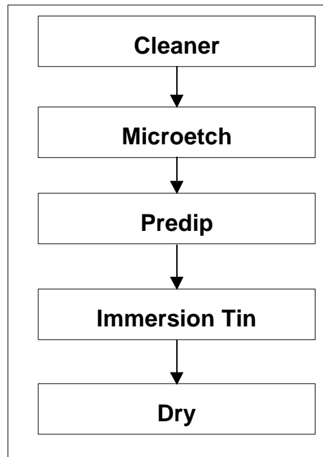
Figure 2: Immersion Tin Process Flow
