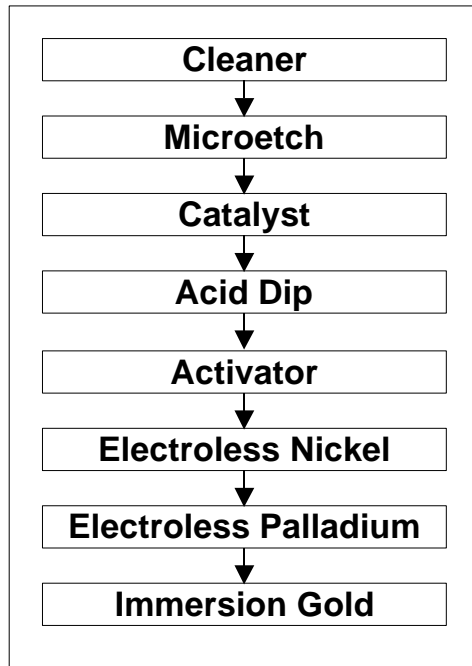
Figure 5: Electroless Nickel/Electroless Palladium/Immersion Gold Process Flow
