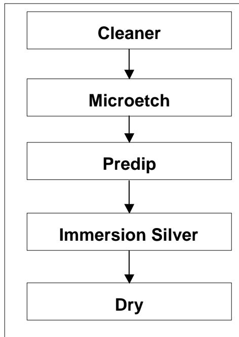
Figure 1: Immersion Silver Process Flow
