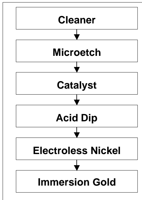
Figure 4: Electroless Nickel/Immersion Gold Process Flow
