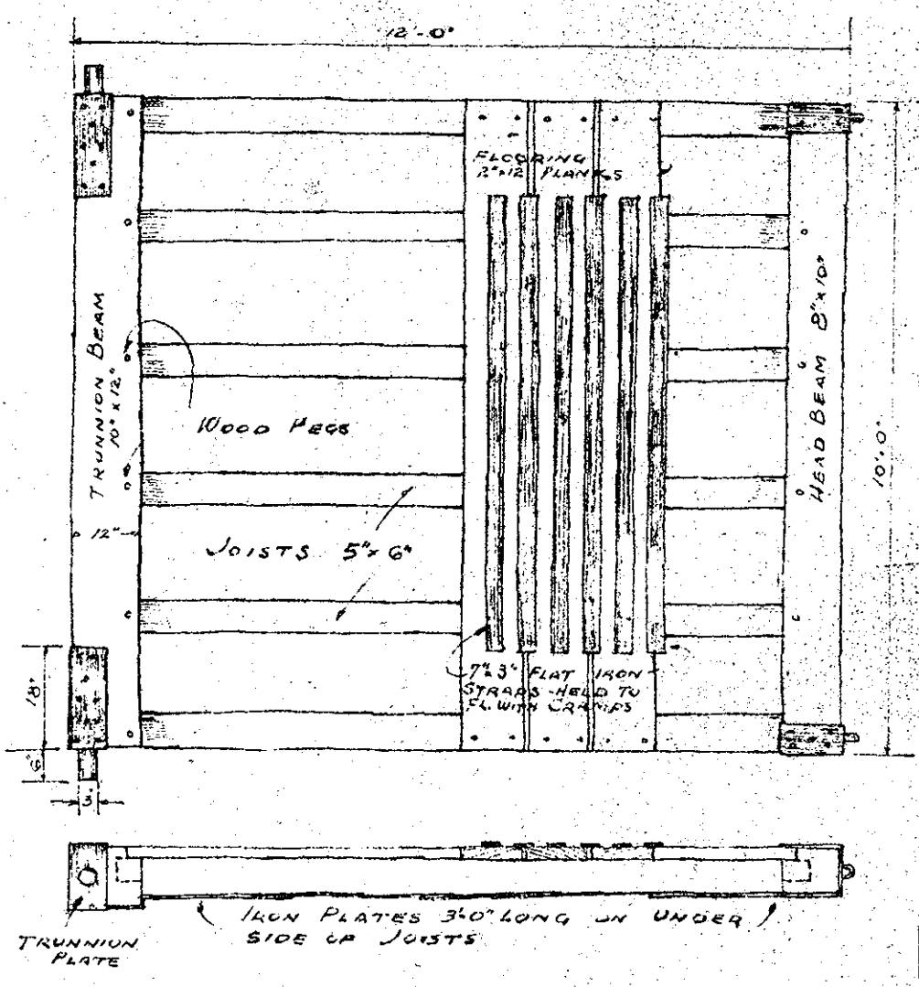
EXHIBIT D: Drawbridge Table based on Muller's description - 1756. Scale: 1/2" = 1'-0"
