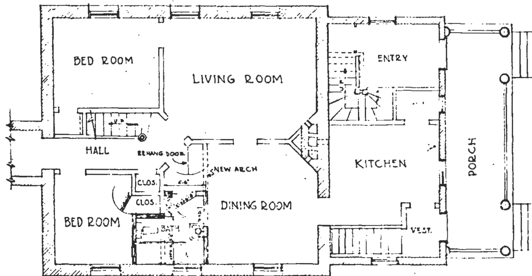
FIRST FLOOR APARTMENT SCALE 3/4" = 1'-0"
