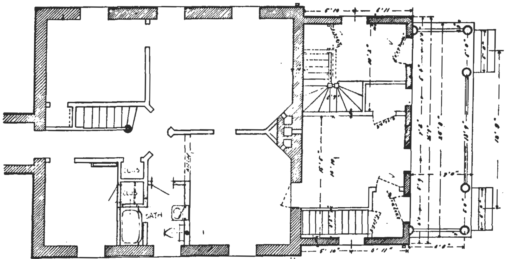
Plan of 1 st Story
