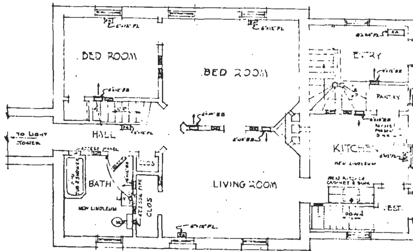
FIRST FLOOR APARTMENT SCALE 1/4" = 1'-0"
