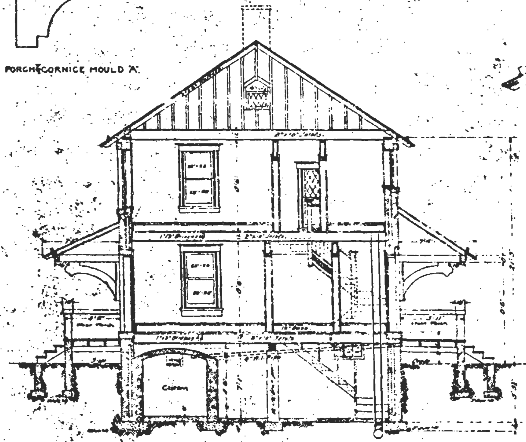
TRANSVERSE SECTION
