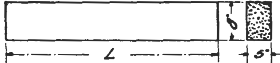
Window Sill 7 Req'd - L = 3'8" 1 .. L = 3'4"
