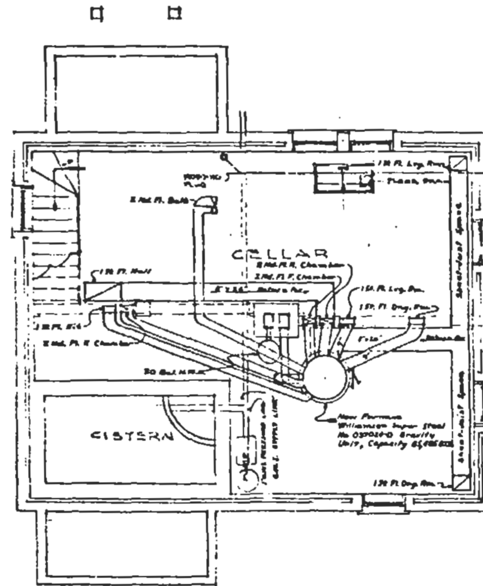
BASEMENT PLAN SCALE: 1/8"=1'-0"
