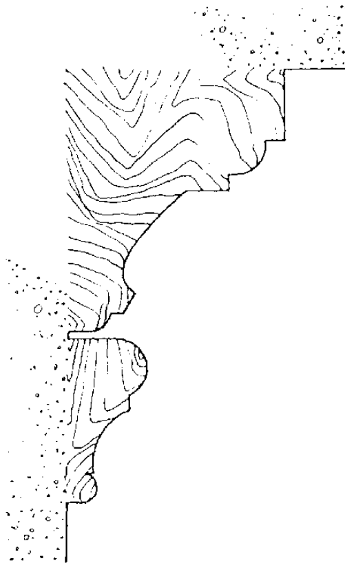
Ⓒ COVE MOLD
