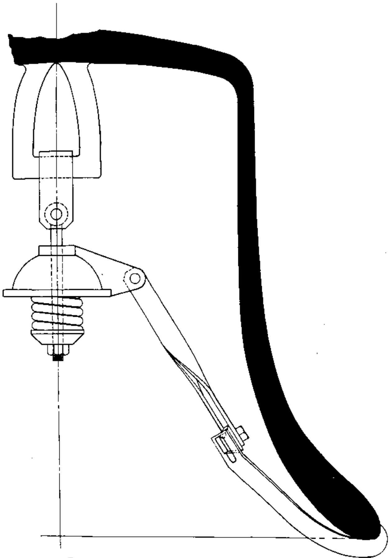
SECTION OF BELL SHOWING ARRANGEMENT OF SPIDER.
