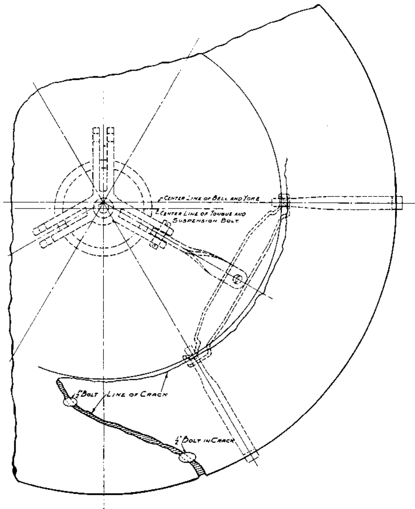
• PART PLAN OF BELL SHOWING SPIDER •
