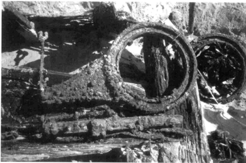
Figure 4.97. Comet 's port windlass purchase arm and windlass hardware on the main deck laying against the port side of the pawl post and bowsprit. NPS photo by Don Morris.
