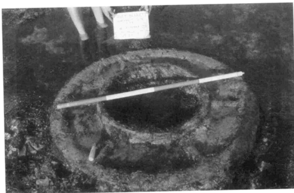
Figure 4.19. Iron ring from a windlass messenger chain system (feature PB-017). NPS photo by Adriane Neidinger.
