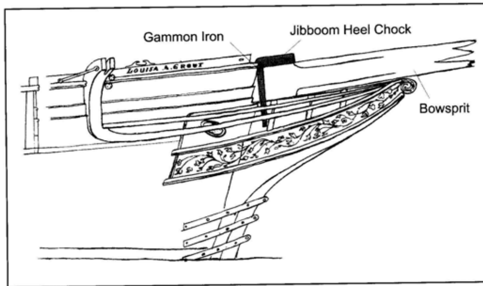
Figure 4.87. Vessel bow section showing location of the gammon iron and jibboom heel chock (after Chapelle 1973:359).
