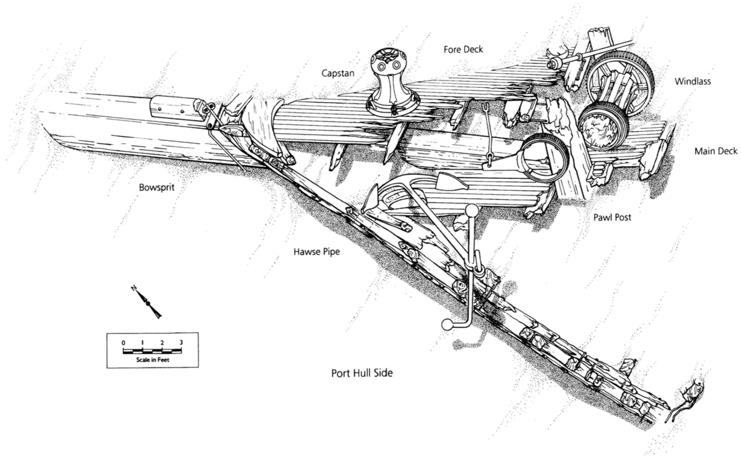
Figure 4.70. Comet site plan. Field drawing by Matt Russell; final drawing by Robert Turner.
