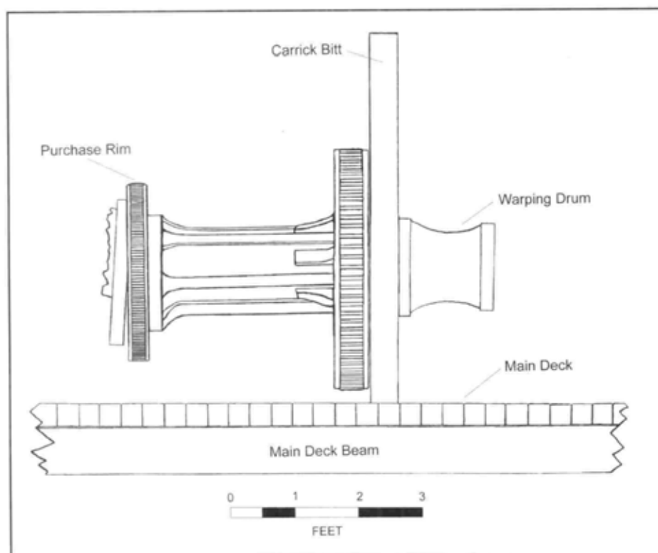
Figure 4.95. Comet's windlass, elevation view looking forward on main deck. Drawing by Jim Bradford and Matt Russell.
