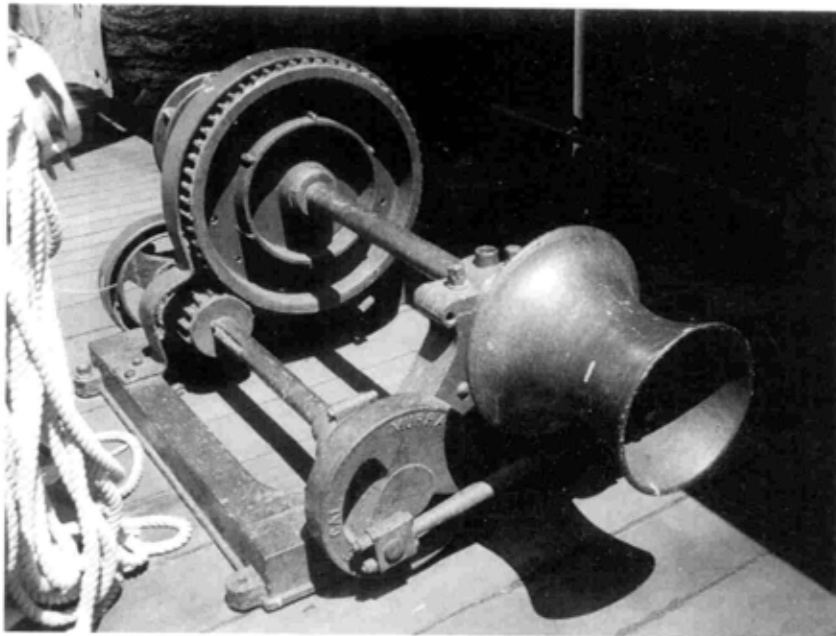
Figure 4.17. Windlass from Falls of Clyde in Honolulu, Hawaii. The smaller mechanism to the left is similar to features PB-021 and PB-022. NPS photo by Matt Russell.
