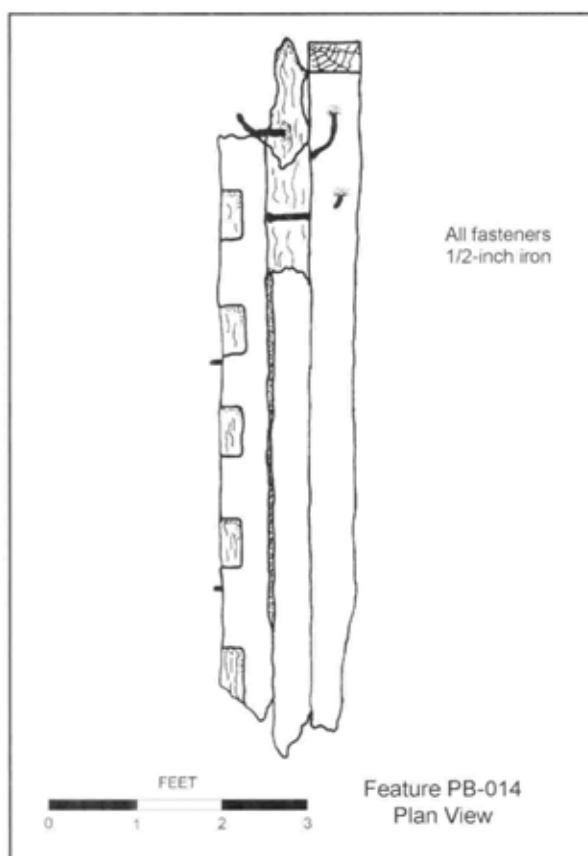
Figure 4.43. Plan view of feature PB-014, likely part of the same coaming as feature PB-011. Drawing by Matt Russell.
