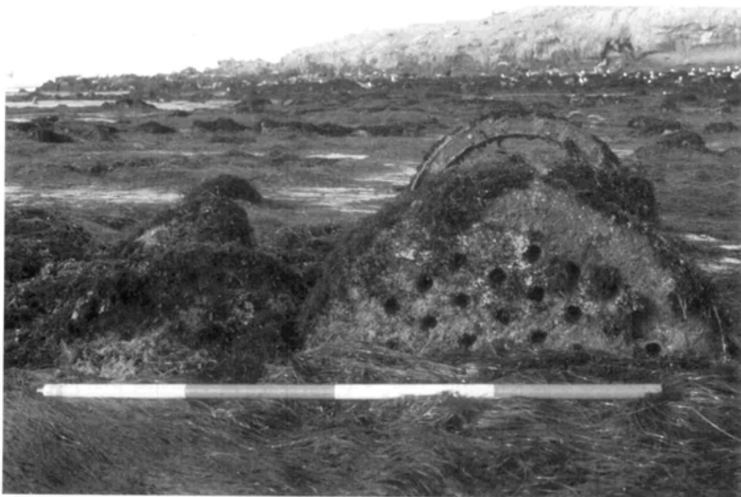
Figure 4.12. End view of the donkey boiler. NPS photo by Adriane Neidinger.
