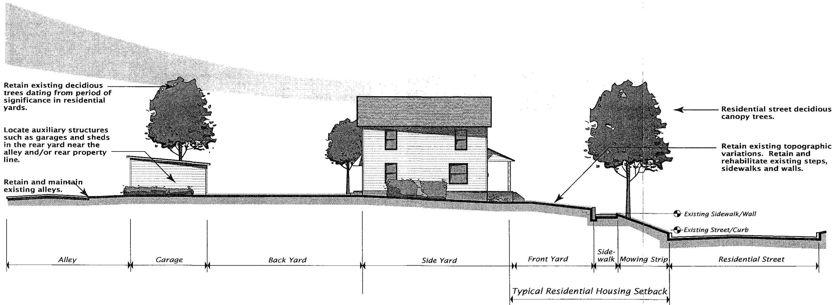
EXHIBIT 29 TYPICAL HOUSE/STREET SETBACK SECTION VIEW NOT TO SCALE
