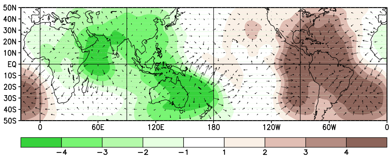
FIGURE T24. Mean (top) and anomalous (bottom) 200-hPa velocity potential ( 10^6\text{m}^2\text{s} ) and divergent wind (CDAS/Reanalysis). Anomalies are departures from the 1979-1995 base period monthly means.
