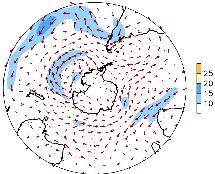
FIGURE E16. Southern Hemisphere mean (left) and anomalous (right) 300-hPa vector wind (CDAS/Reanalysis) for SEP 2007. Mean (anomaly) isotach contour interval is 10 (5) ms -1 . Values greater than 30 ms -1 (left) and 10 ms -1 (right) are shaded. Anomalies are departures from the 1979-95 base period monthly means.
