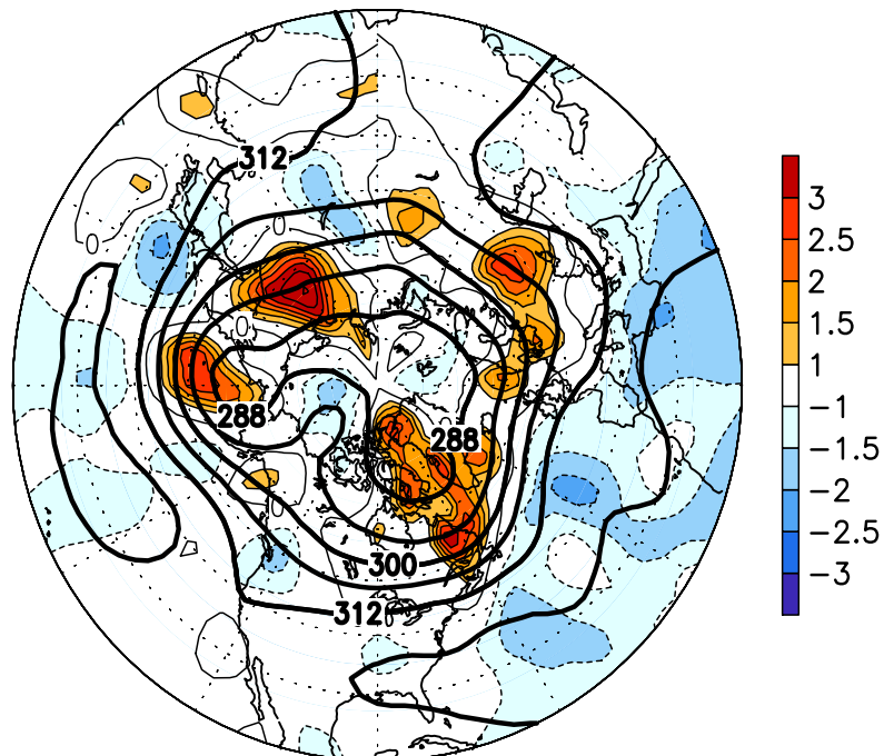
FIGURE E13. Northern Hemisphere: 700-hPa heights for SEP 2007 overlaid with standard deviation of high-pass filtered height (left) and normalized anomalous variance of high-pass filtered height (right). Heights are indicated by thick solid contours in both panels (interval is 60 m). High-pass filtered fields reflect fluctuations having periods less than 10 days, and are indicated by thin contours and shading. Contour interval for standard deviation is 15 m with values > 45 m shaded. Contour interval for normalized variance is 1 standard deviation, with positive values shown by solid contours and dark shading and negative values shown by dashed contours and light shading. Anomalies are departures from the 1964-93 base period monthly means.
