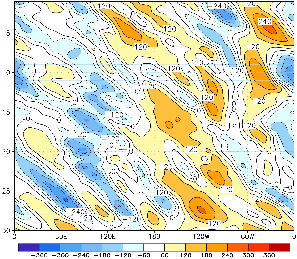
FIGURE E18. Southern Hemisphere: Daily 500-hPa height anomalies for SEP 2007 averaged over the 5° latitude band centered on 40°S. Positive values are indicated by solid contours and dark shading. Negative values are indicated by dashed contours and light shading. Contour interval is 60 m. Anomalies are departures from the 1979-95 base period daily means.
