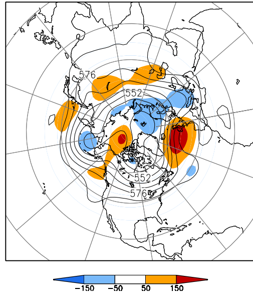
500-hPa Height (dm) & Anomalies (m) (Sep 1–15, 2007)
