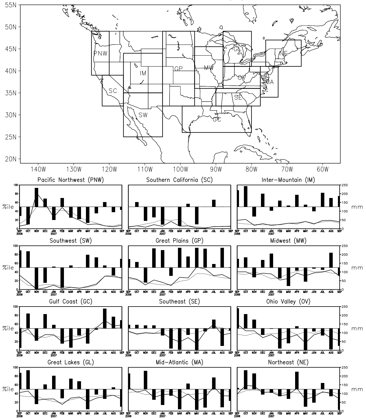
FIGURE E5. Areal estimates of monthly mean precipitation amounts (mm, solid lines) and precipitation percentiles (% bars) for the most recent 13 months obtained from a merge of raingauge observations and satellite-derived precipitation estimates (Janowiak and Xie 1999, J. Climate , 12 , 3335–3342). The monthly precipitation climatology (mm, dashed lines) is from the 1979–2000 base period monthly means. Monthly percentiles are not shown if the monthly mean is less than 5 mm.
