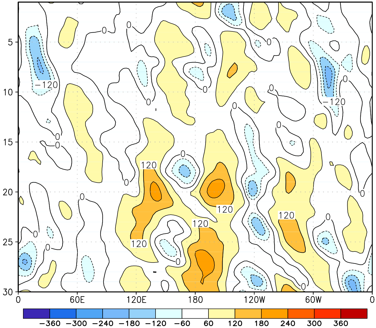
FIGURE E12. Northern Hemisphere: Daily 500-hPa height anomalies for SEP 2007 averaged over the 5° latitude band centered on 40°N. Positive values are indicated by solid contours and dark shading. Negative values are indicated by dashed contours and light shading. Contour interval is 60 m. Anomalies are departures from the 1979-95 base period daily means.
