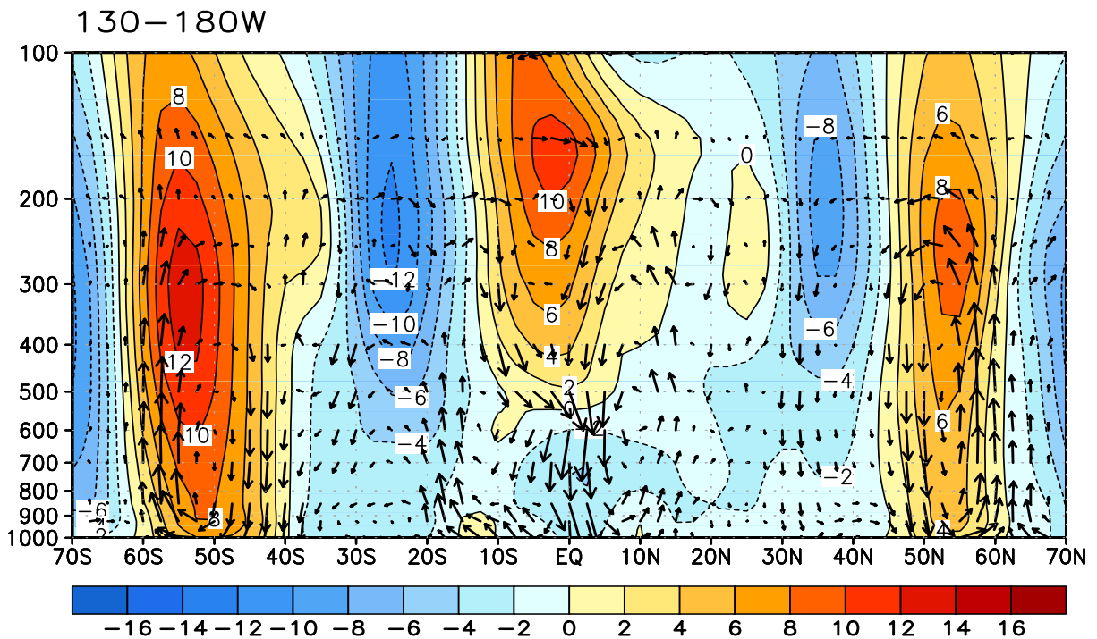
FIGURE T32. Pressure-latitude section of the mean (top) and anomalous (bottom) zonal wind ( \text{m s}^{-1} ) and divergent circulation averaged over the central Pacific sector (130W-180W). The divergent circulation is represented by vectors of combined pressure vertical velocity and the divergent component of the meridional wind. Red shading and solid contours denote a westerly (top) or anomalous westerly (bottom) zonal wind. Blue shading and dashed contours denote an easterly (top) or anomalous easterly (bottom) zonal wind. Anomalies are departures from the 1979-1995 base period monthly means.
