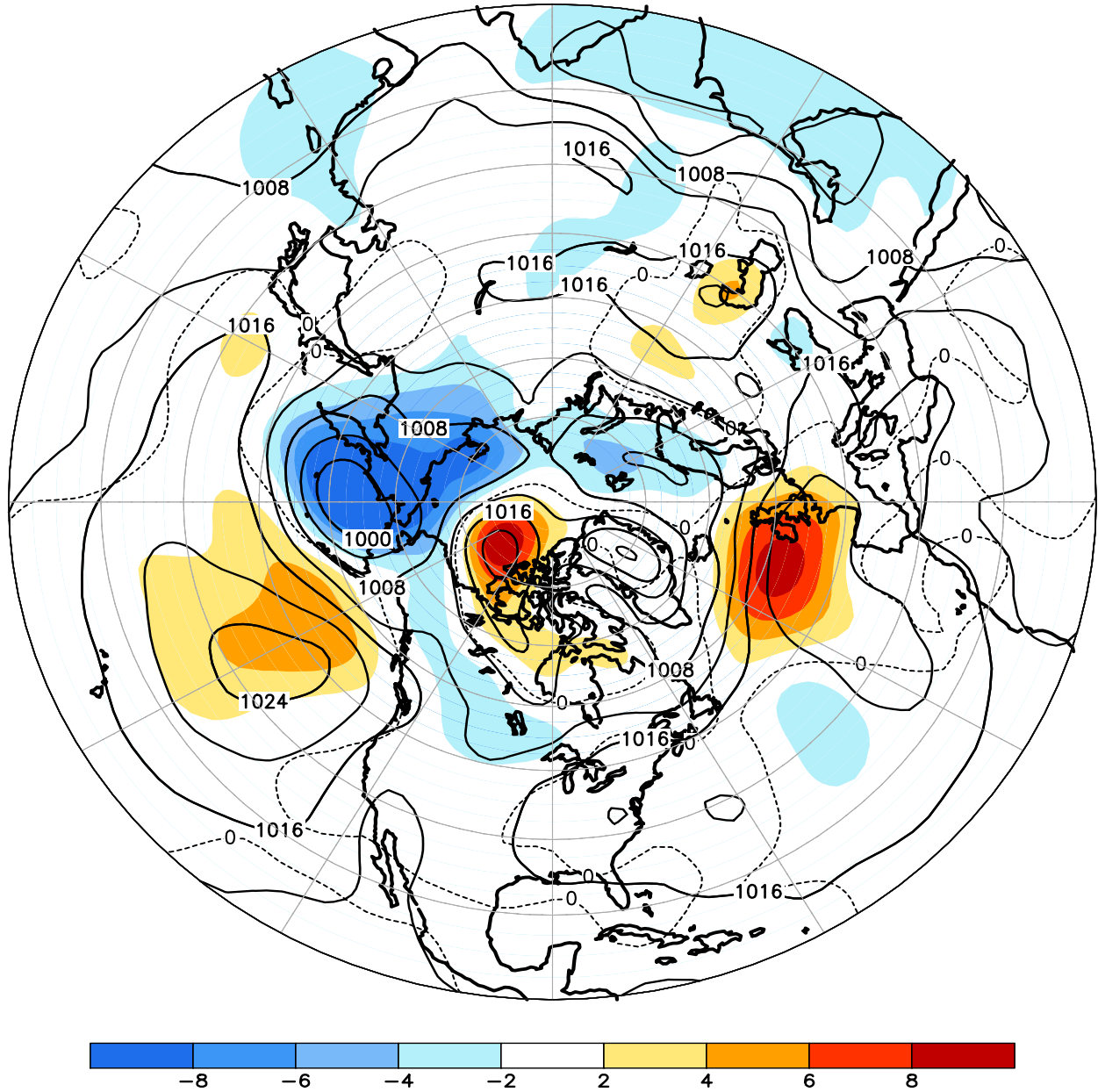
FIGURE E8. Northern Hemisphere mean and anomalous sea level pressure (CDAS/Reanalysis) for SEP 2007. Mean values are denoted by solid contours drawn at an interval of 4 hPa. Anomaly contour interval is 2 hPa with values less (greater) than -2 hPa (2 hPa) indicated by dark (light) shading. Anomalies are calculated as departures from the 1979-95 base period monthly means.
