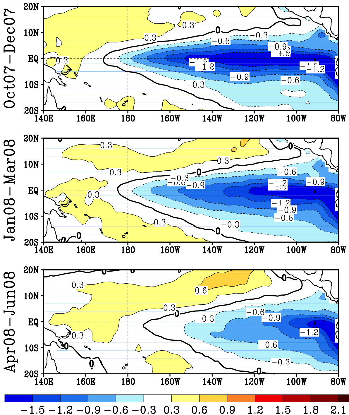
FIGURE F5. Predicted 3-month average sea surface temperature anomalies from the NCEP/CPC Markov model (Xue et al. 2000, J. Climate , 13 , 849-871). The forecast is initiated in SEP 2007. Contour interval is 0.3C and negative anomalies are indicated by dashed contours. Anomalies are calculated relative to the 1971-2000 climatology.
