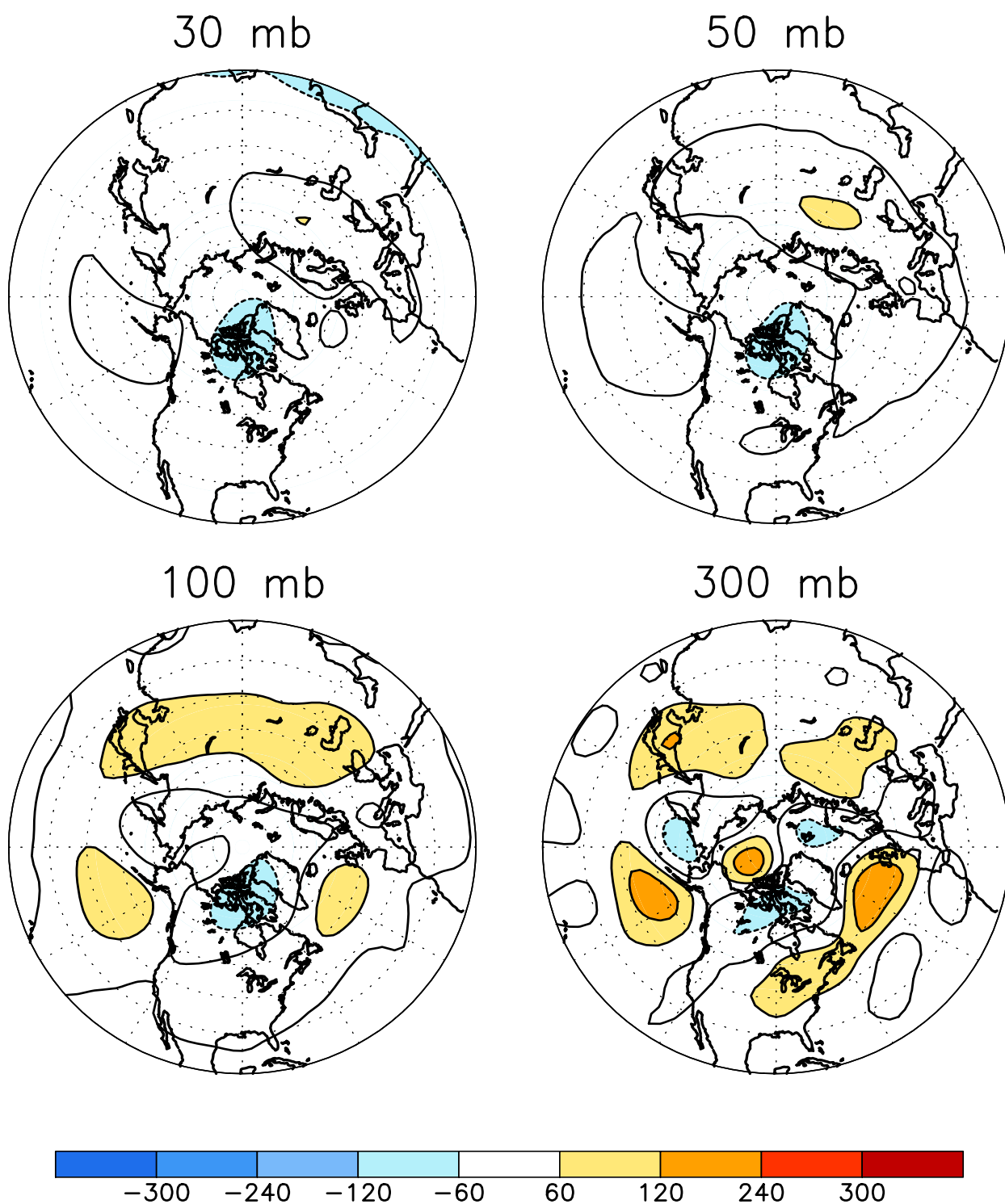
FIGURE S1. Stratospheric height anomalies (m) at selected levels for SEP 2007. Positive values are indicated by solid contours and dark shading. Negative values are indicated by dashed contours and light shading. Contour interval is 60 m. Anomalies are calculated from the 1979–95 base period means. Winter Hemisphere is shown.
