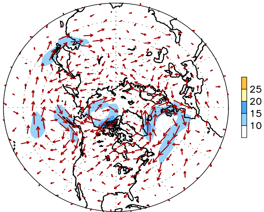
FIGURE E10. Northern Hemisphere mean (left) and anomalous (right) 300-hPa vector wind (CDAS/Reanalysis) for SEP 2007. Mean (anomaly) isotach contour interval is 10 (5) \text{ms}^{-1} . Values greater than 30 \text{ms}^{-1} (left) and 10 \text{ms}^{-1} (rights) are shaded. Anomalies are departures from the 1979-95 base period monthly means.
