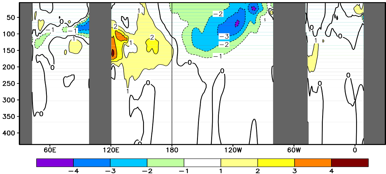
FIGURE T17. Equatorial depth-longitude section of ocean temperature (top) and ocean temperature anomalies (bottom) for SEP 2007. Contour interval is 1°C. Dashed contours in bottom panel indicate negative anomalies. Data are derived from the NCEP's global ocean data assimilation system version 2 which assimilates oceanic observations into an oceanic GCM (Xue, Y. and Behringer, D.W., 2006: Operational global ocean data assimilation system at NCEP, to be submitted to BAMS). Anomalies are departures from the 1982–2004 base period means.
