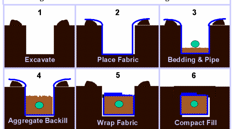
Figure 7-3: Subdrain construction with geotextiles
