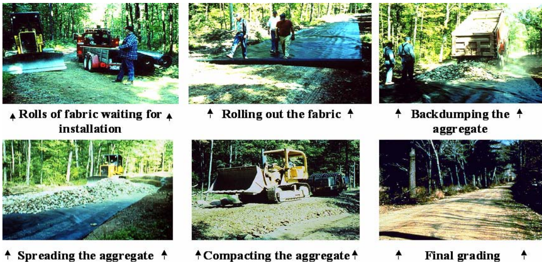
7-29 Installation of a Separation Fabric.
