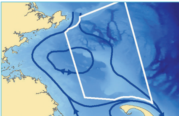
This image depicts the general oceanographic current regime (in blue) around Stellwagen Bank (boundary in white). Source: adapted from P. Lermusiaux, Harvard University
