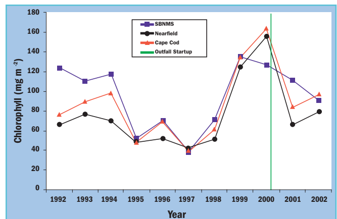
Nutrient and chlorophyll levels appear to decline or remain stable in the first two years after the MWRA Boston Harbor outfall was activated in September 2000.
