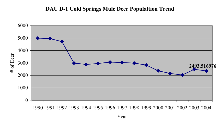
Figure 3-11. Mule Deer Population Trends In Primary Planning Area DAUs
