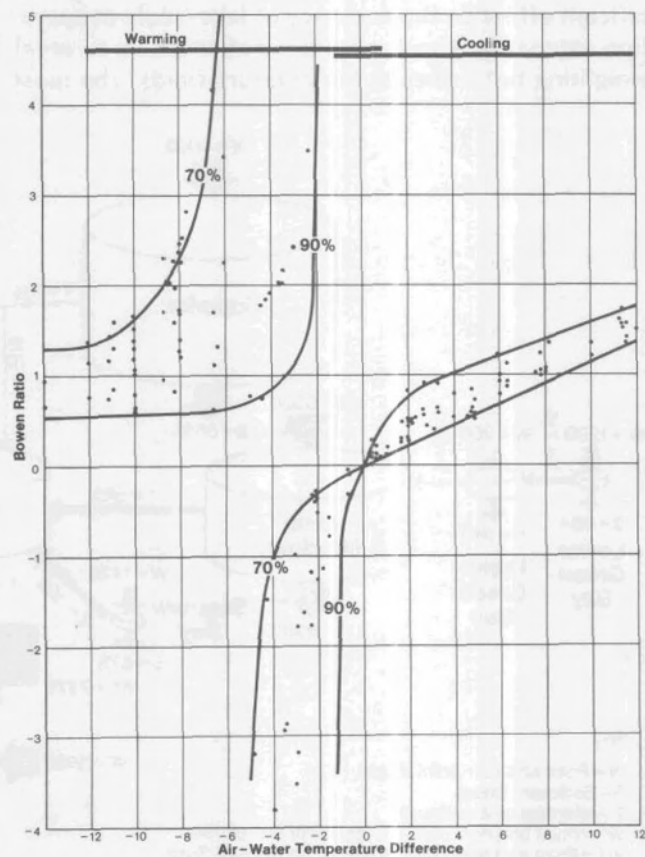
The Bowen ratio as a function of air-water temperature differences at 70 and 90 percent relative humidities. Calculation of the Bowen ratio, the ratio of sensible to latent heat, is necessary to evaporation estimates.
