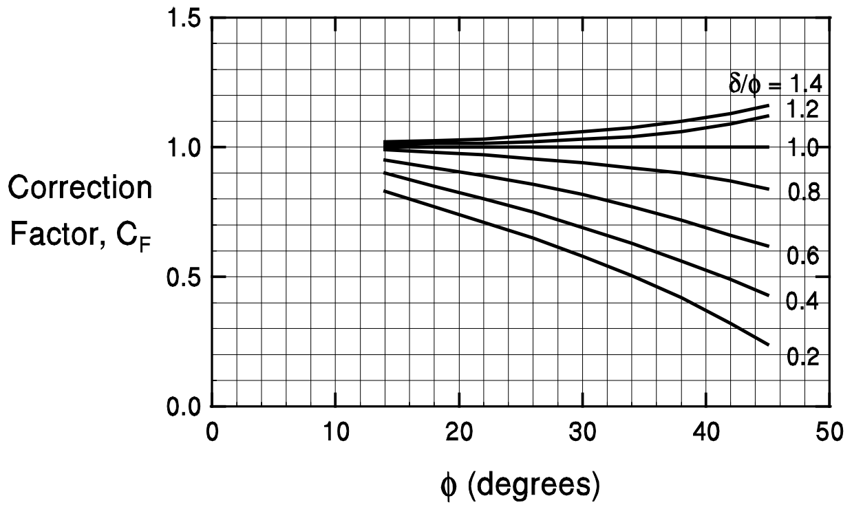
Figure 7-9. Correction factor for K_\delta when \delta \neq \phi (after Norlund 1979).
