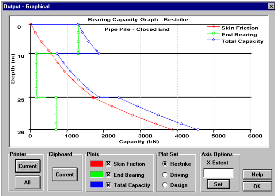
Figure 4-2. Graphical output screen.
