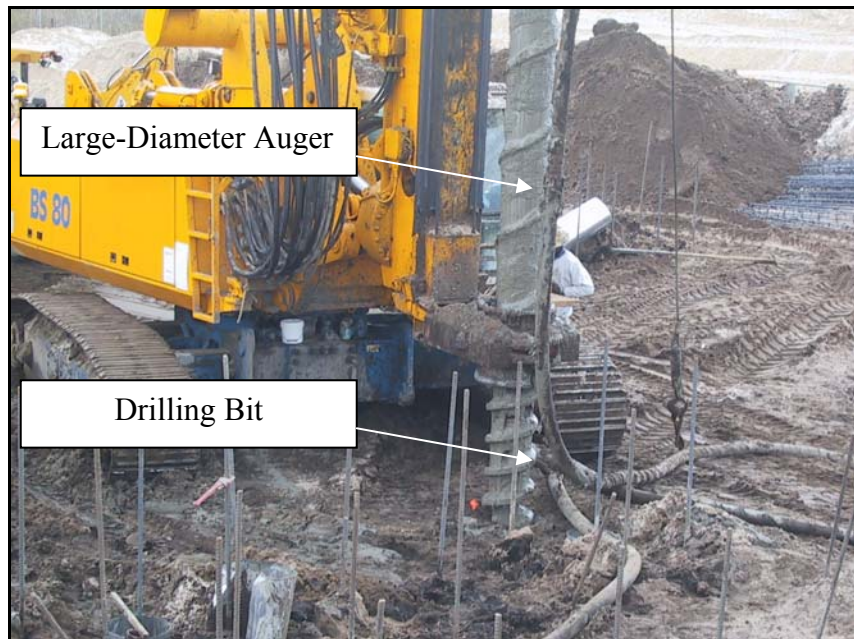
Figure 2.6: Displacement Pile
