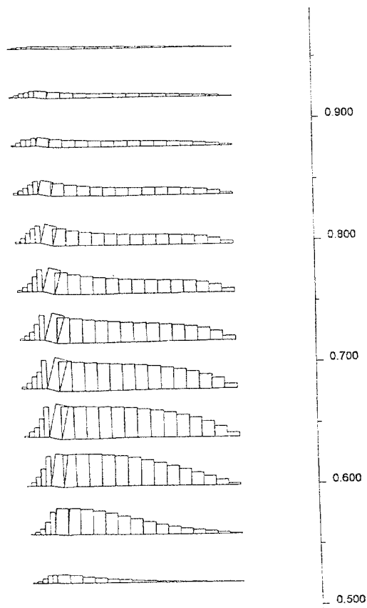
Figure 4.25 Axial Force Distribution in Reinforcement for Case 8-1 ( s=0.4 m, l=1.5 m): (a) Failure State ( h=8.0 m, l/h=0.19 ); (b) Critical State ( h=5.0 m, l/h=0.30 ), Continued.
