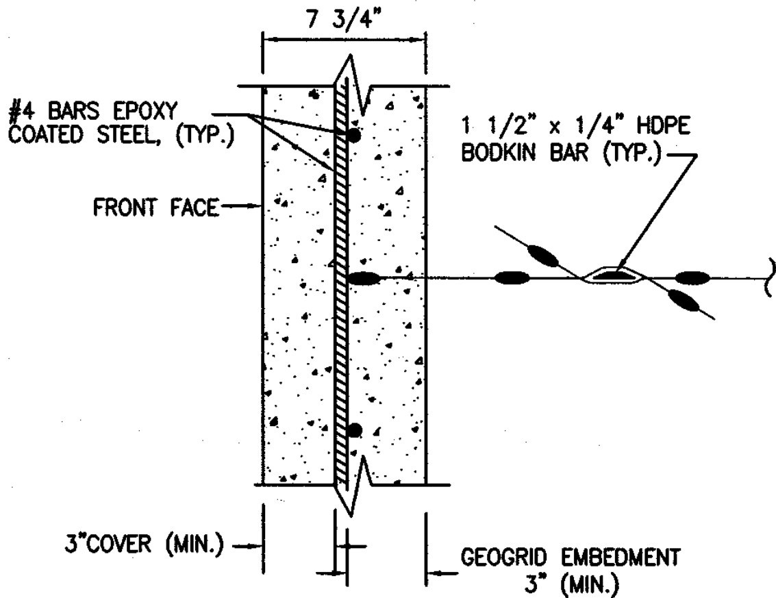
Figure 34. Bodkin connection detail.
