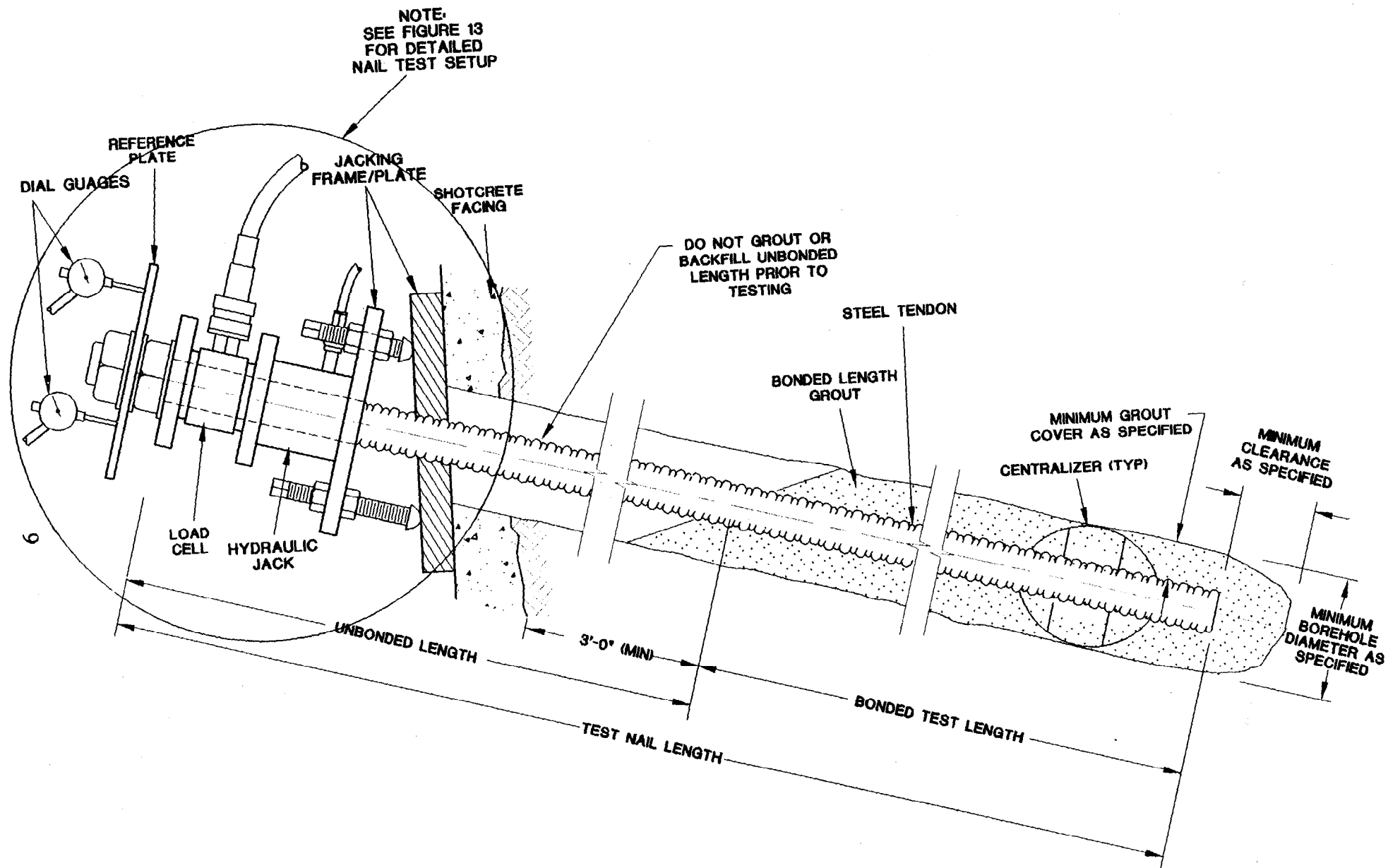
Figure 6. Typical Test Nail Detail.
