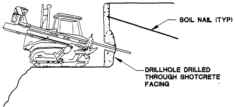
NAIL DRILLING THROUGH THE FULL SHOTCRETE FACING
