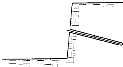
STEP 3. INSTALL AND GROUT NAIL
