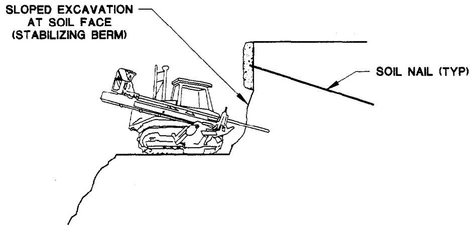
NAIL DRILLING THRU A PROTECTIVE STABILIZING BERM
