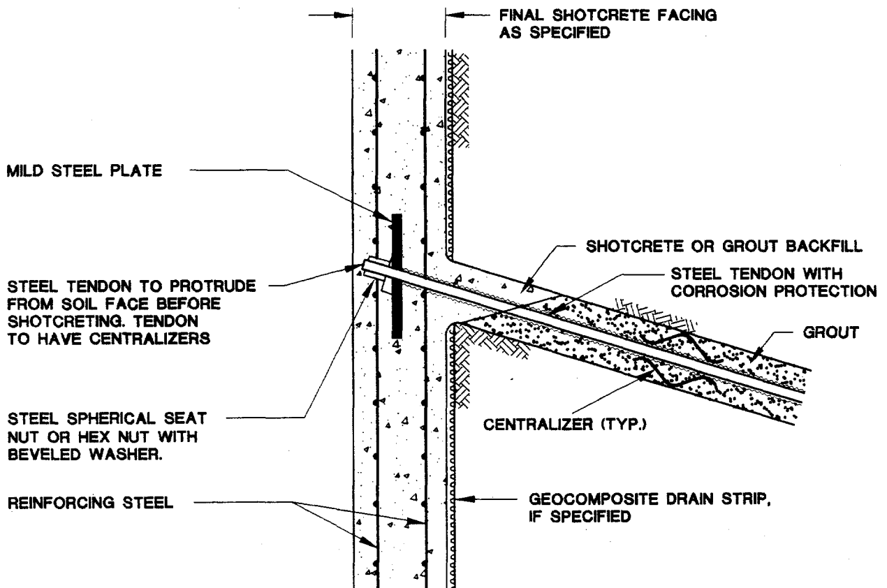
Figure 7B. Typical Permanent Shotcrete Facing Detail.
