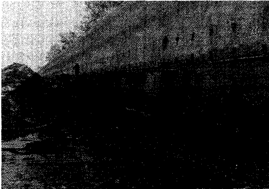
P46. Mass excavation stopped short of final wall line to leave a stabilizing (buffer) berm.
