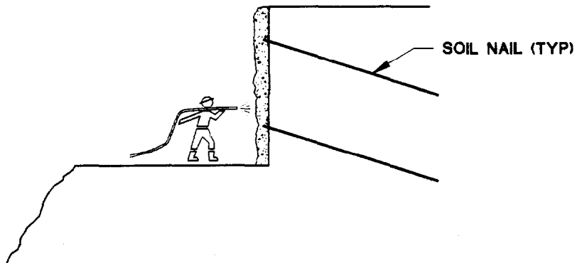
SHOTCRETING AFTER EXCAVATION OF STABILIZING BERM
