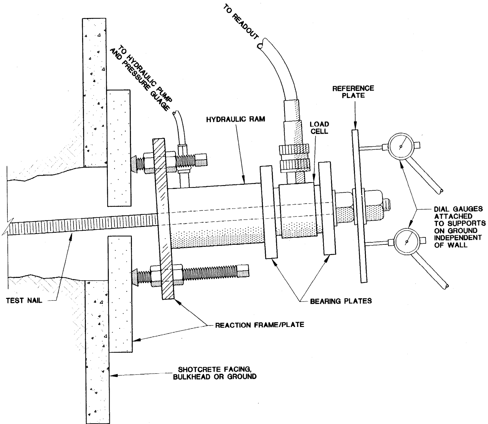
Figure 13. Typical Nail Test Setup.
