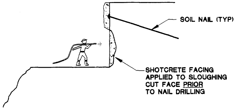
SHOTCRETE FLASHCOAT PRIOR TO DRILLING
