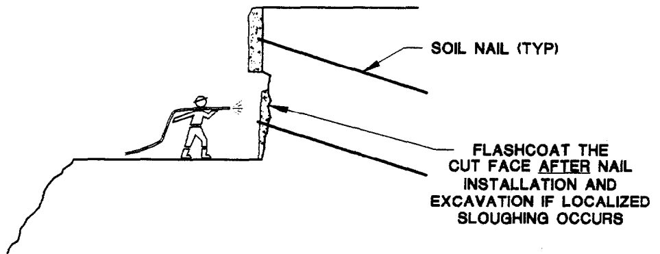
FLASHCOAT SHOTCRETING
