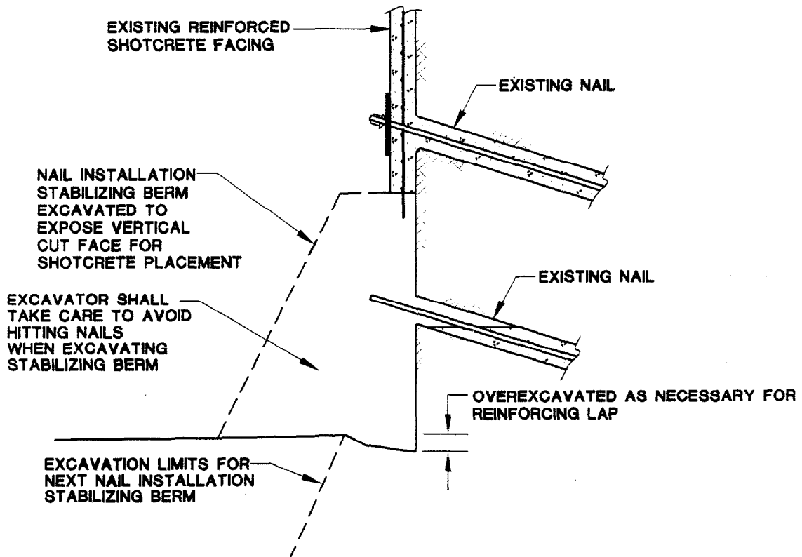
DETAIL 2 EXCAVATION OF STABILIZING BERM FOR SHOTCRETE PLACEMENT
