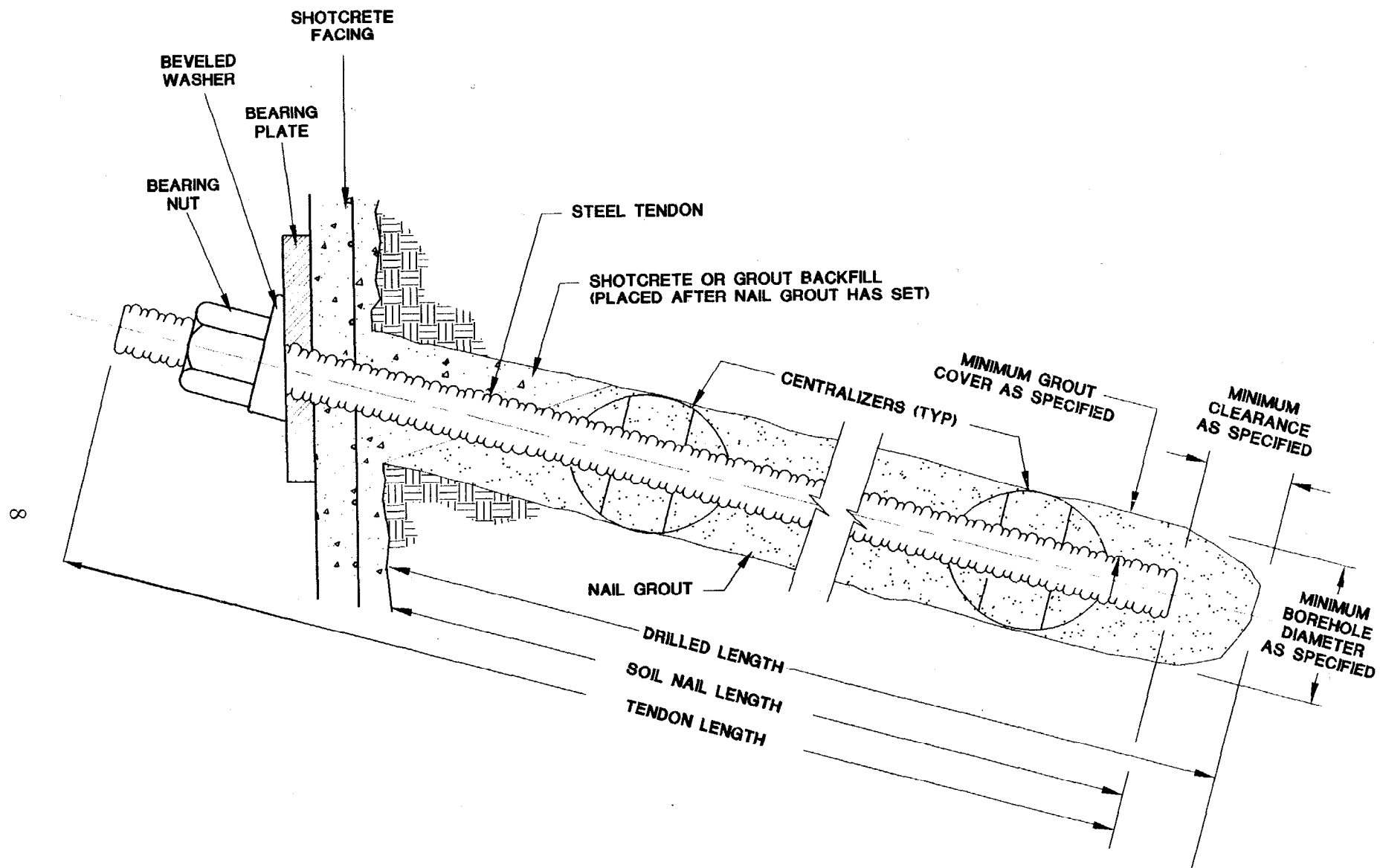
Figure 5. Typical Production Nail Detail.
