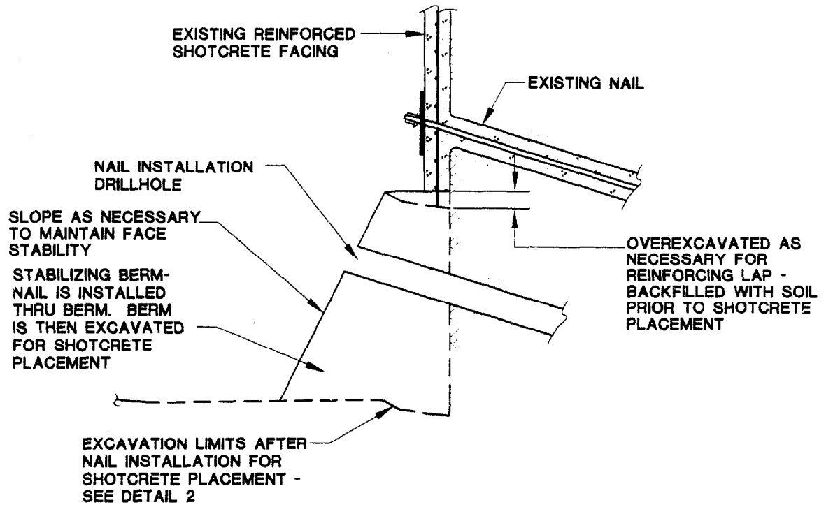
DETAIL 1 NAIL INSTALLATION THRU STABILIZING BERM
