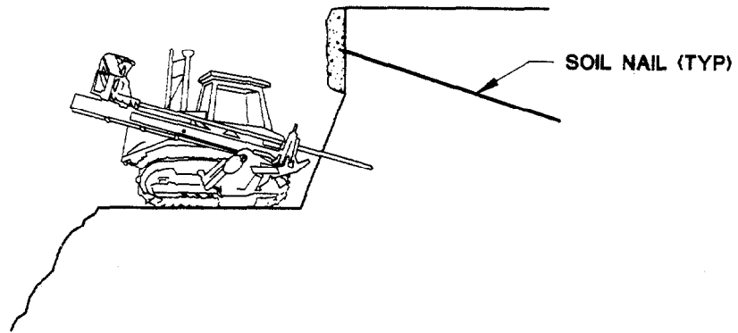
NAIL DRILLING
