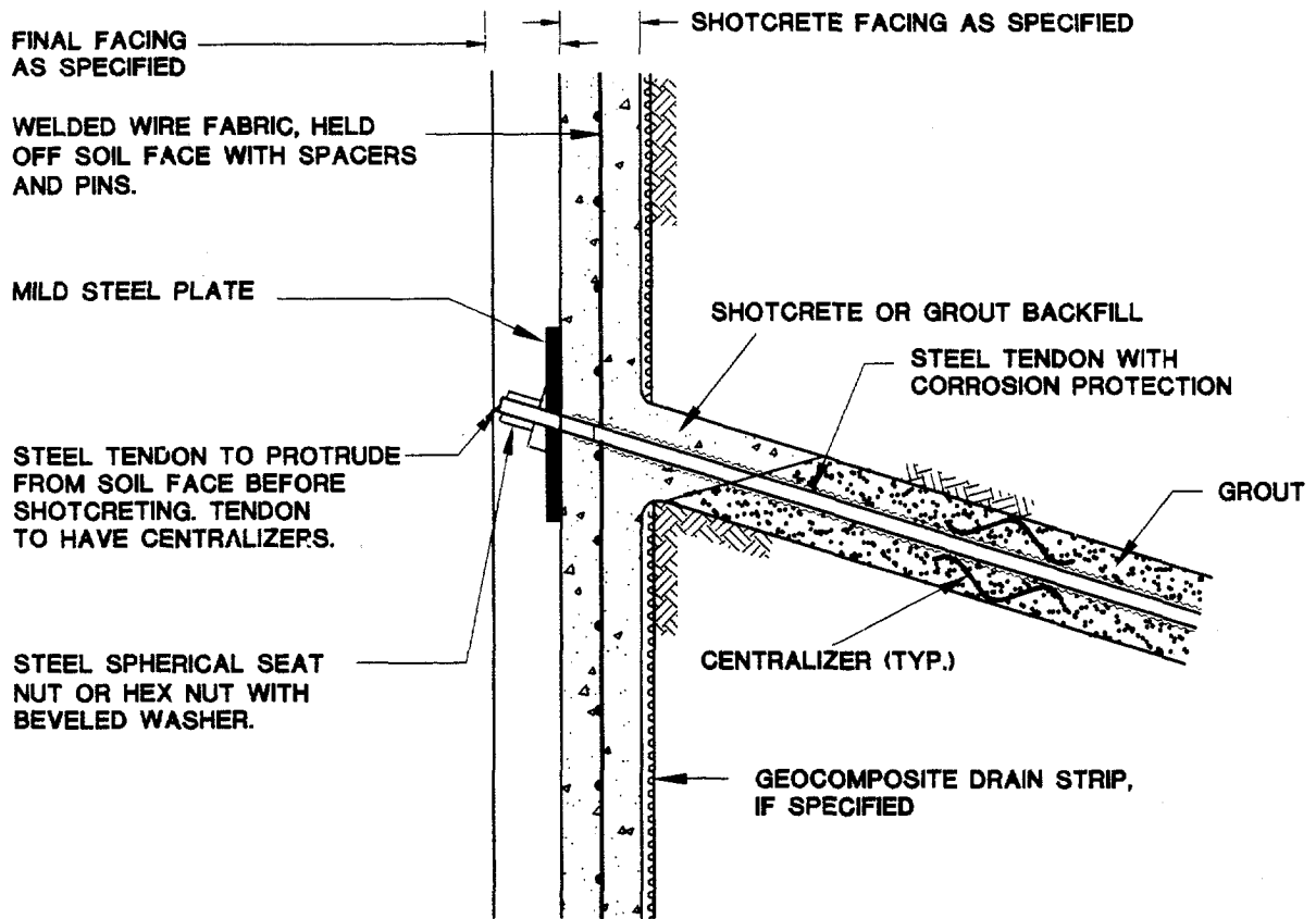
Figure 7A. Typical Temporary Shotcrete Facing Detail.
